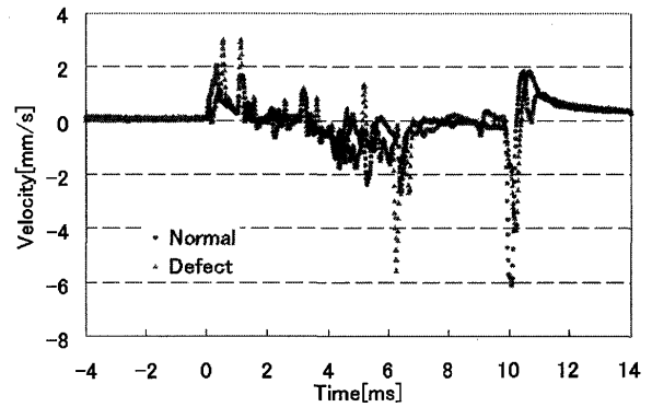
Fig. 5 Monitoring results of vertical vibration velocity of specimen during laser welding.
