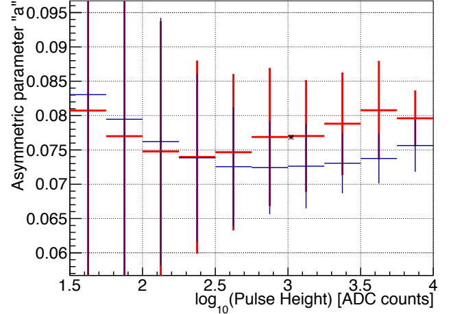
Figure 6.10: The distribution of asymmetric parameter “a” as a function of pulse-height for the crystal of CsI ID=695 ( x[\text{mm}] , y[\text{mm}])=(-12.5, -237.5) with energy of 119.9 MeV. Red and blue points represent neutron-rich sample and photon-rich sample, respectively. The error bars represent the standard deviation of the parameter. The * represents the obtained value in the remaining event in the physics data.
