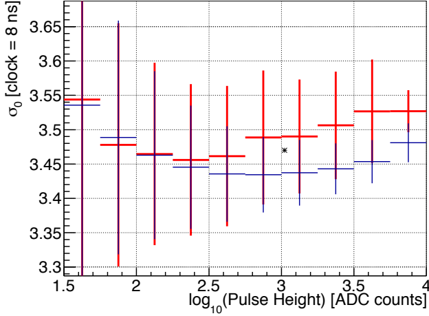
Figure 6.9: The distribution of \sigma_0 as a function of pulse-height for the crystal of CsI ID=695 ( x[\text{mm}] , y[\text{mm}])=(-12.5, -237.5) with energy of 119.9 MeV. Red and blue points represent neutron-rich sample and photon-rich sample, respectively. The error bars represent the standard deviation of the parameter. The * represents the obtained value in the remaining event in the physics data.
