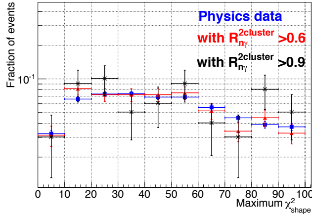
Figure 6.26: Maximum \chi^2_{pulse\ shape} distribution in the physics data with the loose cuts. Blue, red and black histograms represent the physics data without cut on R_{n\gamma}^{2cluster} , with R_{n\gamma}^{2cluster} > 0.6 , and with R_{n\gamma}^{2cluster} > 0.9 , respectively.
