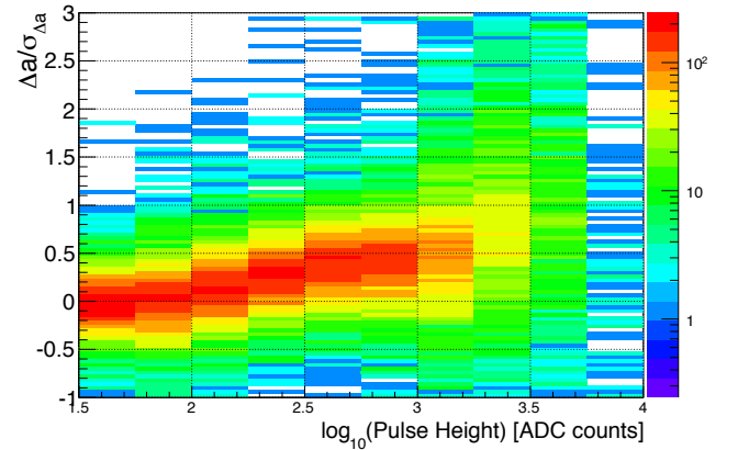
Figure 5.15: The significance of the difference of the asymmetric parameter “ a ” between photon-rich sample and neutron-rich sample after requiring \chi^2_{shape} < 4.6 vs. pulse-height distribution for all channels of the CsI calorimeter.
