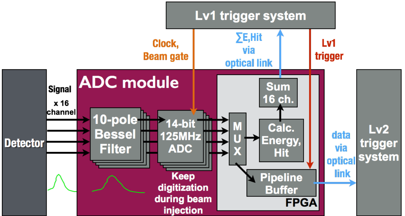
Figure 2.33: 14-bit 125-MHz ADC module with a 10 pole Bessel Filter.
