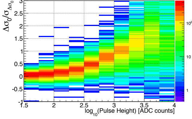
Figure 5.9: The significance of the difference of \sigma_0 between the photon-rich sample and the neutron-rich sample vs. pulse-height distribution for all channels of the CsI calorimeter.
