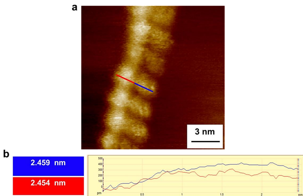
Figure 11. a , STM image of an interacted supramolecular structure arrays of Ni-C12P / SWNT complex on HOPG surface (15 nm × 15 nm, I_t = 0.020 nA, V_{\text{sample}} = 0.130 V) b , The topographic profile showing the molecular length on the upper and lower SWNTs surface, which equals 2.454 and 2.459, respectively; with height difference between them around 0.1 nm.
