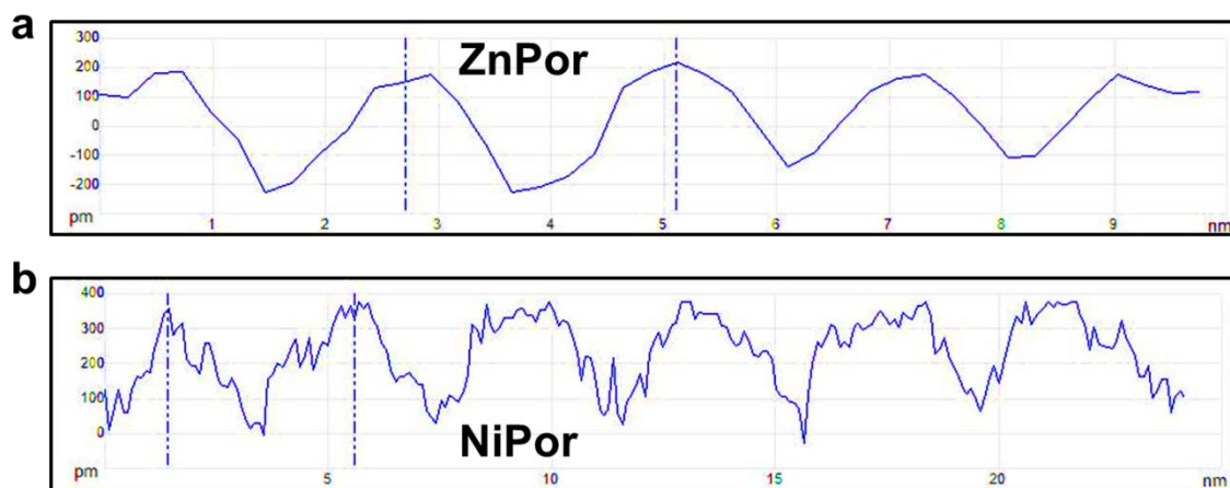
Figure 5. Topographic profiles representing the center to center distances (marking with the blue lines in Fig. 4a and 4g) for a , ZnPor molecules (equals about 2.2 \pm 0.2 nm) and b , NiPor molecules (equals about 3.8 \pm 0.3 nm) on SWNTs surface.
