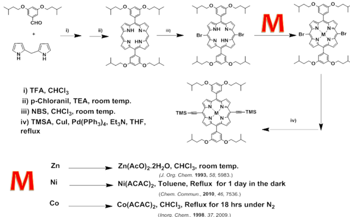
Scheme 1. Procedures for synthesizing 5,15-bis(3,5-bis(isopentyloxyphenyl)-10,20-bis(trimethylsilyl)ethynylporphyrato] with different central metals i.e. Zn, Ni and Co.
