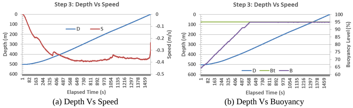
Fig. 59 Robot's ascent
