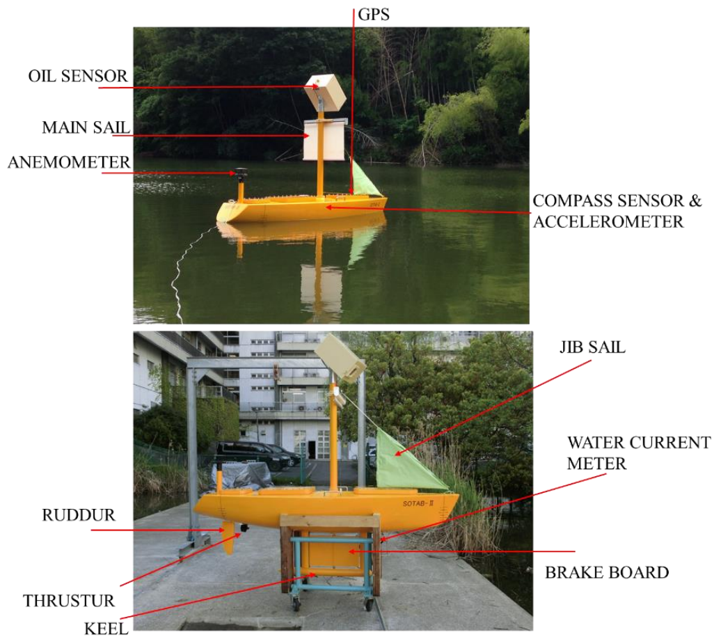
Figure 2.1 SOTAB-II prototype
