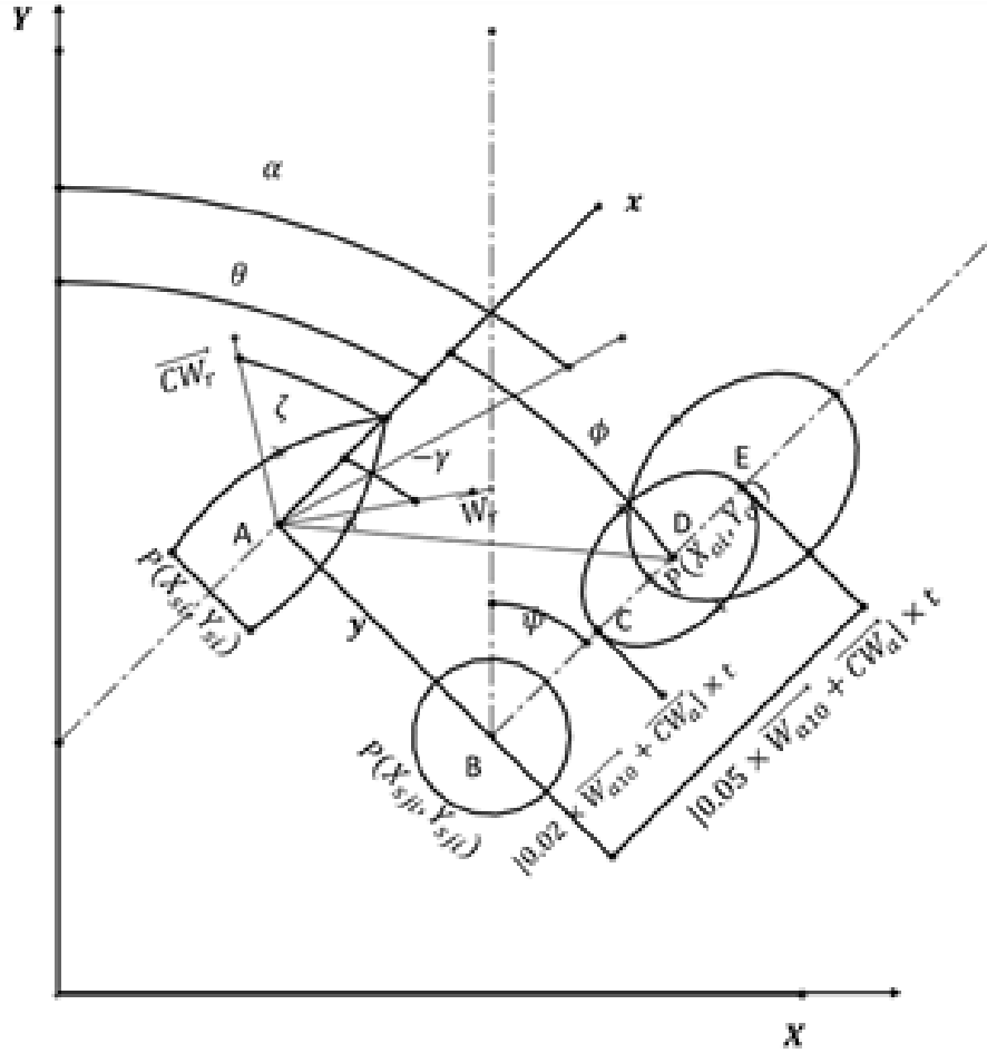
Figure 3.1 Reference system
