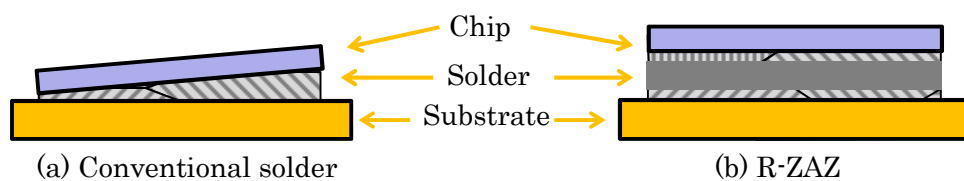
Fig. 3.3 Cross-sectional schematic of effect of reducing chip tilting by residual Al layer.
