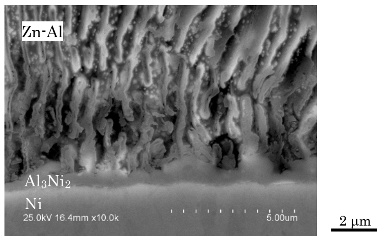
Fig. 2.12 Magnified view near bonded interface of the joint formed using the 45/15/45 μm ZAZ shown in Fig. 2.11b.
