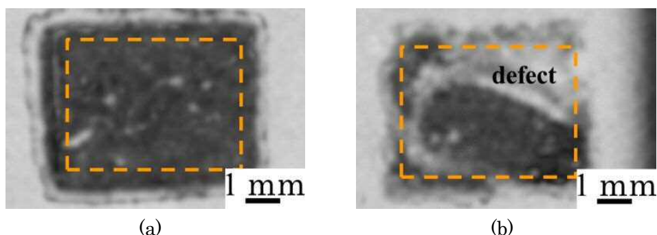
Fig. 4.8 SAT images of Si chip-to-Ni-plated Cu substrate formed using ZAZ, after bonding at 385°C for 3 min under an applied pressure of 0.4 kPa in N 2 with oxygen concentrations of (a) 25 and (b) 125 ppm.
