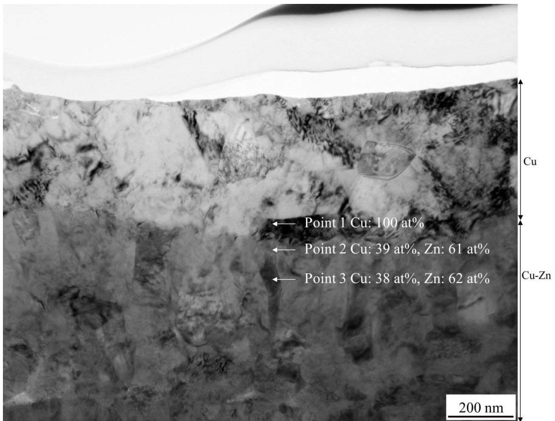
Fig. 4.17 Cross-sectional TEM images of CZAZC and EDX results obtained at each point.
