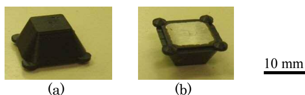
Fig. 6.1 Transfer molded Si chip-to-Cu/Ni/Au substrate joint; (a) top view, (b) back side view.
