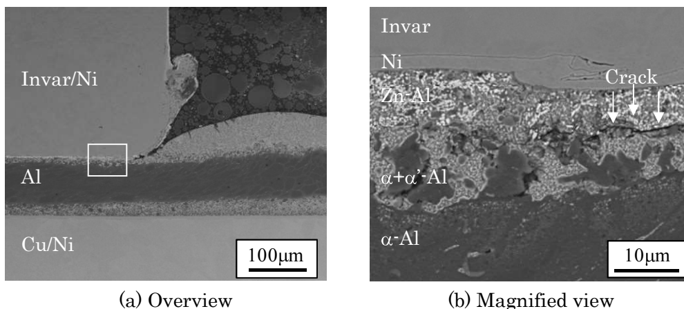
Fig. 3.13 Cross-sectional microstructures of Invar/Ni-to-Cu/Ni substrate joint formed using R-ZAZ of 28/80/28 \mu\text{m} after thermal cycle of 300 cycles.
