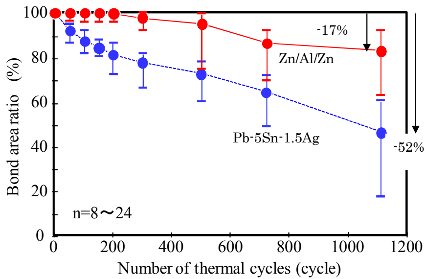
Fig. 3.12 Changes of bond area ratio of Invar-to-Cu/Ni substrate joints formed using R-ZAZ of 28/80/28 \mu\text{m} and Pb-5Sn-1.5Ag through thermal cycle test between -55^{\circ}\text{C} and 150^{\circ}\text{C} .
