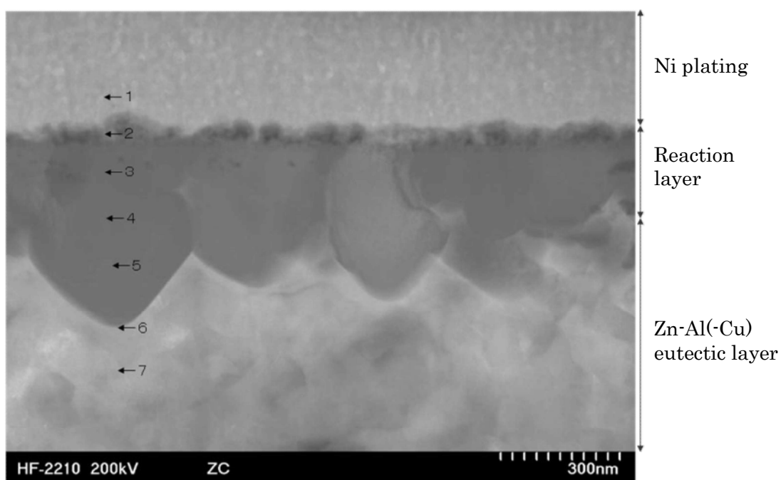
Fig. 5.12 HAADF-STEM images of Region B in Fig. 5.11.
