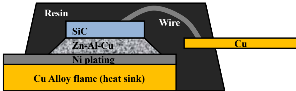
Fig. 6.3 Cross-sectional schematic image of SiC TO-220 package formed using CAZAC.
