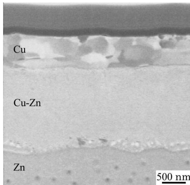
Fig. 4.16 Cross-sectional SIM image of CZAAC.
