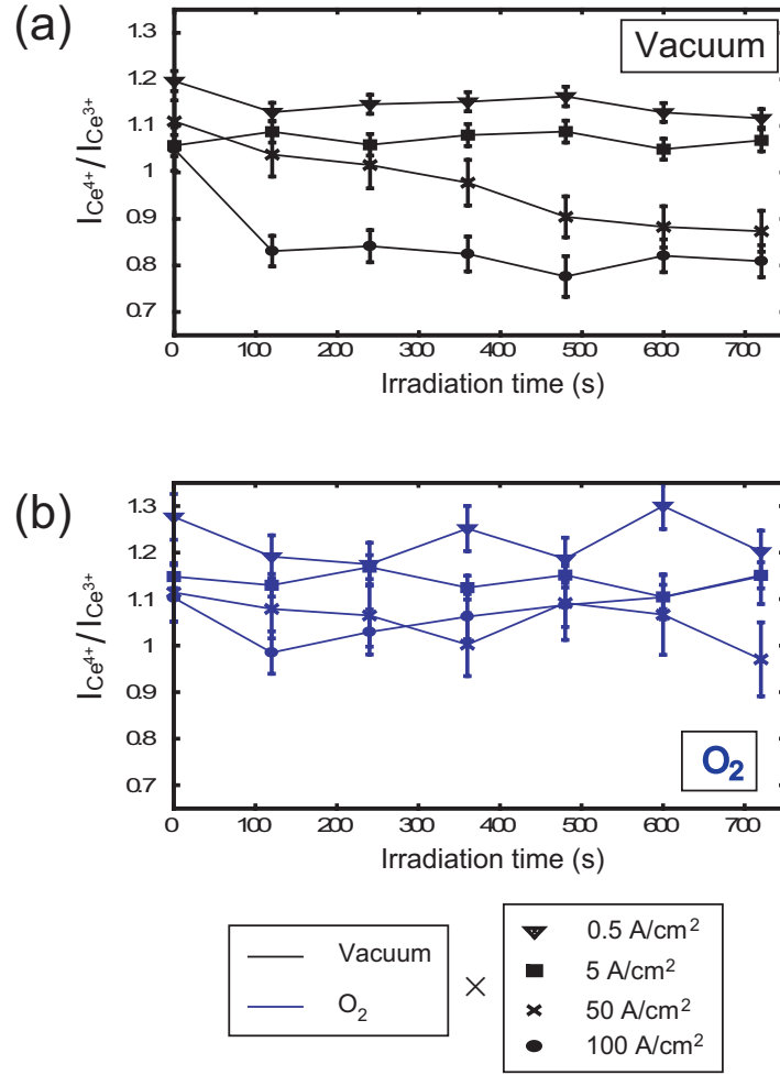
Figure 4.6: Results of EELS measurements of CeO 2 in vacuum and O 2 under electron flux of 0.5, 5, 50 and 100 A/ cm 2 . Horizontal axis of the graph is irradiation time. Vertical axis of the graph is a ratio of the peak intensity of Ce 4+ and Ce 3+ .
