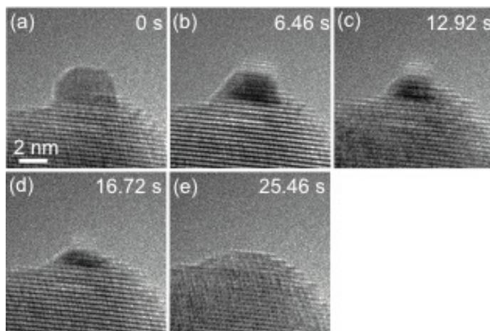
Figure 4.3: (a)-(e) Successive ETEM images of a AuNP on \text{CeO}_2 under 100 \text{ A/ cm}^2 electron beam irradiation. The recording time is shown in each image.
