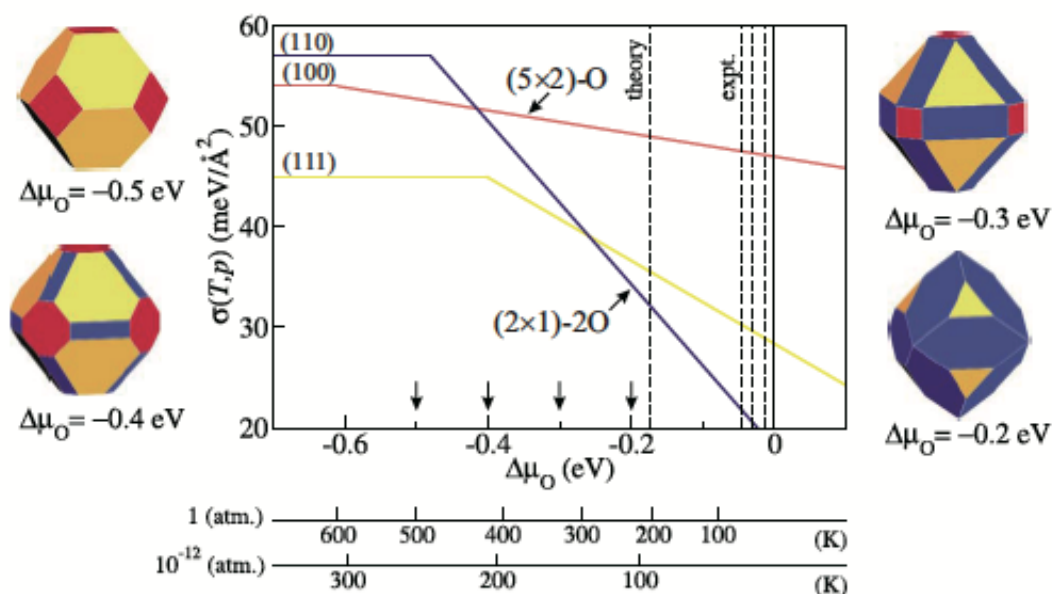
Figure 8.8: Dependency of surface free energies for O at Au (100), Au (110) and Au (111) on the oxygen chemical potential. The predicted nanoparticle shapes of -0.5, -0.4, -0.3 and -0.2 eV of the oxygen chemical potential are also shown. The facets are colored as red for (100), blue for (110) and orange for (111) [82].
