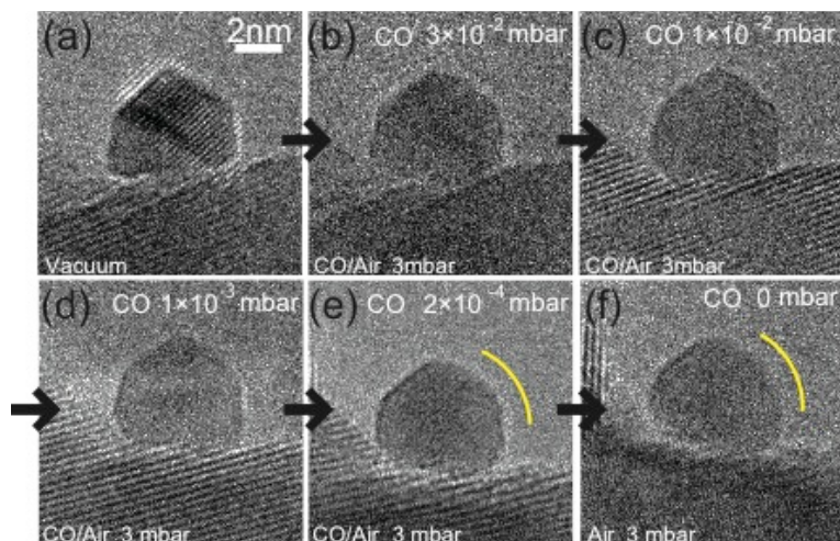
Figure 6.3: ETEM images of a AuNP obtained in the mixture of 1 vol.% CO/air and air. The morphology of the AuNP changes with the decrease of the CO partial pressure. The AuNP becomes round with the decrease of the CO partial pressure. The total pressure of gases was kept at 3 mbar.
