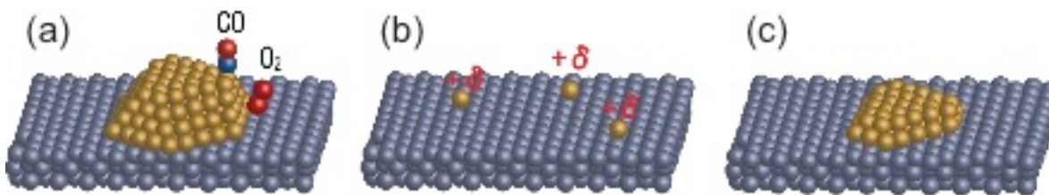
Figure 1.2: Reaction models. (a) Perimeter interface model [11], (b) Au cation model [31,32] and (c) Two layers model [33,34].
