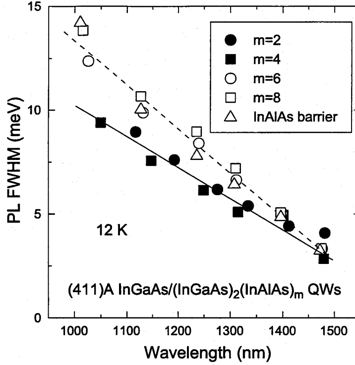
Figure 4.16: FWHMs of PL peaks at 12 K from the (411)A InGaAs/(InGaAs) 2 (InAlAs) m QWs [ m = 2 (closed circles), 4 (closed squares), 6 (open circles) and 8 (opens squares)] and the (411)A InGaAs/InAlAs QWs (open triangles) grown at T_s = 540^\circ\text{C} .
