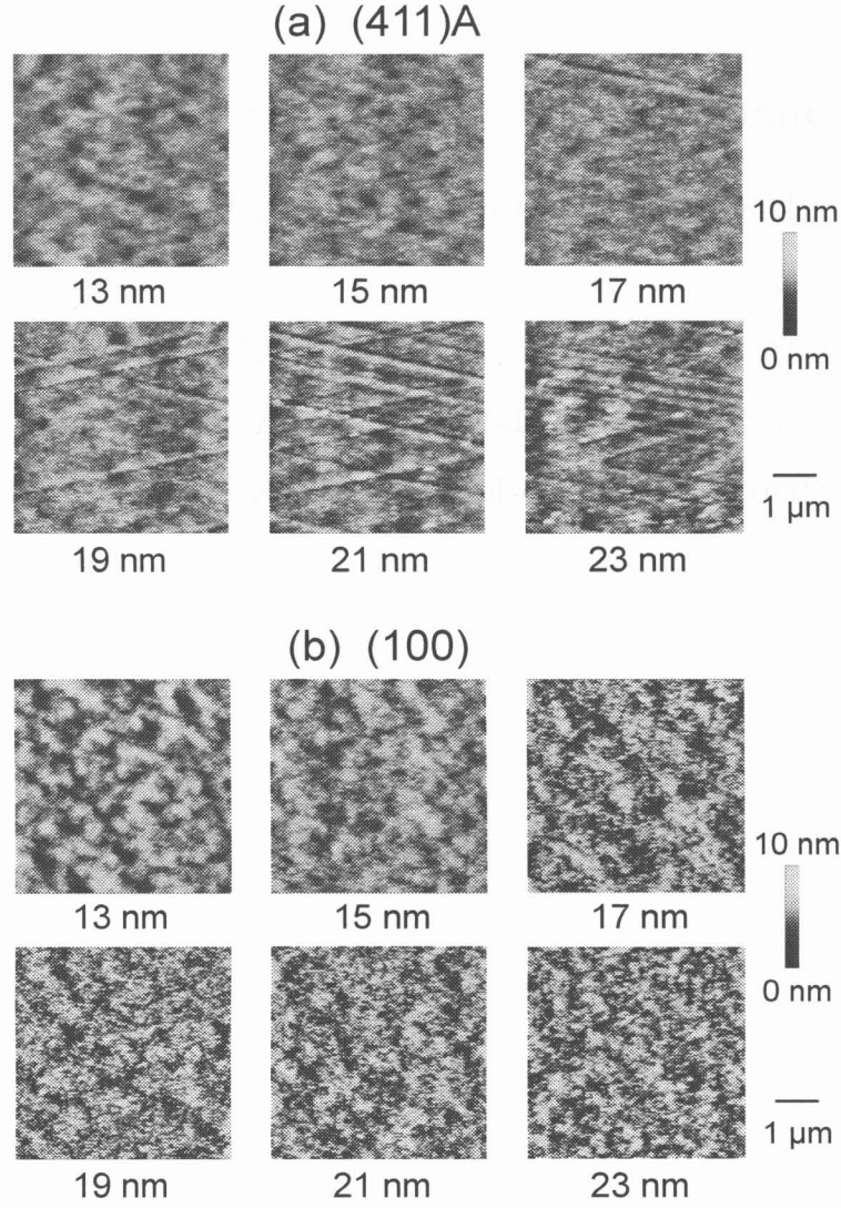
Figure 3.12: AFM images of (a) the (411)A and (b) (100) \text{In}_{0.25}\text{Ga}_{0.75}\text{As} top layer with thickness of L_w (13 - 23 nm). The scan area is 5\text{ }\mu\text{m} \times 5\text{ }\mu\text{m} .
