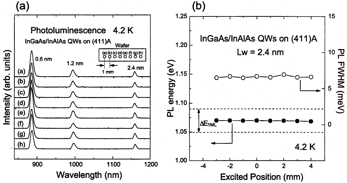
Figure 4.13: Excited position dependence of (a) PL spectra (4.2 K) from the (411)A \text{In}_{0.53}\text{Ga}_{0.47}\text{As}/\text{In}_{0.52}\text{Al}_{0.48}\text{As} QWs with L_w = 0.6 , 1.2 , and 2.4 nm, and (b) PL peak energy and FWHM of the (411)A QW with L_w = 2.4 nm. \Delta E_{1ML} indicates a calculated PL energy difference for 1 ML fluctuation of the QW.
