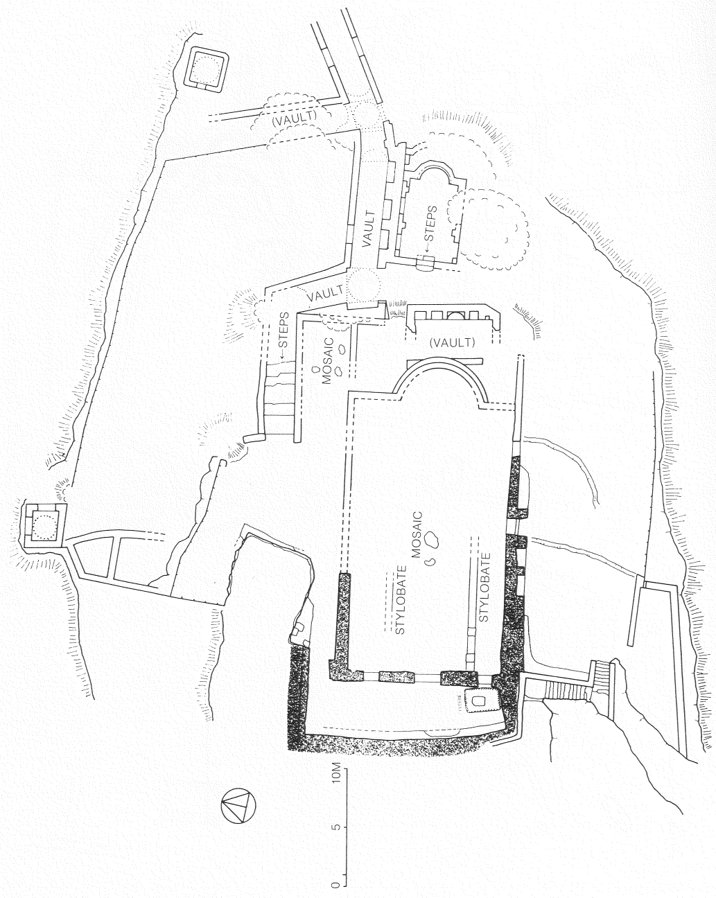
Fig. 6. Plan of Church III, Gemiler Ada.
