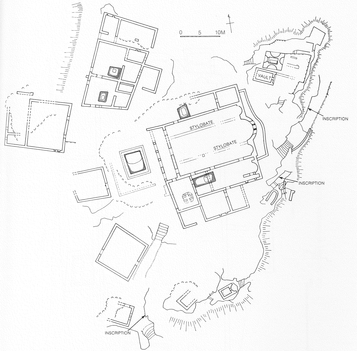
Fig. 9. Plan of Karacaören Ada Basilica.
