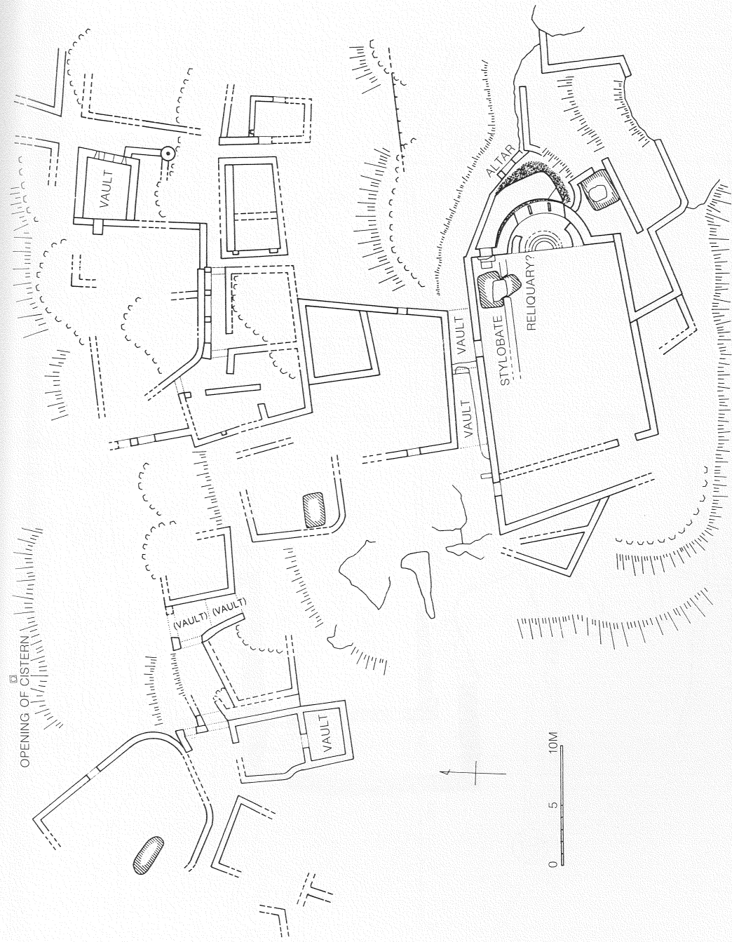
Fig. 5. Plan of Church II, Gemiler Ada.
