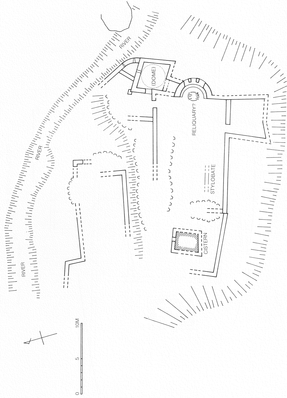
Fig. 12. Plan of Mustafa Basilica.
