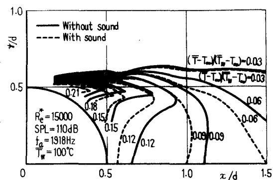
図3-13 等平均温度 (\bar{T} - T_\infty)/(T_w - T_\infty) 線図 ( Re^* = 15000 , f_a = 1918 Hz, SPL = 110 dB, \bar{T}_w = 100^\circ\text{C} )
