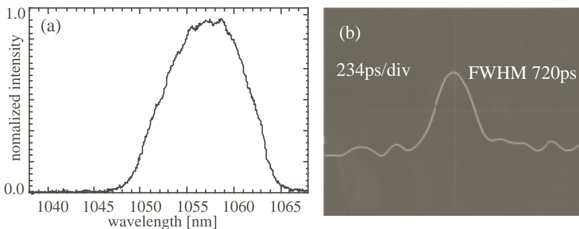
Figure 2.10: Pulse shape and spectrum out of the pulse stretcher. (a) Spectrum with the spectral width of 10nm. (b) Pulse shape with the chirped pulse duration of 720ps.
