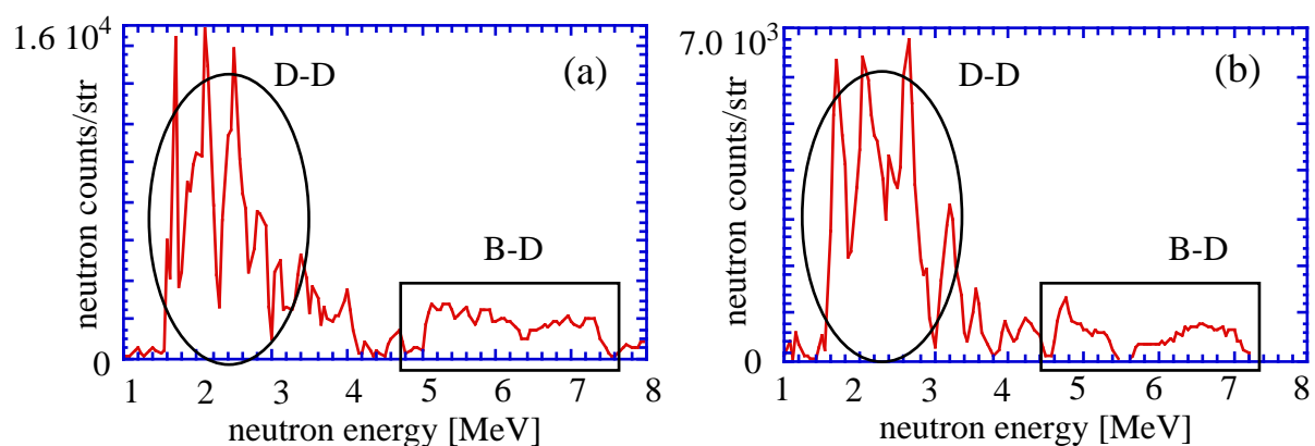
Figure 7.3: The neutron spectra generated from D-B fusion reaction ( \sim 6 MeV) with D-D reaction ( \sim 2.45 MeV). (a) The spectrum at the 86.5^\circ . (b) The spectrum at the 145^\circ .
