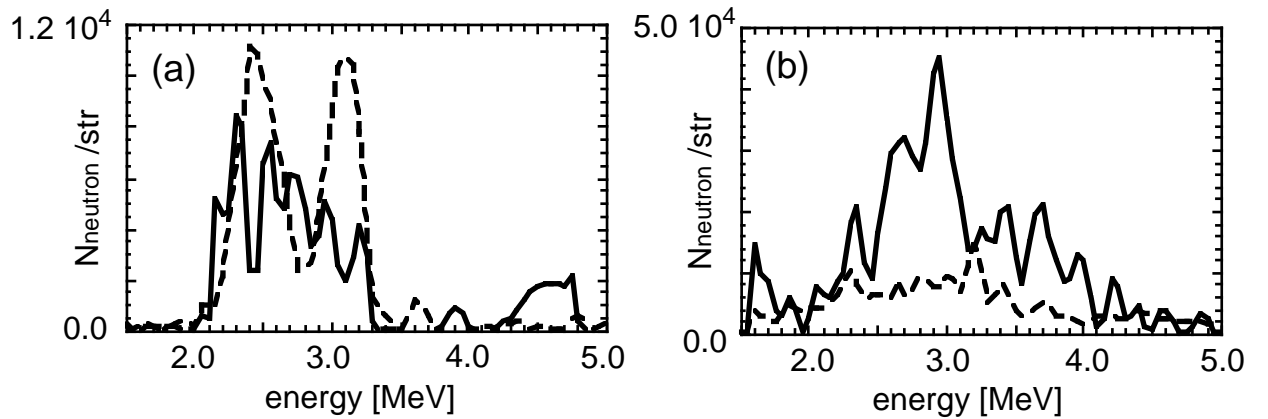
Figure 6.6: Laser intensity dependence at neutron spectra. (a) Neutron spectra at intensities of 10^{18}W/cm^2 at 43° (solid line) and 87° (dotted line) from the target normal. (b) Neutron spectra at intensities of 10^{19}W/cm^2 . The other figure conditions are as same as Fig. 6.6(a).
