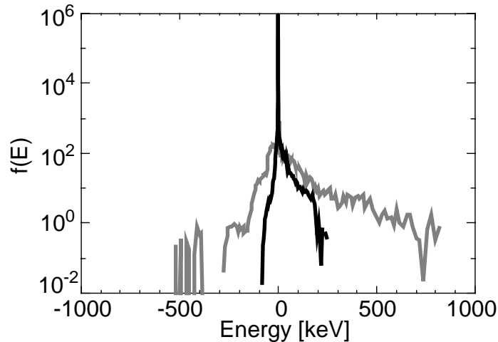
Figure 6.7: The ion energy distribution from the PIC simulation results. The black and grey solid lines are the distribution transverse and parallel to the target surface.
