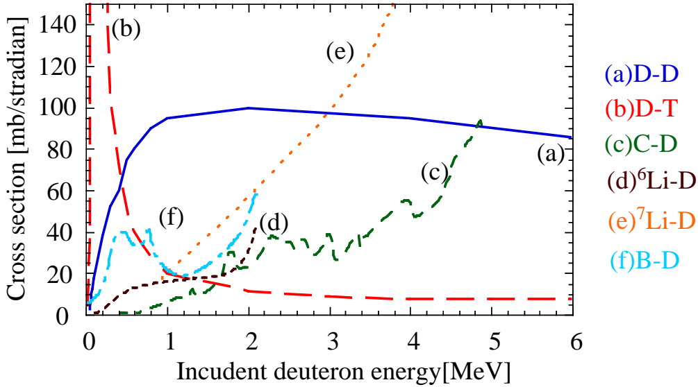
Figure 7.1: The cross section of the neutron generated (a)D-D ( d[d,n]^3\text{He} ), (b)D-T ( d[t,n]^4\text{He} ), (c)D-C ( ^{12}\text{C}[d,n]^{13}\text{N} ), (d)D- ^6\text{Li} ( ^6\text{L}[d,n]^7\text{Be} ), (e)D- ^7\text{Li} ( ^7\text{L}[d,n]^8\text{Be} ) and (f)D- ^{10}\text{B} ( ^{10}\text{B}[d,n]^{11}\text{C} ) fusion reaction with the initial deuteron energy.
