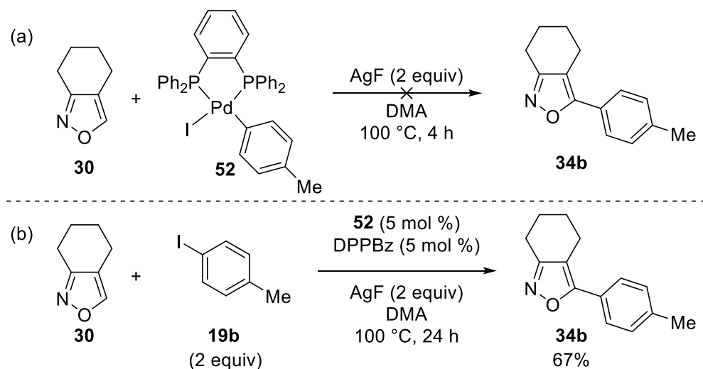
Scheme 2-22. Direct arylation using Pd complex 52
