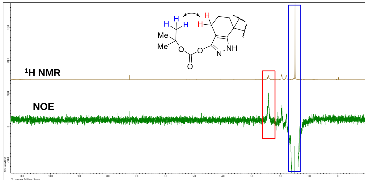
Figure 3-4 ^1\text{H} NMR and NOE chart of 89
