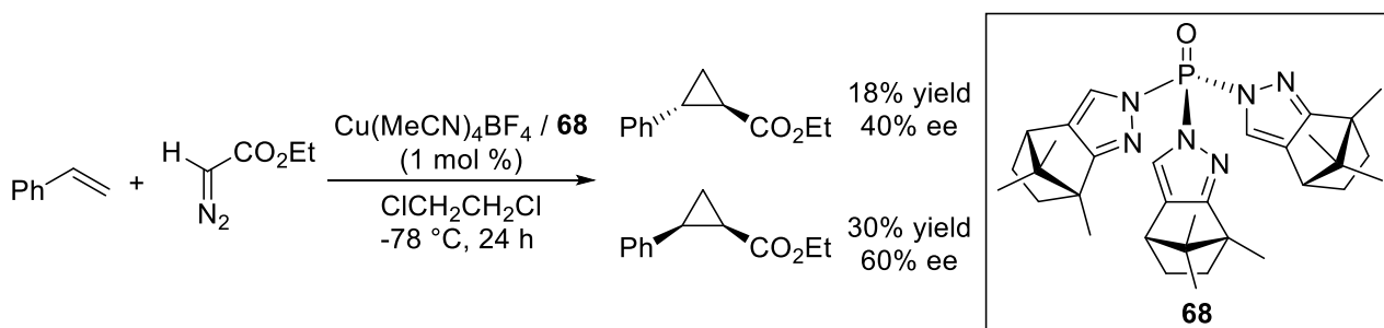
Scheme 3-1. Cu-catalyzed asymmetric cyclopropanation using chairlike pyrazole ligand
