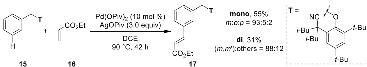
Scheme 2-5. Pd-catalyzed meta -selective functionalization
