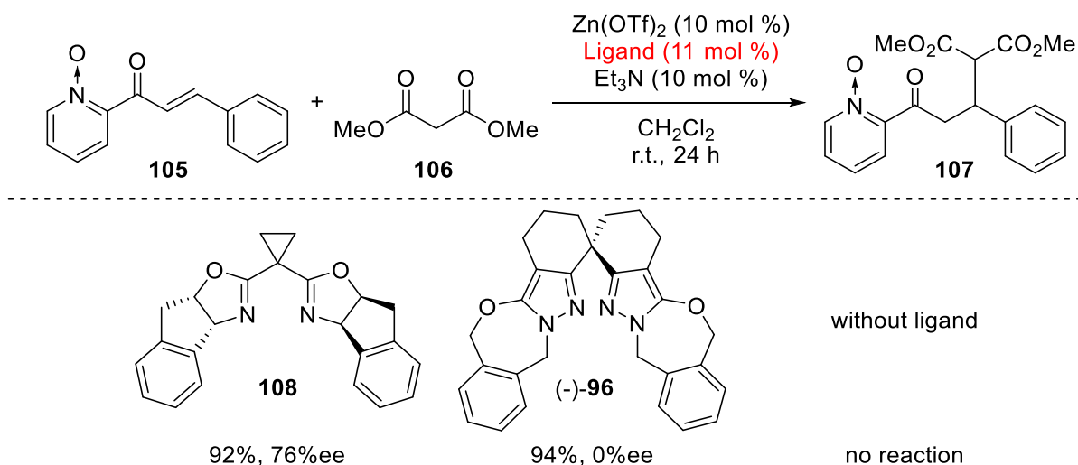
Scheme 3-18. Asymmetric Michael addition
