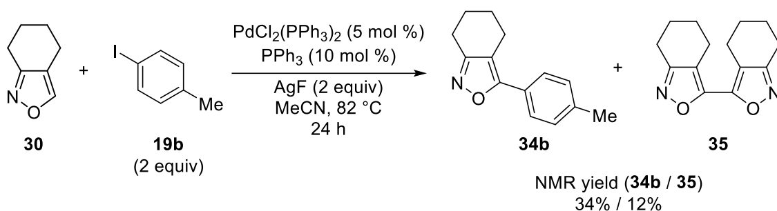
Scheme 2-14. Direct arylation of isoxazole ring at C5 position
