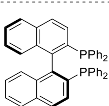
(S)\text{-BINAP} 27%, rac
