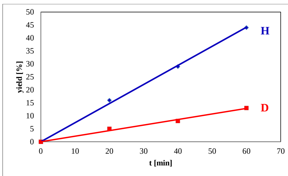
Figure 2-7. Chart of the reaction rate
