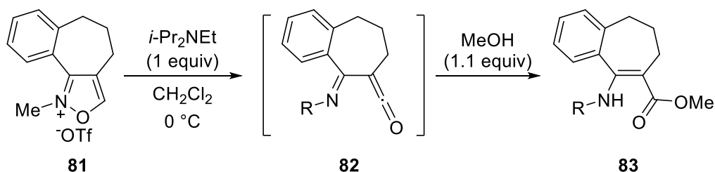
Scheme 3-4. Transformation of isoxazolium salt to β-enamino ester
