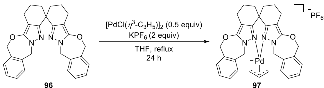
Scheme 3-14. Complexation of 96 with Pd salt
