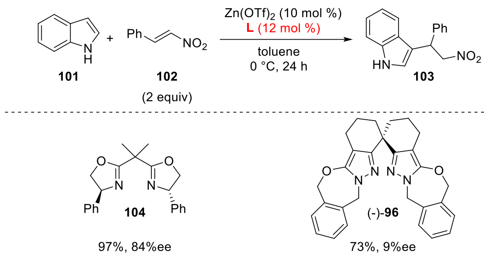
Scheme 3-17. Asymmetric Friedel-Crafts reaction
