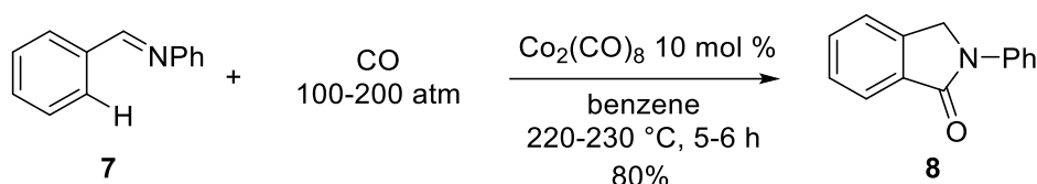
Scheme 2-2. Co-catalyzed carbonylation of aromatic imine 7
