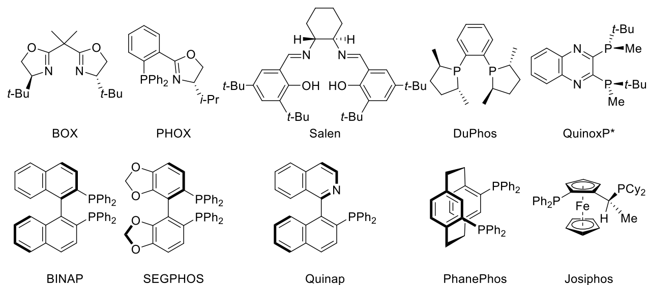
Figure 1-2. Chiral ligands
