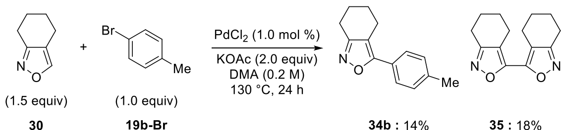
Scheme 2-11. First trial of direct arylation of isoxazole 30 at the C5 position
