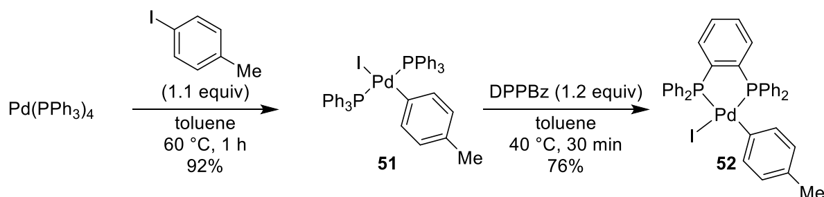
Scheme 2-21. Synthesis of Pd complex 52
