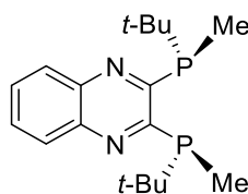
(R,R)\text{-QuinoxP}^* 48%, rac
