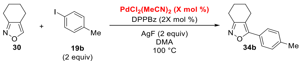
Figure 2-10. Kinetic Study
