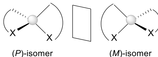
Figure 1-2. Chiral spiro skeleton
