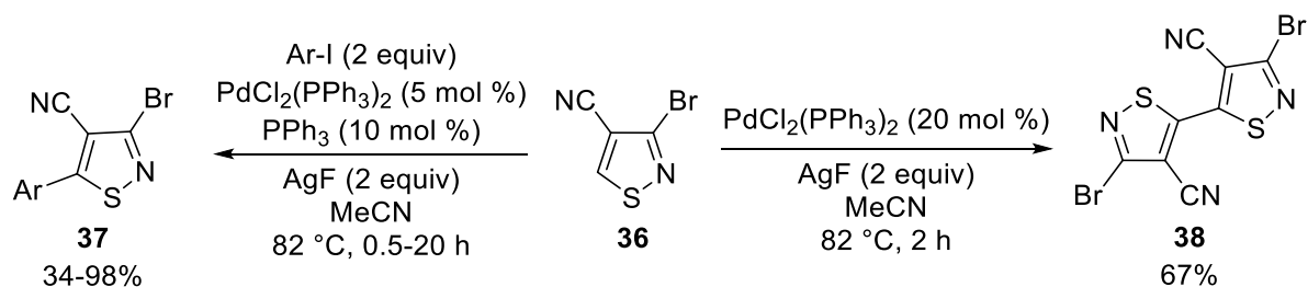
Scheme 2-13. Pd-catalyzed direct arylation of isothiazole
