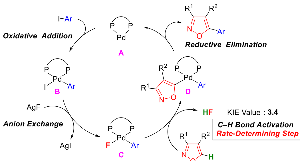
Figure 2-9. Plausible mechanism
