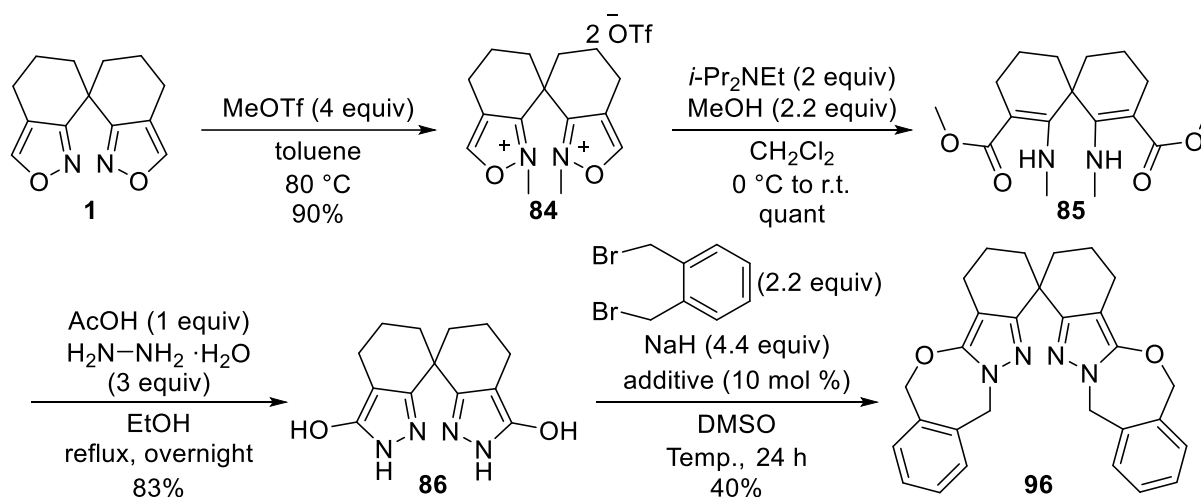
Scheme 3-19. Synthesis of 96
