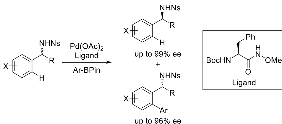
Scheme 2-27. Kinetic Resolution of Benzylamines via Palladium(II)-Catalyzed C–H Cross-Coupling
