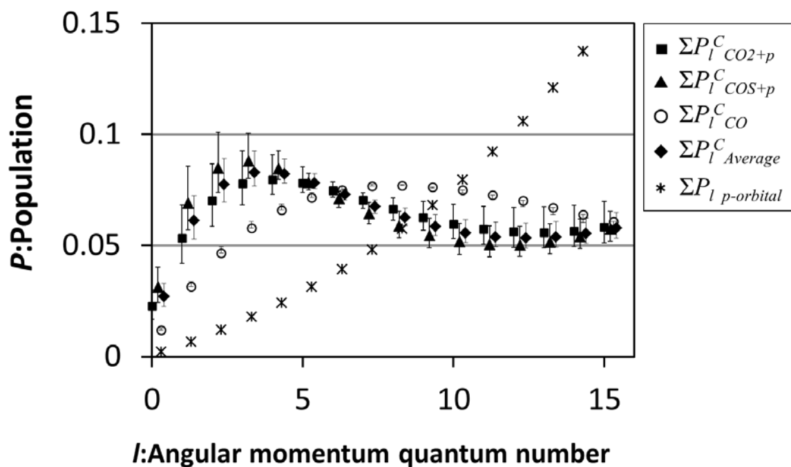
Fig.3-23 Modified angular momentum quantum number distribution of muon captured by carbon atom in CO_2 and COS ( \blacksquare : \Sigma P_l^C_{CO2+p} and \blacktriangle : \Sigma P_l^C_{COS+p} ); including the influence of p-orbital electrons partially. Angular momentum quantum number distribution of muon captured by carbon atom in CO molecule ( \circ : \Sigma P_l^C_{CO} ); average value of \Sigma P_l^C_{CO2+p} and \Sigma P_l^C_{COS+p} ( \blacklozenge : P_l^C_{Average} ); angular momentum quantum number distribution when a muon interacts with pure p-orbital electrons ( * : \Sigma P_l_{p-orbital} ) are also written in this figure.
