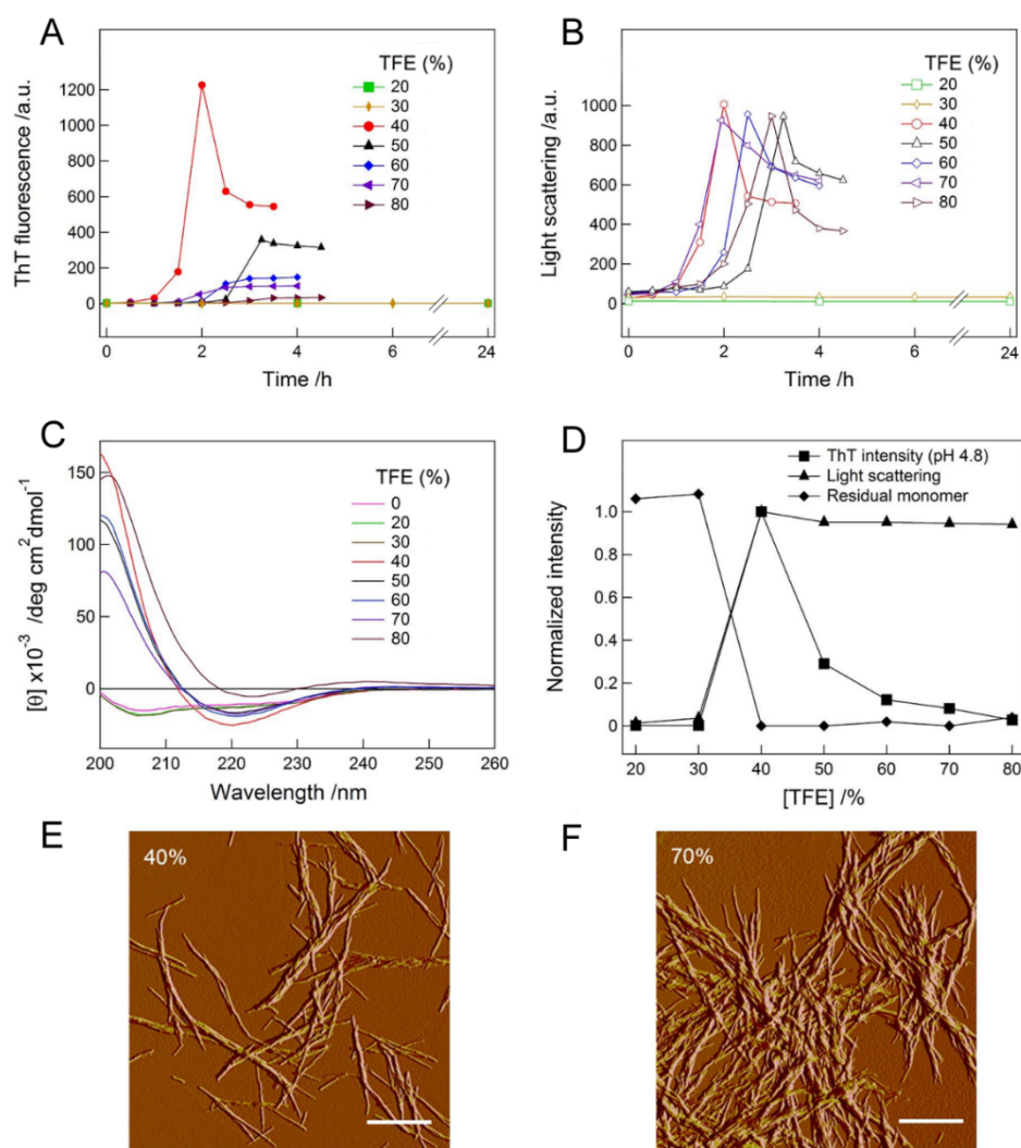
Figure 8. Aggregation kinetics and solubility of lysozyme at 5 mg mL -1 in water/TFE mixtures. (A,B) Amyloid fibrillation of lysozyme at 5 mg mL -1 monitored by ThT assay (A) and light scattering (B) in real time in 25 mM sodium acetate buffer (pH 4.8) under sonication treatment with continuous stirring. (C) The far-UV CD spectra of lysozyme solutions after incubation as shown in A. (D) Concentrations of remaining monomers (♦) and ThT (■) and light scattering (▲) intensities after incubation as shown in a Normalized values were plotted against TFE concentration. (E,F) AFM images of fibrils formed in 40 and 70% TFE. The scale bars indicate 1 μm.
