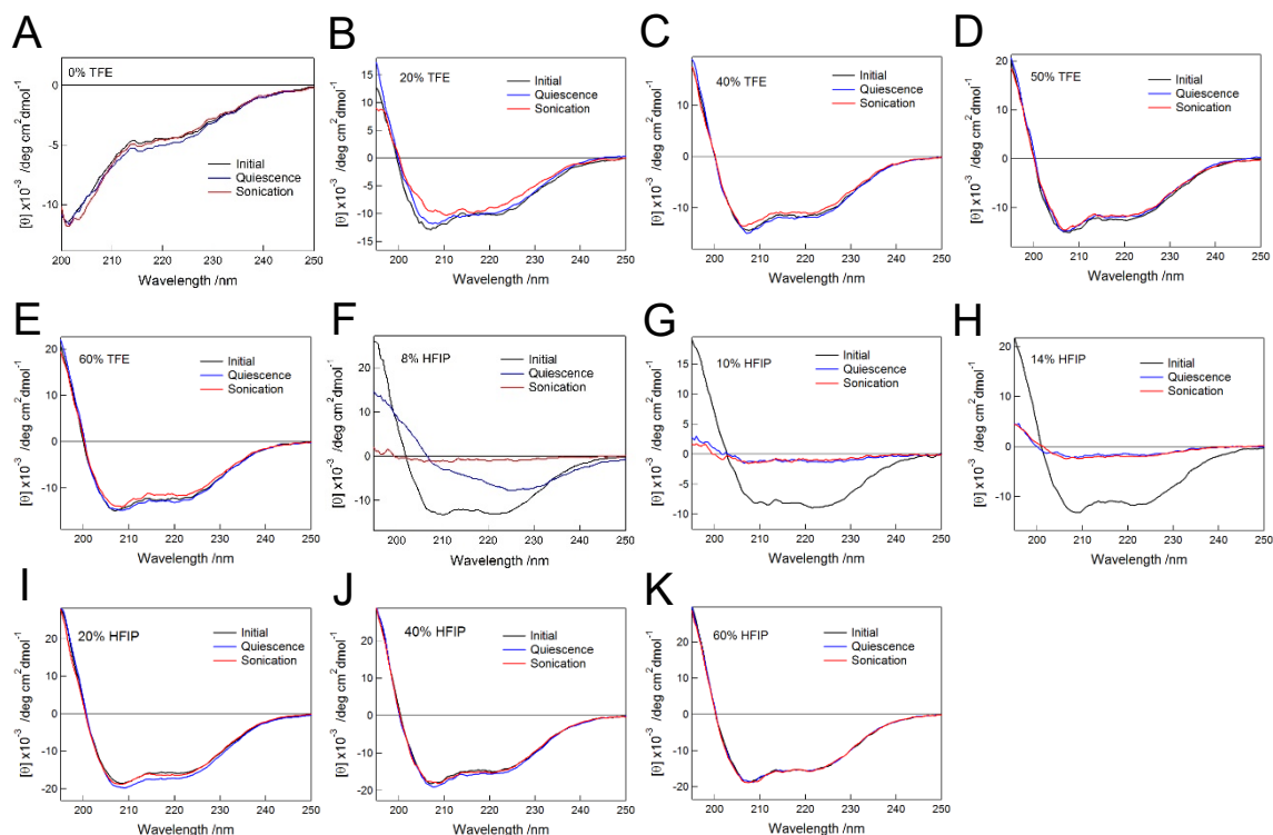
Figure 7. Alcohol-dependent aggregation of Ag-apoCytC monitored by far-UV CD. Far-UV CD spectra of Ag-apoCytC at ~5 mins (black lines) and 15 h when incubated without (blue lines) and with ultrasonication (red lines) after sample preparation were determined in the presence of TFE concentrations of 0% (A), 20% (B), 40% (C), 50% (D), 60% (E); or HFIP concentrations of 8% (F), 10% (G), 14% (H), 40% (I), 20% (J), and 70% (K).
