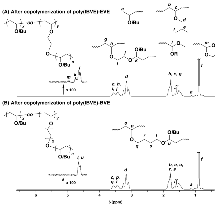
Figure 7. 1 H NMR spectra of the products of the copolymerizations of IBVE with poly(IBVE)-EVE (A) [ M_n(\text{GPC}) = 14.4 \times 10^3 , M_w/M_n(\text{GPC}) = 1.29 ], and poly(IBVE)-BVE (B) [ M_n(\text{GPC}) = 24.7 \times 10^3 , M_w/M_n(\text{GPC}) = 1.50 ] (500.16 MHz, in CDCl_3 at 30 °C; *water).
