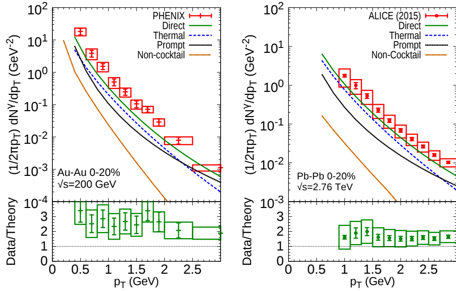
(a) Numerical simulation of photon production yield in Au+Au collisions at \sqrt{s} = 200 GeV [41]. (b) Numerical simulation of photon production yield in Pb+Pb collisions at \sqrt{s} = 2.76 TeV [41].
