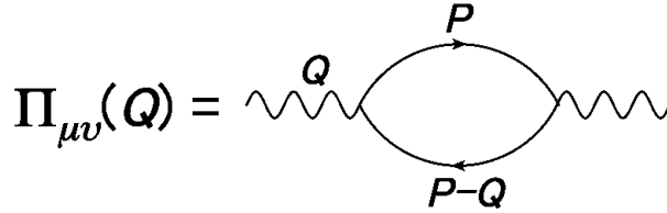
Figure 10: Diagrammatic representation of the photon self-energy, Eq. (107).
