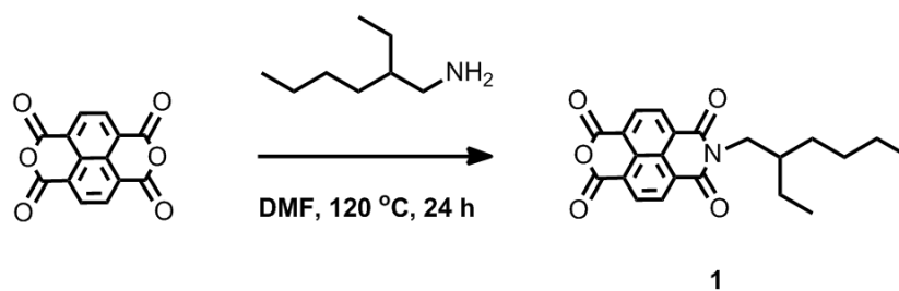
Scheme 2-2-2. Synthesis of 1 .
