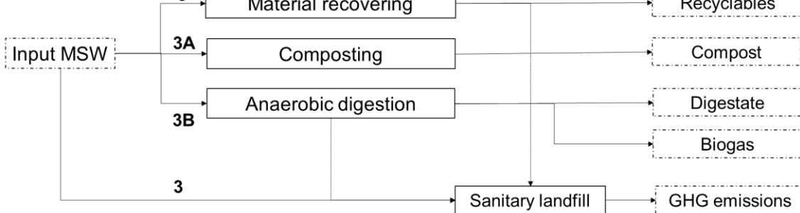
Figure 19 Diagrams of MSW flow of each scenario considered
