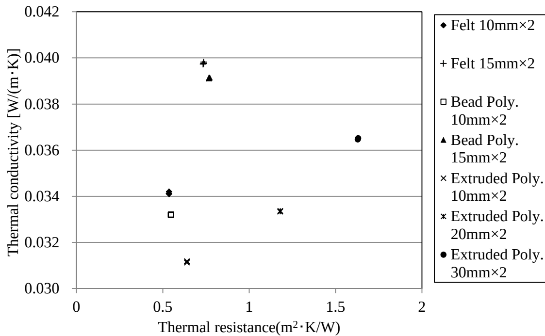
Fig. 3.12 Relationship between thermal resistance and thermal conductivity (Base plate and test sample)
