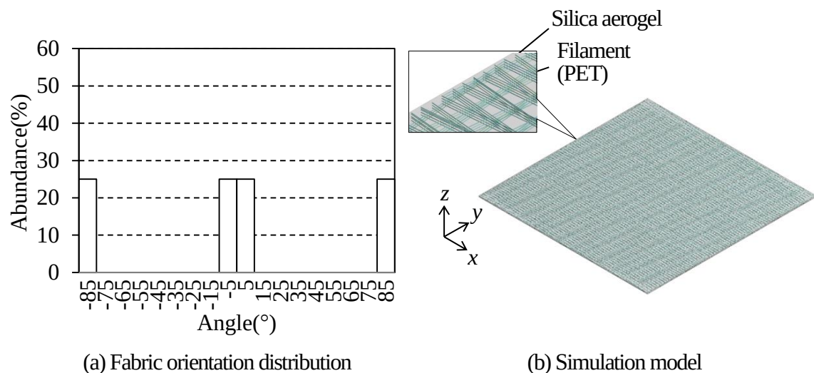
Fig. 2.18 Examined structure of thermal insulation material
