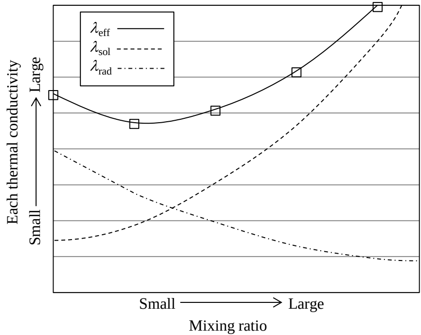
Fig. 4.14 Analyzing of combination of thermal conductivities
