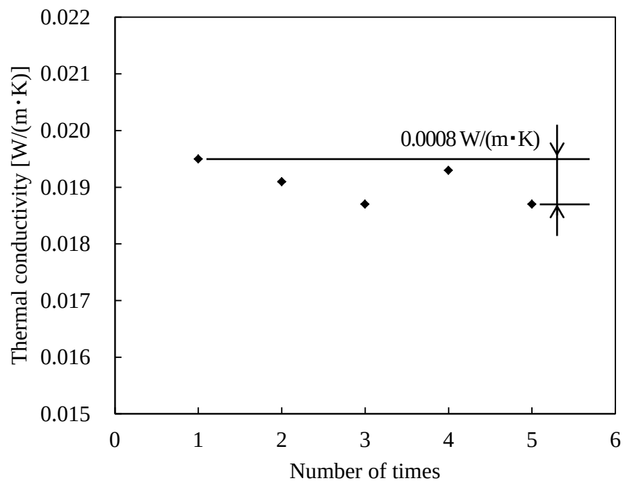
Fig. 3.17 Evaluation of reproducibility of measurement of thermal conductivity for test sample of t 1.0 mm
