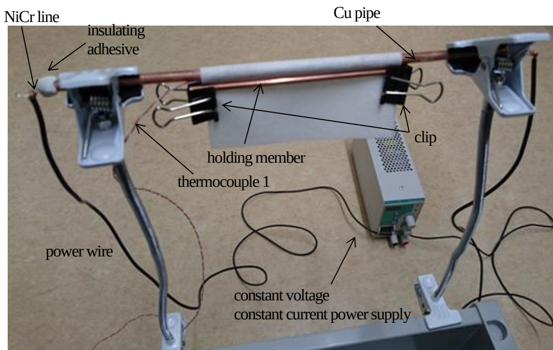
Fig. 5.1 Test equipment
