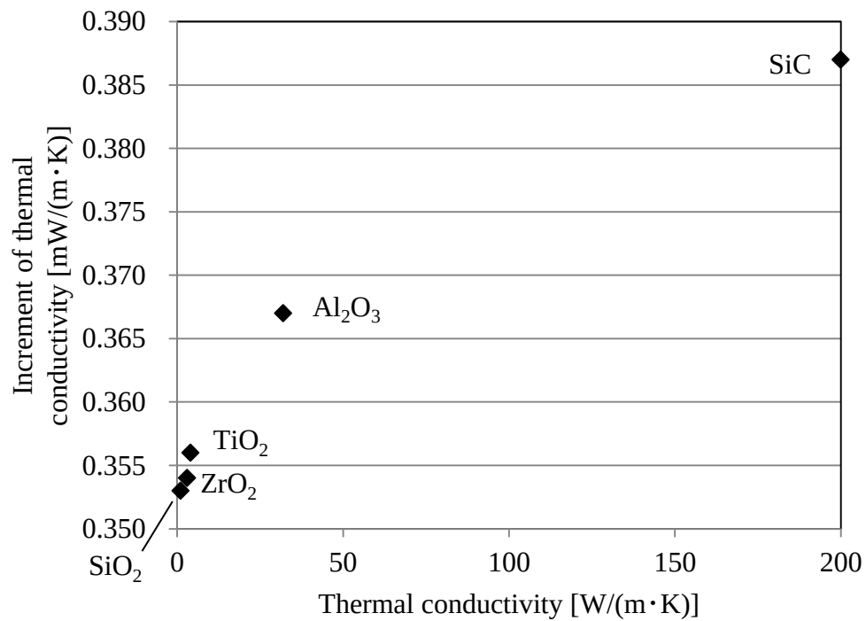
Fig. 4.19 Inclement of (B) in Fig.4.16 and thermal conductivity of radiative heat transfer reduce particles
