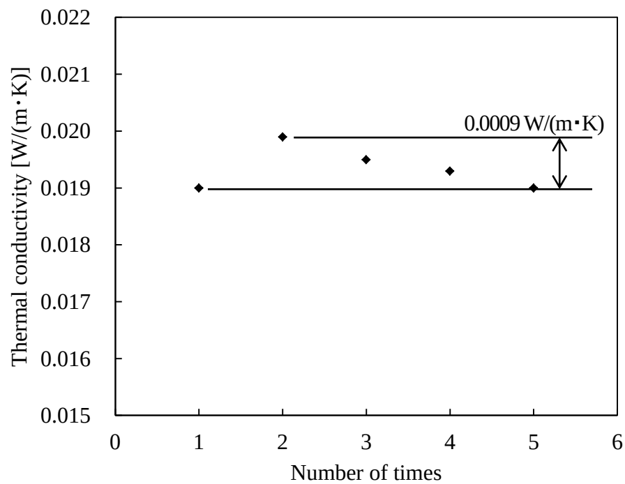
Fig. 3.18 Evaluation of reproducibility of measurement of thermal conductivity for test sample of t 2.0 mm
