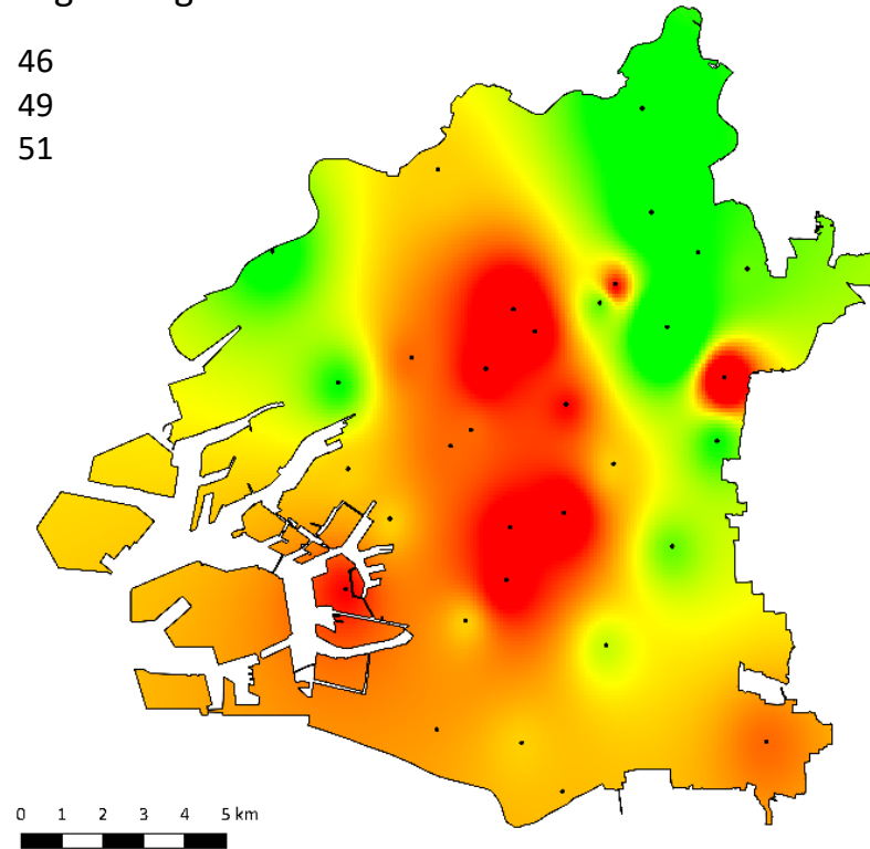
Figure 3.4.4: Interpolated observational data of the number of degree hours > 30°C (a) and the number of days where T_{min} > 25^{\circ}\text{C} (b) for Osaka City in summer 2007. The scale indicates the mean (yellow), and 2 SD from the mean (green -2 SD; red +2 SD). Black dots indicate the location of weather recording stations.
