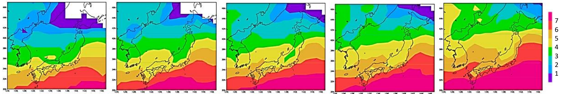
Figure 2.4.7: Projections of the estimated number of months that malaria transmission can be supported in Japan and South Korea based upon monthly average temperature generated from the CCSM4 climate model for 2001-2010, 2021-2030, 2041-2050, 2061-2070 and 2091-2100 respectively.
