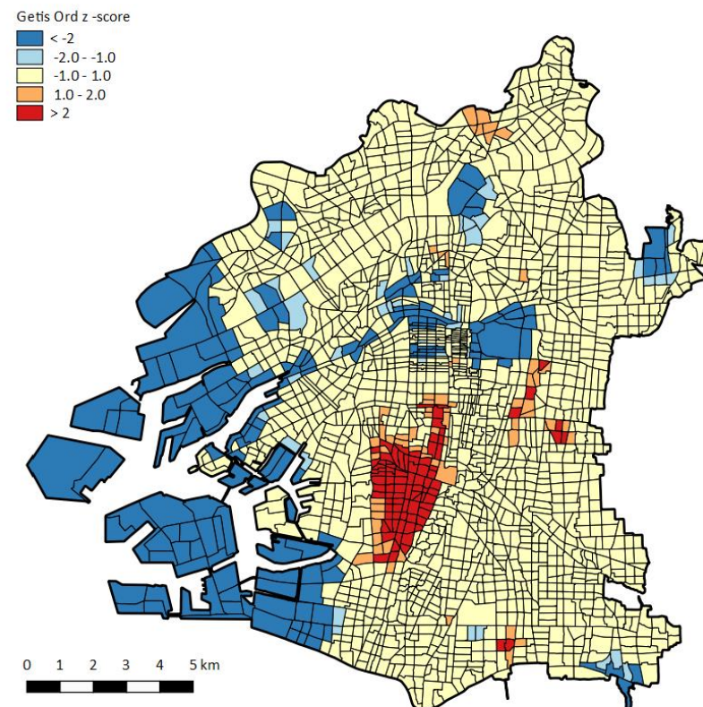
Figure 3.4.2: Output from the vulnerability index calculation, showing low (white, green) to high (orange, red) vulnerability (a); Getis-Ord z score Hot Spot Analysis, showing clusters of high (red) and low (blue) vulnerability (b).
