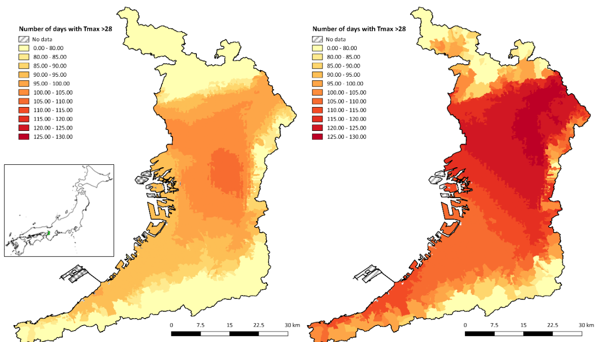
Figure 4.5.2: Projections of the annual number of days with a Tmax > 28oC, averaged for each administrative zone in Osaka Prefecture for the baseline climate (a) and 2050 (b) Inset shows the location of Osaka Prefecture in Japan.
