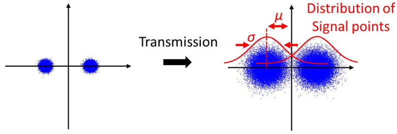
Figure 1.14: Signal degradation.
