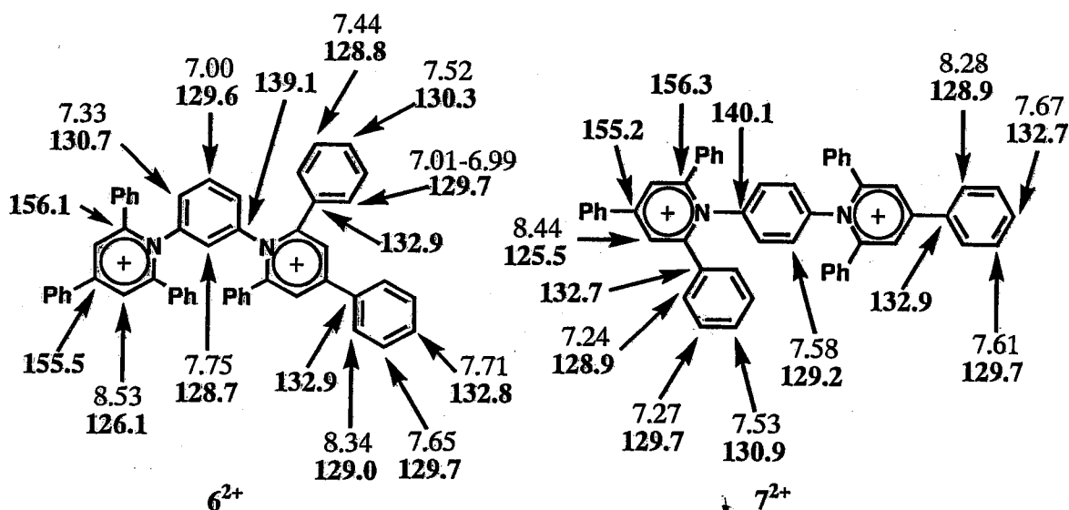
Figure 3-1. ^1\text{H} and ^{13}\text{C} chemical shifts of 6^{2+} and 7^{2+} (in DMSO- d_6 ).
