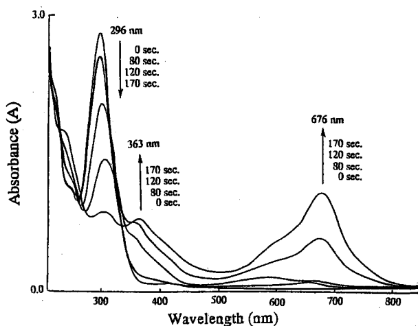
Figure 2-11. UV-vis spectral change upon reduction of 2^{3+} \cdot 3(\text{BF}_4^-) .
