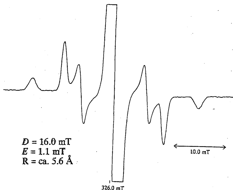
Figure 4-9. ESR spectrum of diradical 9 in MTHF-acetonitrile at -150 °C.
