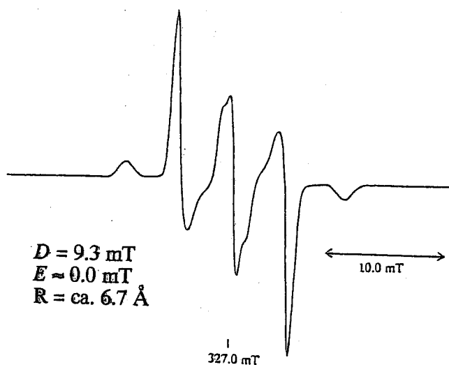
Figure 4-11. ESR spectrum of diradical 11 in MTHF-acetonitrile at -150 °C.
