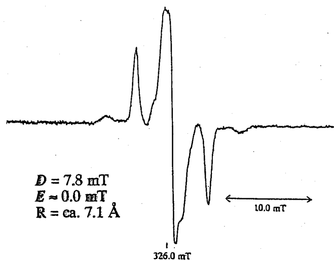
Figure 4-12. ESR spectrum of diradical 12 in MTHF-acetonitrile at -150 °C.
