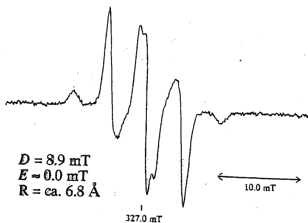
Figure 4-10. ESR spectrum of diradical 10 in MTHF-acetonitrile at -150 °C.
