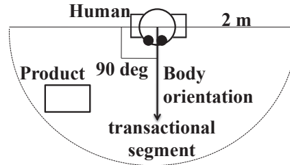
Figure 3.10 Transactional segment
