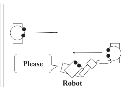
Figure 5.2 Distribution service
