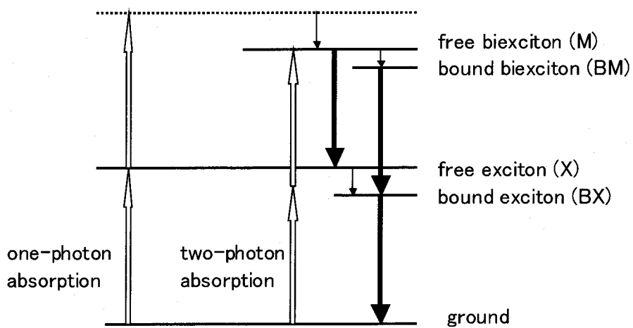
Figure 3-2. The energy diagram of the relaxation process.
