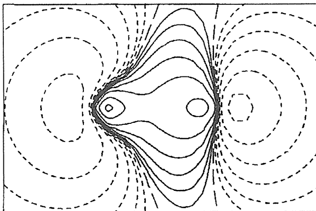
5 \sigma Molecular orbital
