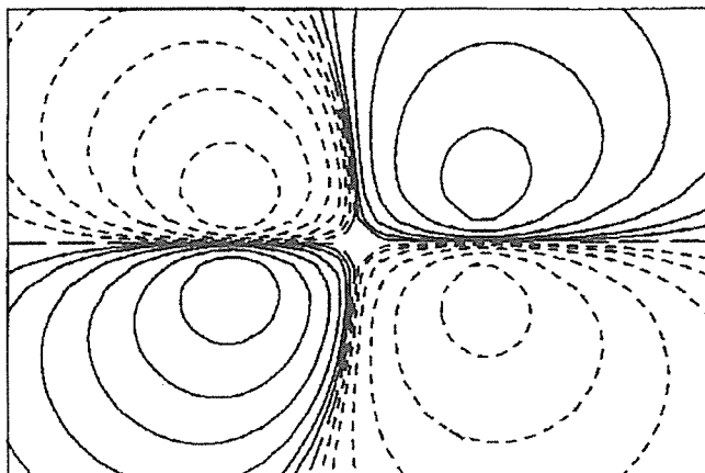
2 \pi Molecular orbital
