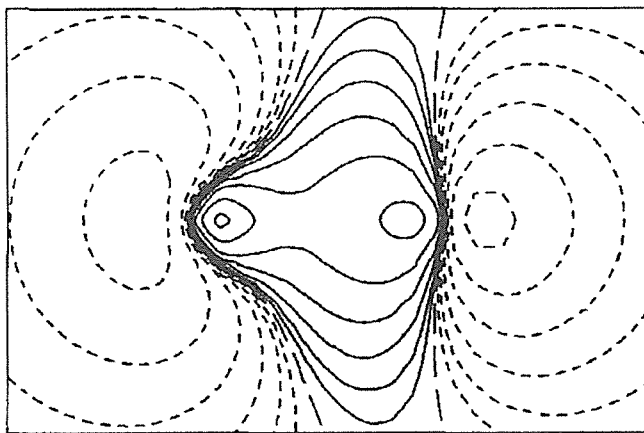
5σ Molecular orbital
