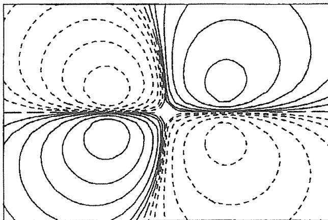
2π Molecular orbital
