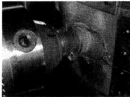
The early stages of a Cu canister weld. Note that the tool is operating at red heat
