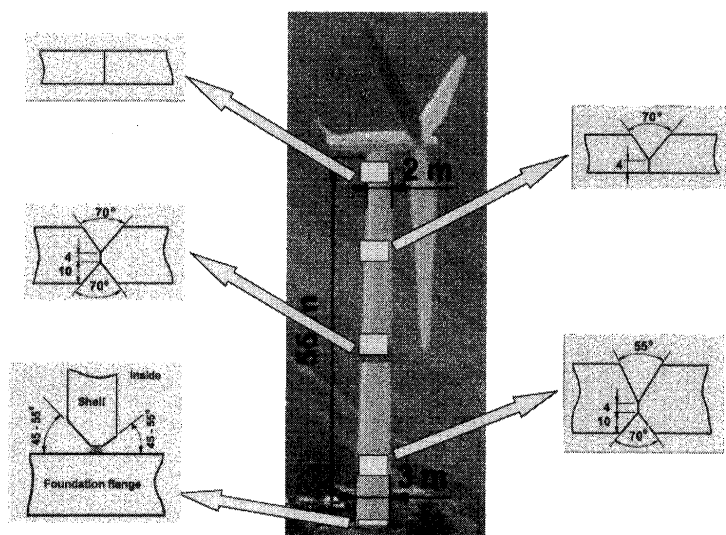
Fig.12 Typical joint preparations.
