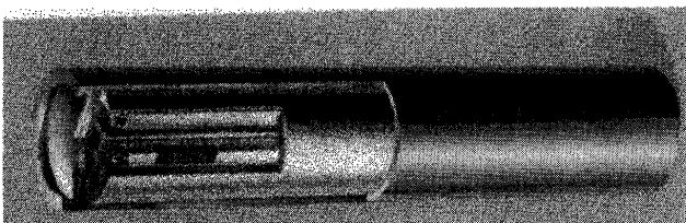
Fig.14 Cu-canister for nuclear waste.
