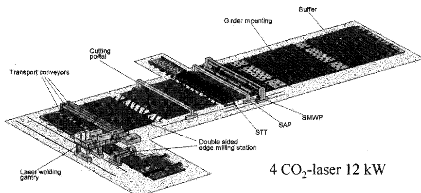
Fig.10 Laser hybrid MIG ship panel line.
