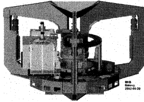
Fig.15 The welding heat rotates during the process around the fixed canister.
