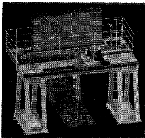
Fig.11 Concept on a YAG-laser installation.
