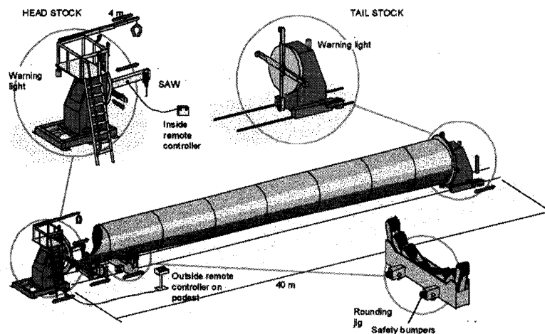
Fig.13 Setup for welding a tower.
