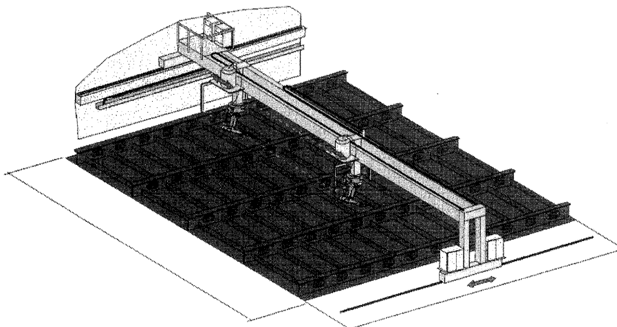
Fig.7 Robot gantry for welding of ship panels.
