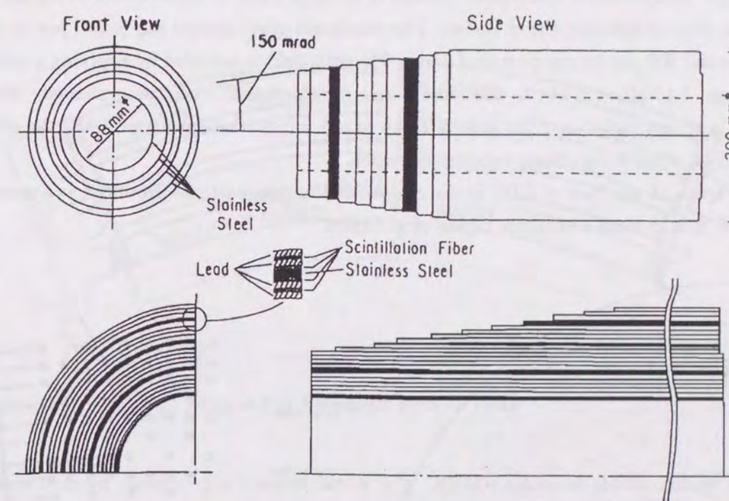
Figure 2.5: Schematic view of active mask
