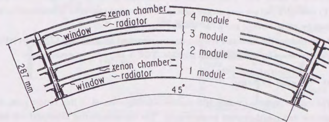
Figure 2.7: Schematic view of TRD
