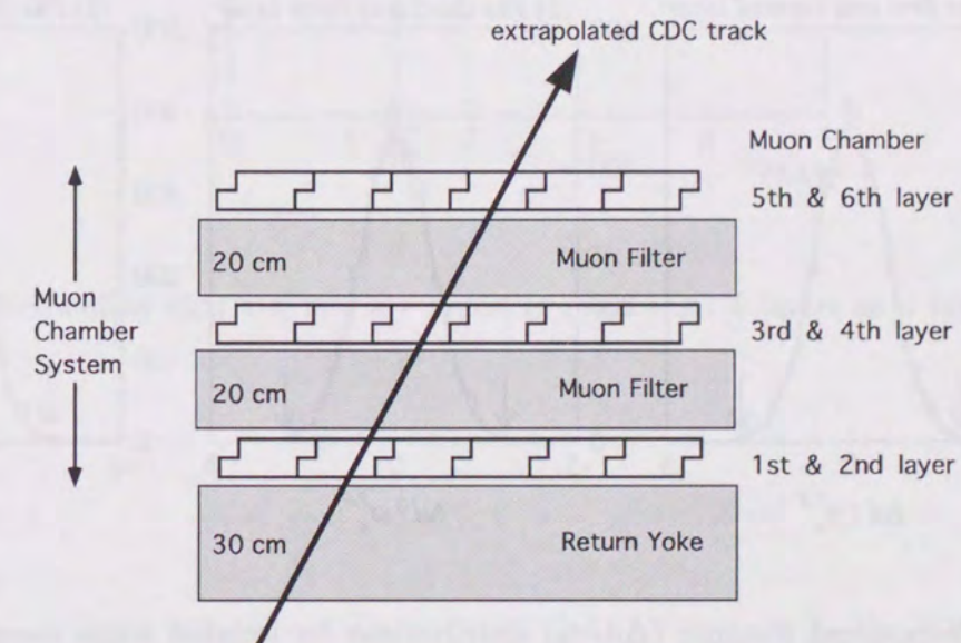
Figure 5.1: Schematic view of muon chamber system.
