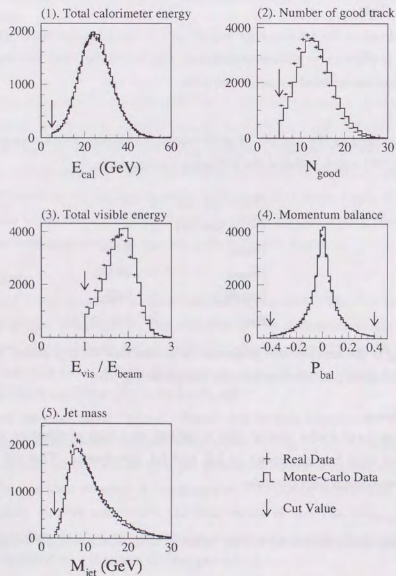
Figure 3.3: Distributions of the cut variable after hadronic event selection
