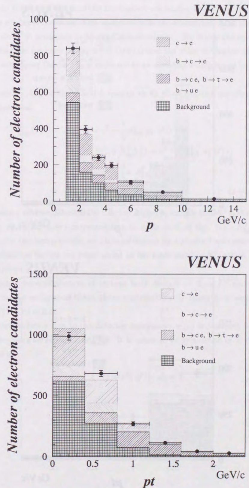
Figure 6.1: Momentum p and transverse momentum p_t spectrum of electron candidates.
