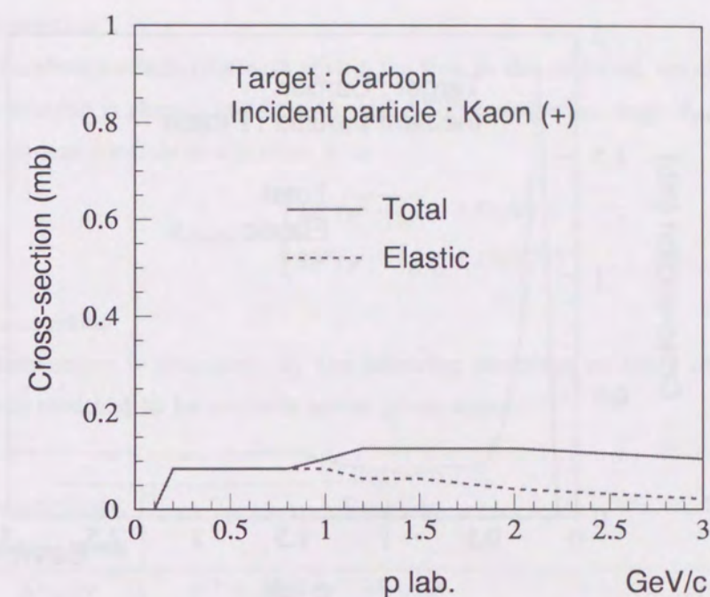
Figure C.3: Cross-section of nuclear interactions for K^+ .
