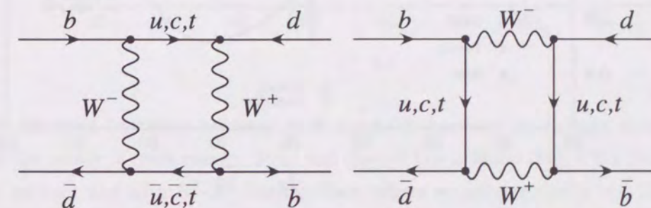
Figure 7.1: Box diagram of B^0-\bar{B}^0 mixing.
