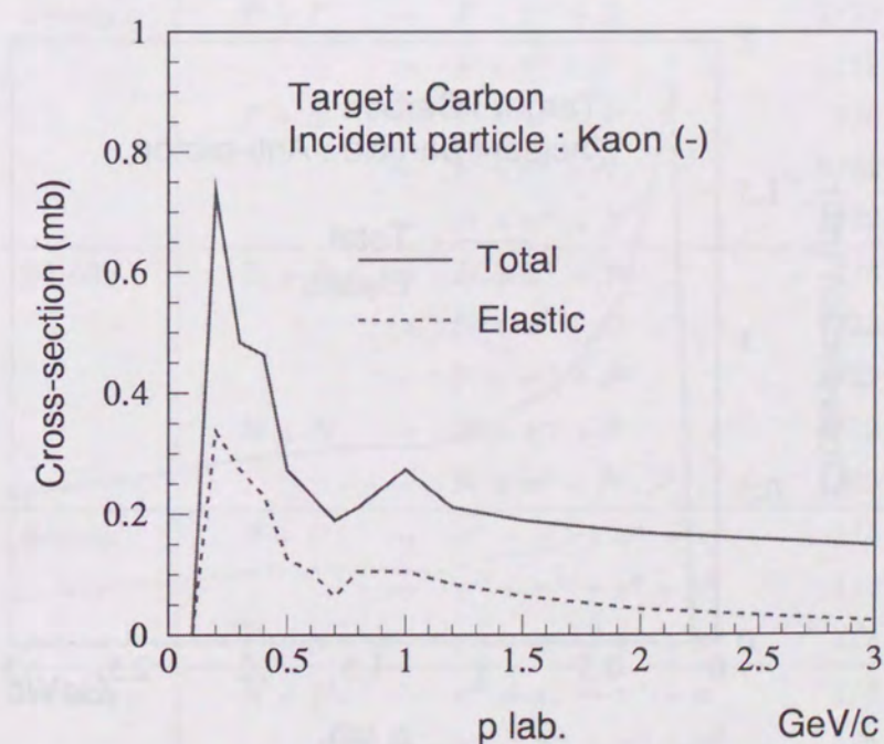
Figure C.4: Cross-section of nuclear interactions for K^- .
