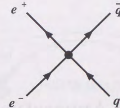
Figure 1.7: Contact interaction of e^+e^- \rightarrow q\bar{q} process
