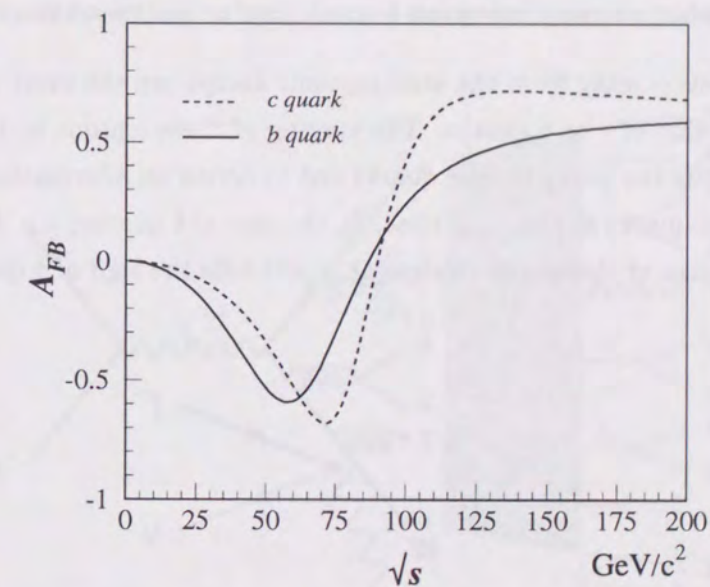
Figure 1.2: Forward-backward asymmetry of c and b quarks.
