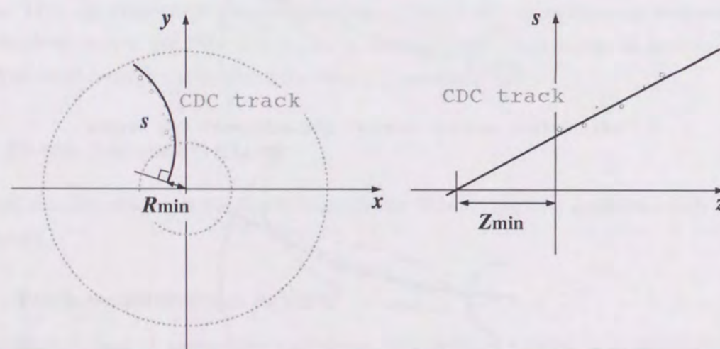
Figure 3.2: Definition of track parameters: (a) R_{\min} and (b) Z_{\min} . Both figures show in the case of negative values.
