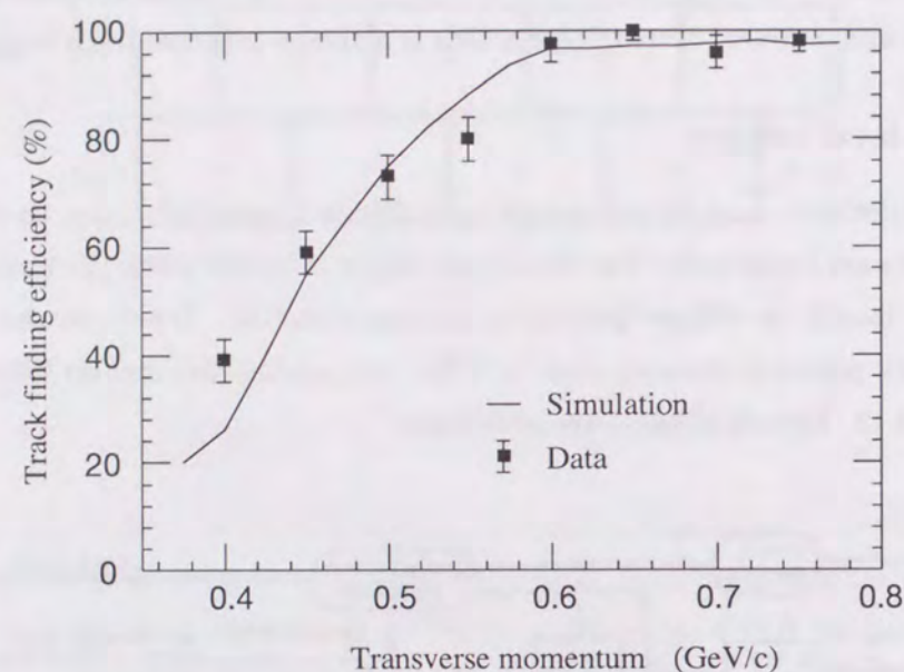
Figure 2.13: Trigger efficiency of the track finder
