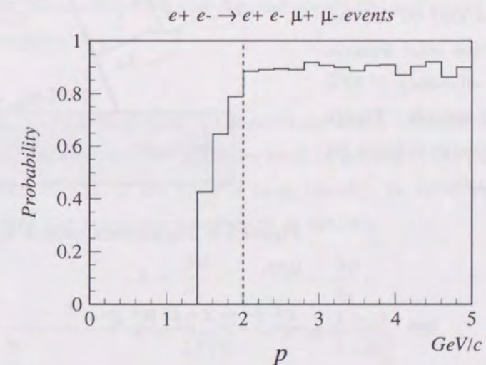
Figure 5.3: Probability that the hits are found in more than 4 layers as a function of muon momentum.
