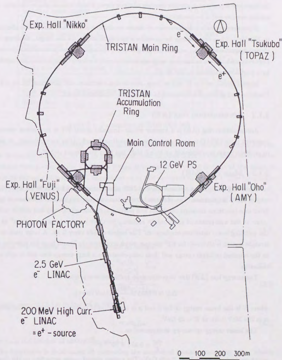
Figure 2.1: Layout of TRISTAN
