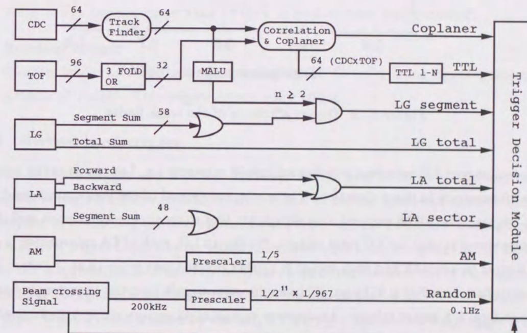
Figure 2.12: Trigger logic
