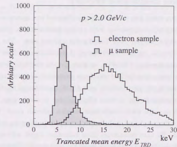
Figure 4.3: Truncated mean energy of TRD for electrons and muons
