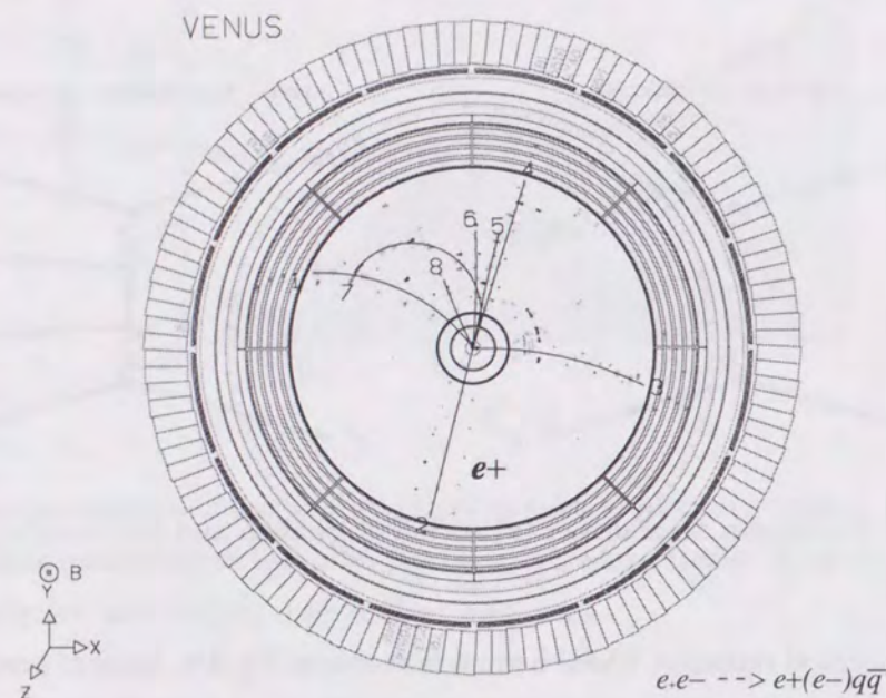
Figure 3.9: Electron inclusive event in two-photon process
