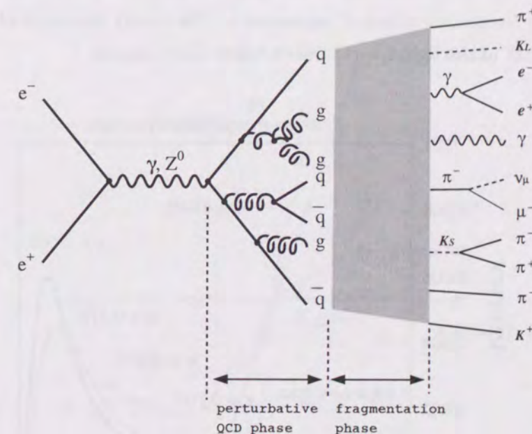
Figure 1.4: QCD processes
