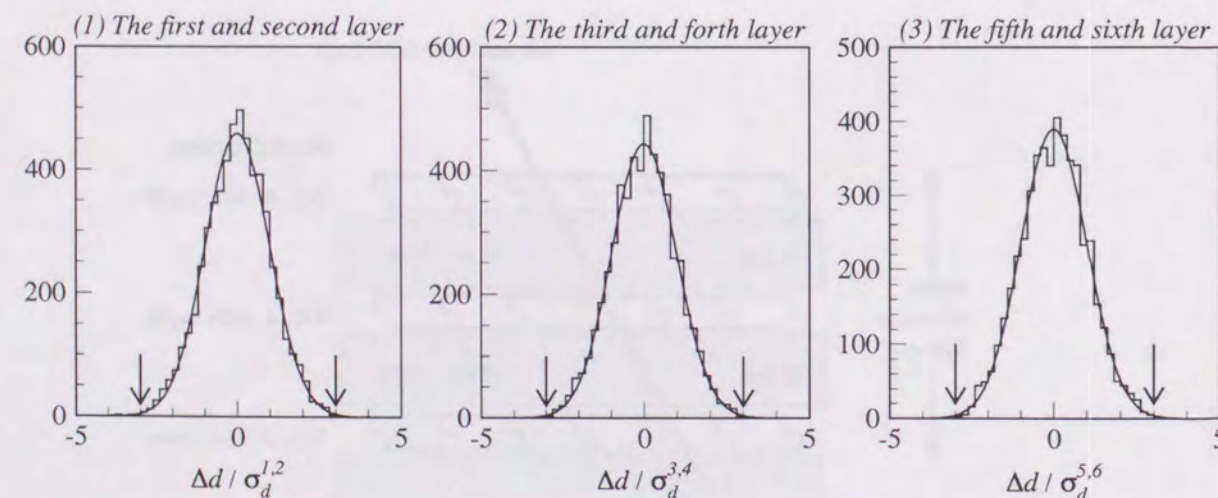
Figure 5.2: Normalized distance ( \Delta d/\sigma_d ) distributions for isolated muon sample, where \Delta d is the distance between the chamber hit position and that extrapolated from CDC, and \sigma_d^i is calculated from multiple Coulomb scattering.
