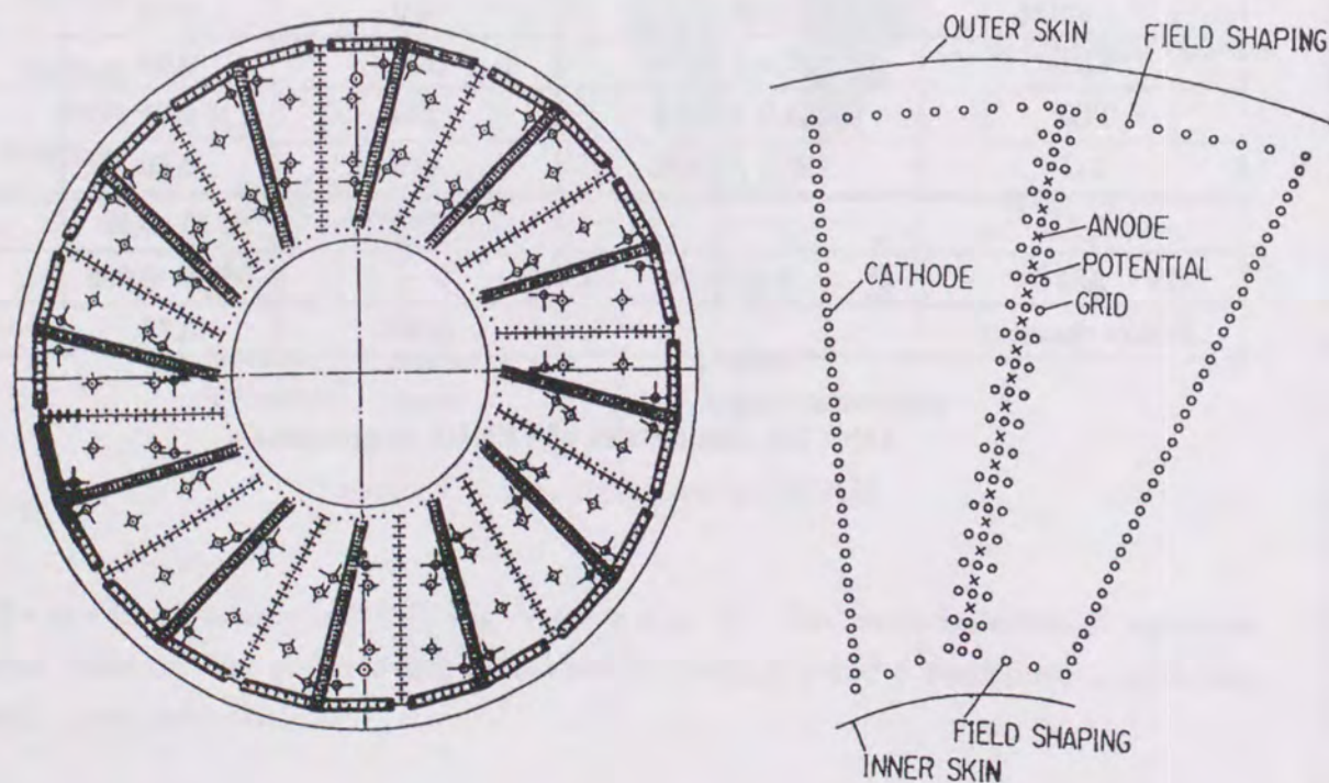
Figure 2.4: Schematic view of VTX
