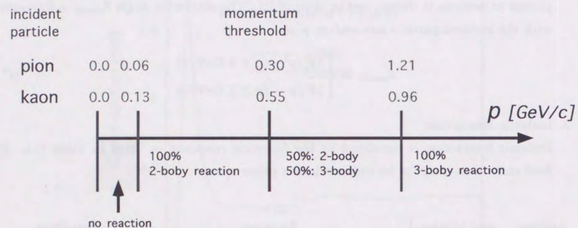
Figure C.7: Momentum threshold of inelastic reactions for pion and kaon.
