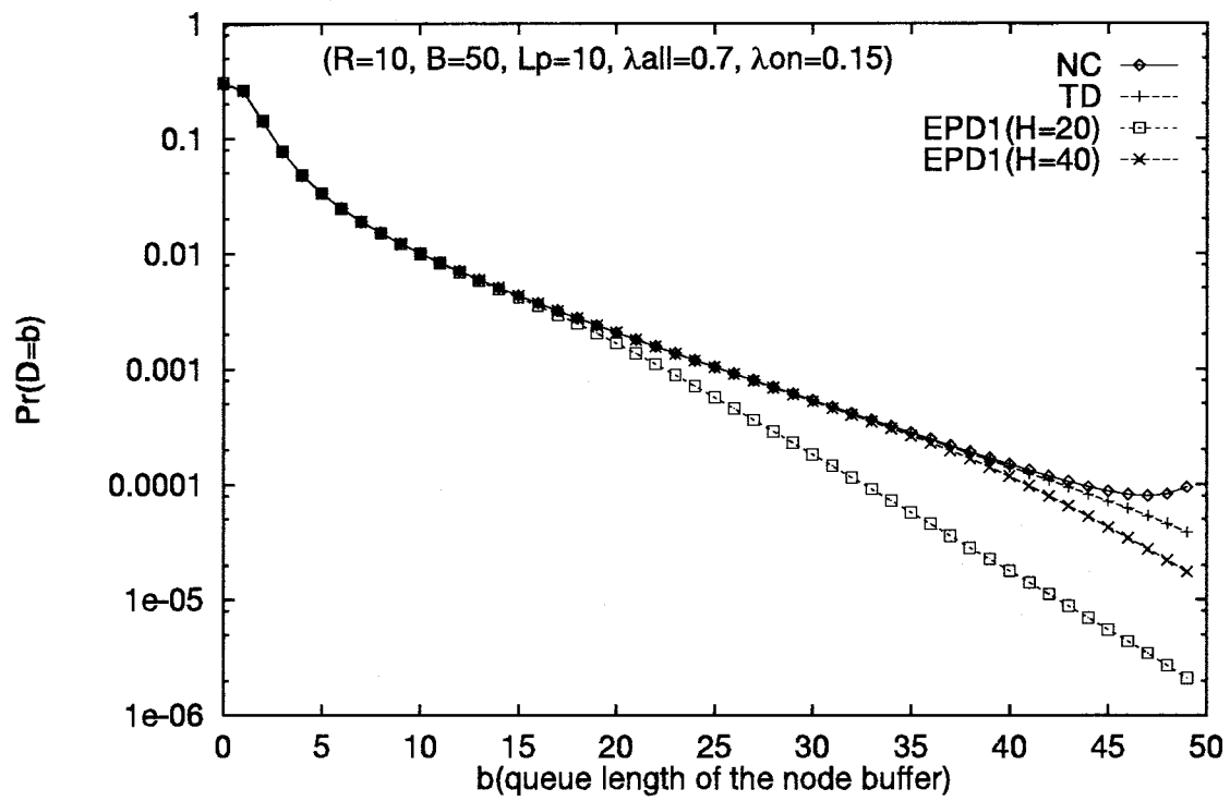
Figure 4.11: Distribution of the queue length: cases of H_b = 20 and 40
