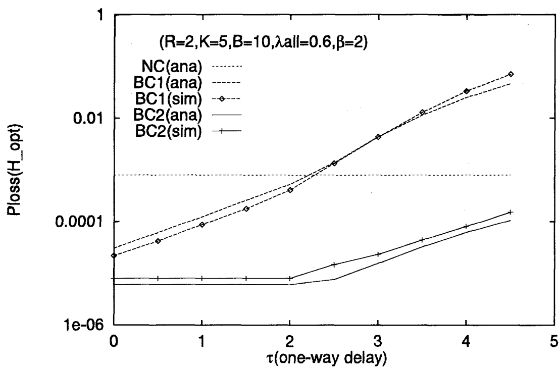
Figure 2.5: Cell loss probability as a function of \tau : comparison between analysis and simulation
