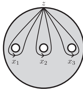
Fig.2. The punctured disk D_3 .
