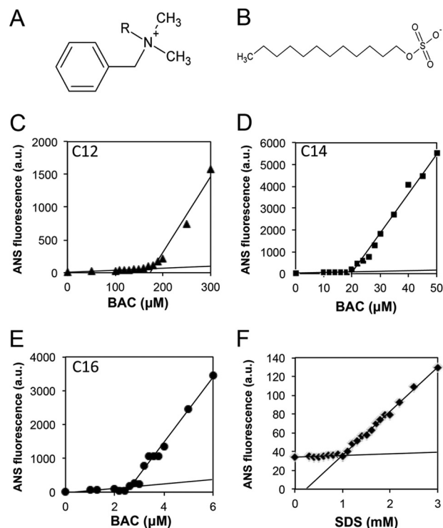
FIGURE 2. Molecular structures and CMCs of BAC and SDS. A and B, chemical structures of BAC (A) and SDS (B). C–F, determination of CMCs for BAC( \text{C}_{12} ) (C), \text{C}_{14} (D), and \text{C}_{16} (E) and SDS (F) using ANS fluorescence. The CMC values of BAC and SDS were determined to be 0.15 mM (BAC( \text{C}_{12} )) (C), 0.02 mM (BAC( \text{C}_{14} )) (D), 0.0025 mM (BAC( \text{C}_{16} )) (E), and 1 mM (SDS (F)), respectively.
