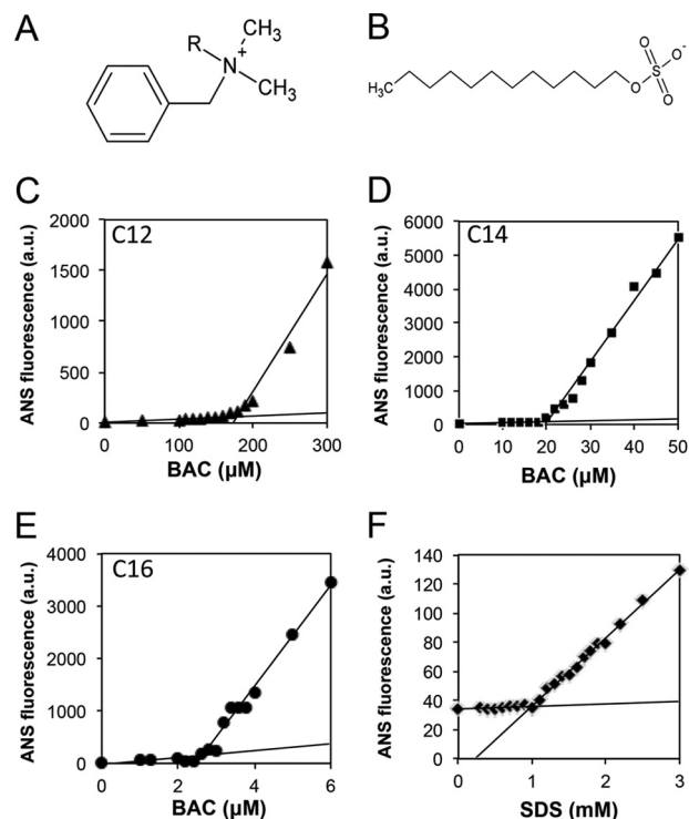
FIGURE 2. Molecular structures and CMCs of BAC and SDS. A and B, chemical structures of BAC (A) and SDS (B). C–F, determination of CMCs for BAC(C 12 ) (C), C 14 (D), and C 16 (E) and SDS (F) using ANS fluorescence. The CMC values of BAC and SDS were determined to be 0.15 mM (BAC(C 12 )) (C), 0.02 mM (BAC(C 14 )) (D), 0.0025 mM (BAC(C 16 )) (E), and 1 mM (SDS (F)), respectively.
