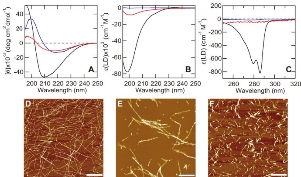
FIGURE 4. Comparison of the flow-induced LD spectra of different fibrils. Shown are far-UV CD ( A ), far-UV LD ( B ), and near-UV LD ( C ). Fibrils studied are mature \beta 2-m fibrils (red), f218 fibrils (blue), and f210 fibrils (black). Shown also are atomic force microscopy images of f210 ( D ), \beta 2-m ( E ), and f218 ( F ) fibrils. The scale bars in D–F represent 1 \mu m.
