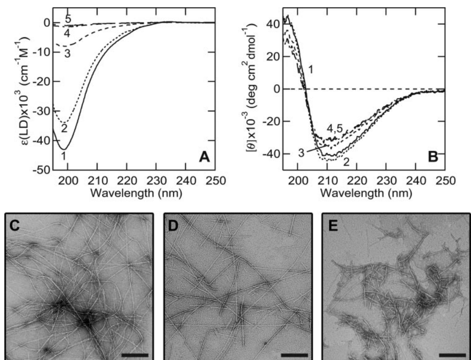
FIGURE 3. Dependence of LD on the length of f210 fibrils. The number of ultrasonication pulses applied was 0 (trace 1), 1 (trace 2), 10 (trace 3), 20 (trace 4), and 30 (trace 5). A , far-UV LD spectra under vertical flow. B , far-UV CD spectra without flow. Shown also are electron microscopy images of f210 fibrils without ultrasonication ( C ), after 10 pulses ( D ), and after 30 pulses ( E ) of ultrasonication. The scale bars in C–E represent 200 nm.
