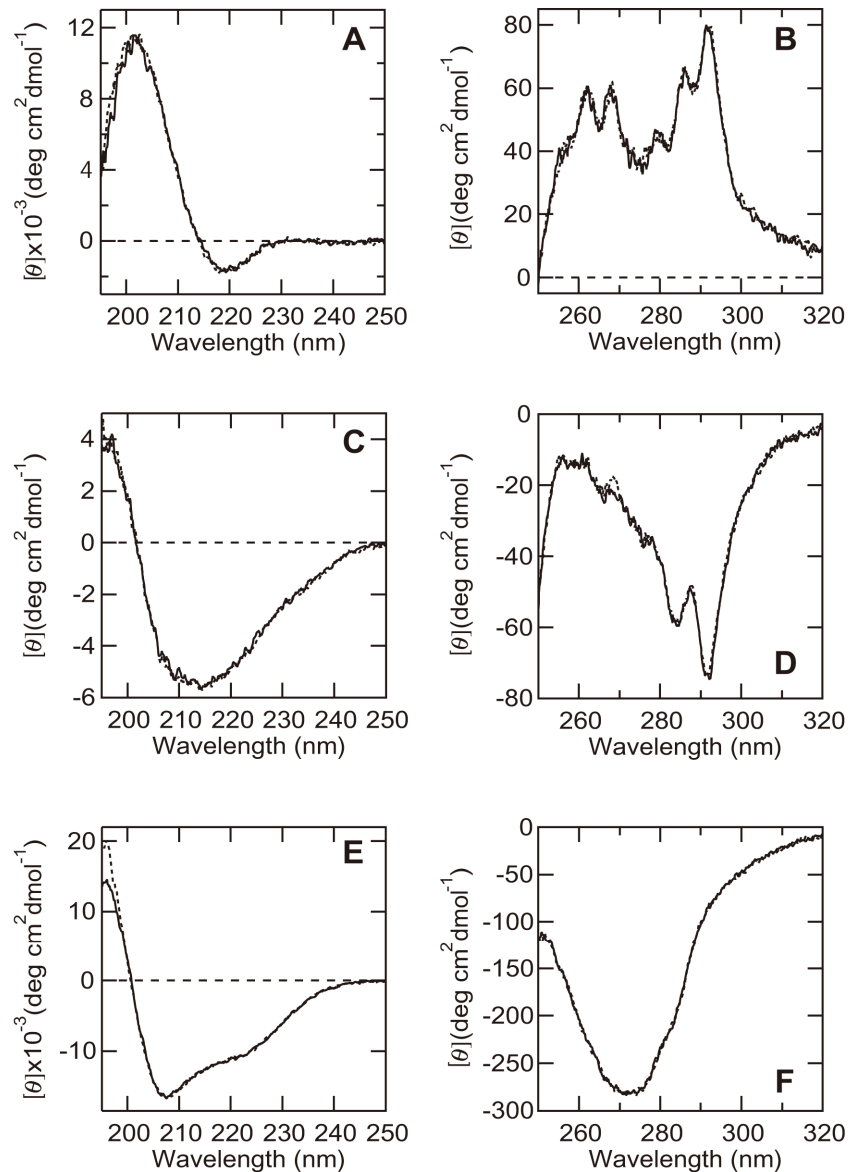
SUPPLEMENTAL FIGURE 1. The flow-induced CD spectra of the native monomeric proteins. \beta 2-m (A, B) at pH 7.0, bovine \beta -lactoglobulin (C, D) at pH 7.0, and bovine insulin (E, F) at pH 2.0. Far-UV (A, C, E) and near-UV (B, D, F) CD spectra were measured under vertical flow (solid line) or without flow (dotted line), revealing no flow-induced CD for the native states.
