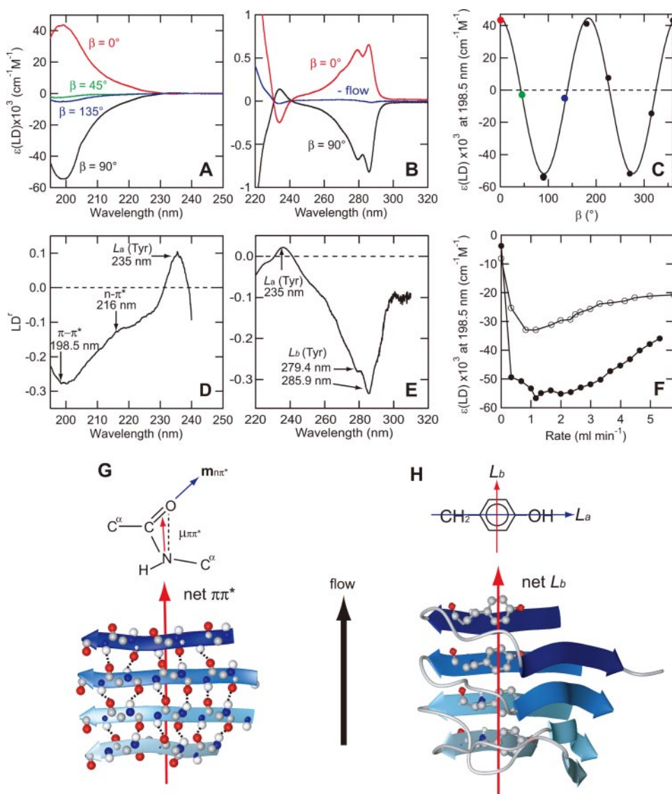
FIGURE 2. The flow-induced LD spectra of f210 fibrils. A and B, dependence of flow-induced LD on the direction of flow. A, far-UV LD spectra at various angles of the flow cell ( \beta = 0^\circ , 45^\circ , 90^\circ (vertical), and 135^\circ ). B, near-UV LD spectra at \beta = 0^\circ , \beta = 90^\circ , and without flow. C, dependence of \epsilon(\text{LD}) at 198.5 nm on \beta . Solid circles are observed values, of which four points between 0 and 135^\circ correspond to the spectra with the same color in A. LD' spectra in the far-UV (D) and near-UV (E) regions, which were obtained by \epsilon(\text{LD})/\epsilon(\text{UV}) . F, dependence of \epsilon(\text{LD}) at 198.5 nm on the flow rate at \beta = 90^\circ . The results for the two fibril preparations are shown. G, electric dipole transition moment of the amide \pi\pi^* transition ( \mu_{\pi\pi^*} ), the magnetic dipole transition moment of the amide n\pi^* transition ( m_{n\pi^*} ), and three-dimensional structural model of f210 fibrils representing an ordered backbone with net \pi\pi^* transition moments parallel to the fibril axis. H, the transition moments of tyrosine chromophores and three-dimensional structural model representing ordered Tyr 26 side chains. The Tyr side chain has two transition moments; one is L_a with \epsilon_{\text{max}} = \sim 10^4 \text{ M}^{-1} \text{ cm}^{-1} near 230 nm, and the other is L_b with \epsilon_{\text{max}} = \sim 1,400 \text{ M}^{-1} \text{ cm}^{-1} at \sim 280 \text{ nm} . The LD' spectrum suggests that the L_b transition moment of Tyr 26 contributes most to the observed LD'.
