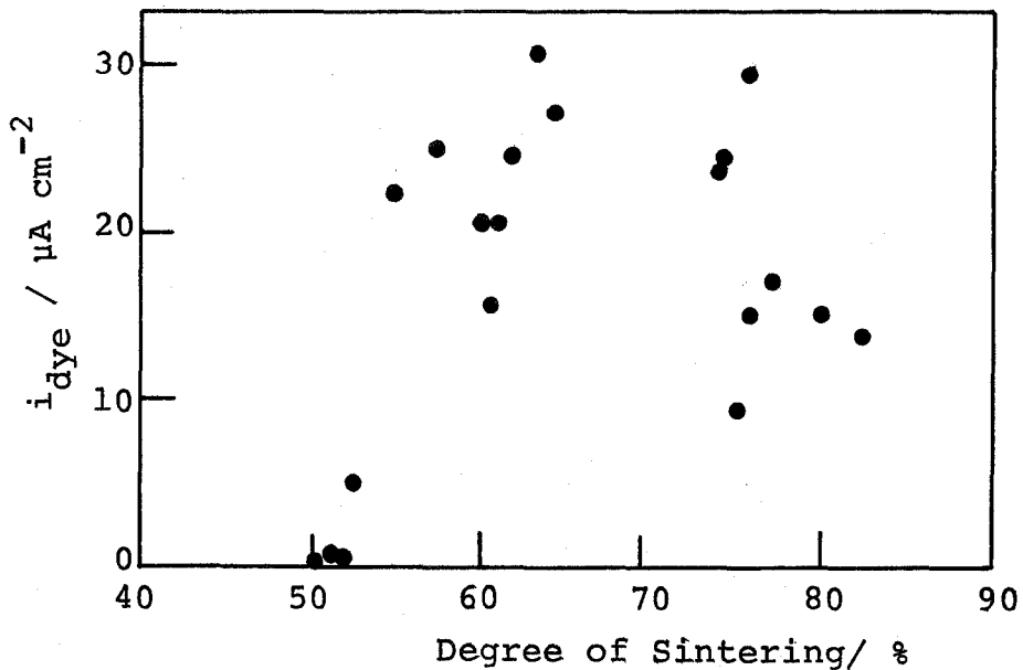
Fig. 9. Dye-sensitized photocurrent against the degree of sintering of the ZnO electrodes doped with 0.5 mol% Al 2 O 3 .
