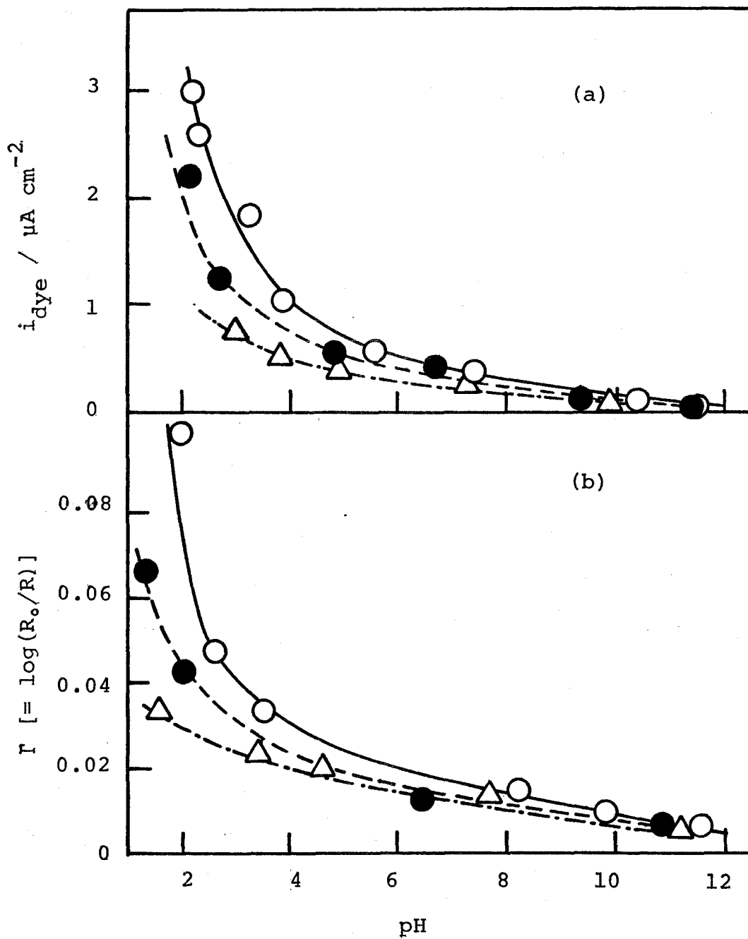
Fig. 13. The effect of alkali halides on the photocurrent sensitized by rhodamine B (a), and the adsorption of the dye on the ZnO sinter (b): rhodamine B, 2 \times 10^{-5} M; ○, 1M KI; ●, 1 M KBr; △, 1 M KCl.
