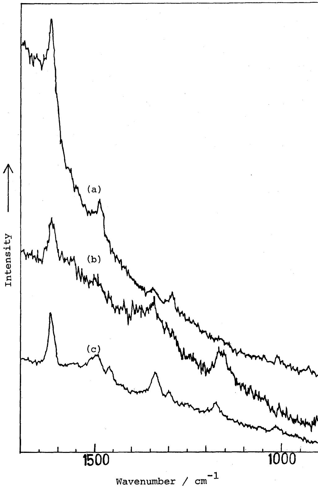
Fig. 6. Resonance Raman spectra of rose bengal: (a) aqueous solution of the dye, (b) the dye adsorbed on the ZnO sinter, (c) zinc salt of the dye.
