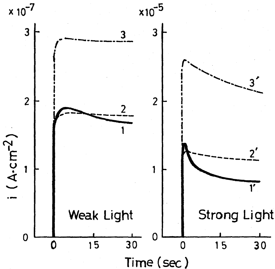
Fig. 5 The change of photocurrents with time for \langle \text{ZnO} | \text{rose bengal} - \text{reducing agent} | \text{Pt} \rangle . 1, Without any reducing agent; 2, with TMPD ( 6 \times 10^{-4} mol/l); 3, with hydroquinone ( 6 \times 10^{-4} mol/l). Rose bengal, 2.7 \times 10^{-5} mol/l; \text{Na}_2\text{SO}_4 , 0.2 mol/l; electrode potential, 0.2 V (vs SCE).
