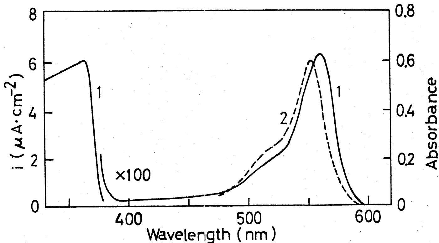
Fig. 2 Curve (1) is the photocurrent action spectrum of \langle \text{ZnO} | \text{rose bengal} | \text{Pt} \rangle in a solution of 2.4 \times 10^{-6} mol/l rose bengal and 0.2 mol/l \text{Na}_2\text{SO}_4 at an anodic bias of 0.5 V (vs. SCE), for the illumination by 4.7 \times 10^{14} photons/cm 2 s. Curve (2) is the absorption spectrum of the dye obtained from 6 \times 10^{-6} mol/l aqueous solution.
