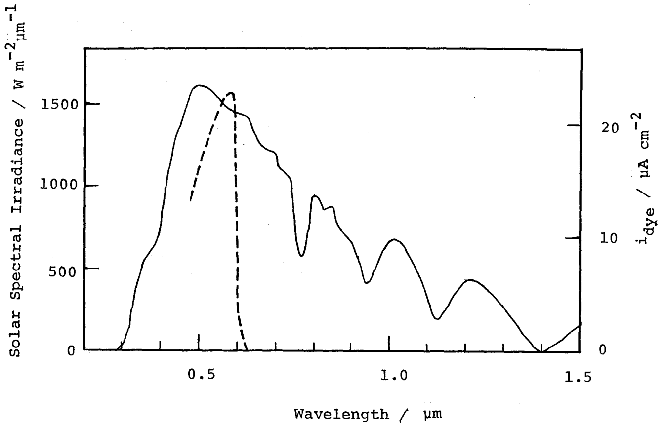
Fig. 10. The action spectrum of the photocurrent sensitized by rose bengal at the porous ZnO electrode (----), and the AM 1 solar spectrum (—). The solar energy in the wavelength region above 1.5 μm is less than 10 % of the total.
