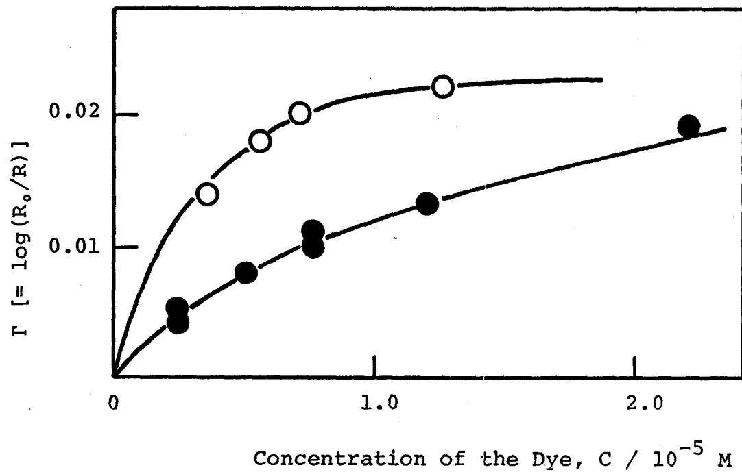
Fig. 1. Adsorption of dyes from the aqueous neutral solutions containing 0.1 M \text{KNO}_3 on the ZnO sinter at 22 °C: \circ , rose bengal; \bullet , phloxine B. The ordinate indicates the absorbance of the adsorbed dyes obtained from the diffuse reflectance spectra of the ZnO sinter at the wavelengths of 562 nm(rose bengal) and 551 nm (phloxine B).
