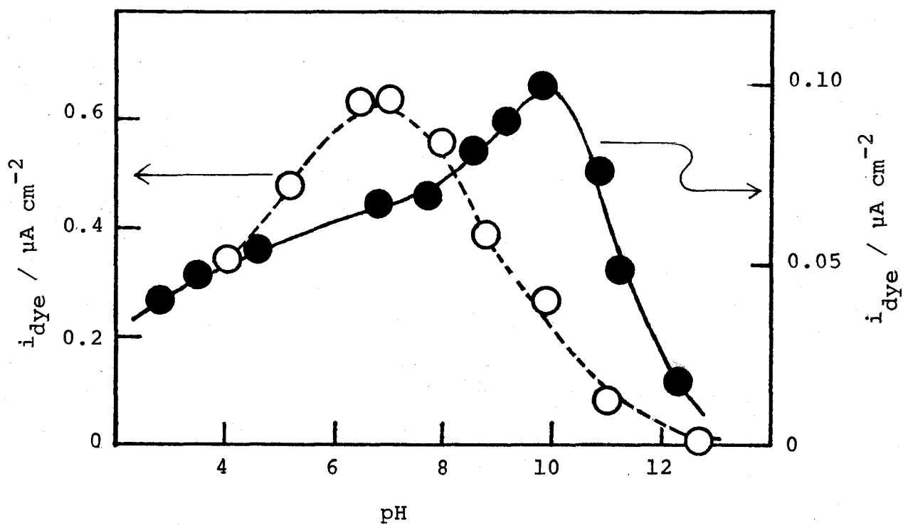
Fig. 12. The pH-dependence of the dye-sensitized photocurrent at the ZnO electrode: \circ , rhodamine B ( 1.6 \times 10^{-5} M, \lambda 556 nm); \bullet , rhodamine 6G ( 1.5 \times 10^{-5} M, \lambda 540 nm); \text{KNO}_3 , 0.1 M; U, 0.5 V vs SCE.
