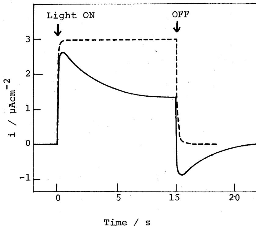
Fig. 2. The change of the short-circuit photocurrent of the dye-sensitized photocell vs. time: rose bengal, 2 \times 10^{-6} M; KI, 0.1 M; I_2 , 0 M (—) and 10^{-4} M (----).
