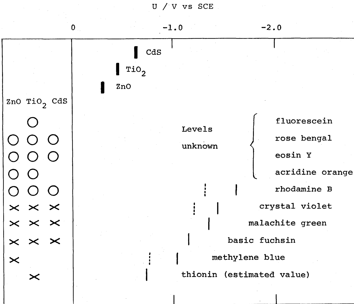
Fig. 4 The correlation between the energy levels of the semiconductors and dyes, and the presence (○) and absence ( x ) of the dye-sensitized photocurrent. █ Conduction band of the semiconductor. — Singlet excited state of the dye. ---- Triplet excited state of the dye.
