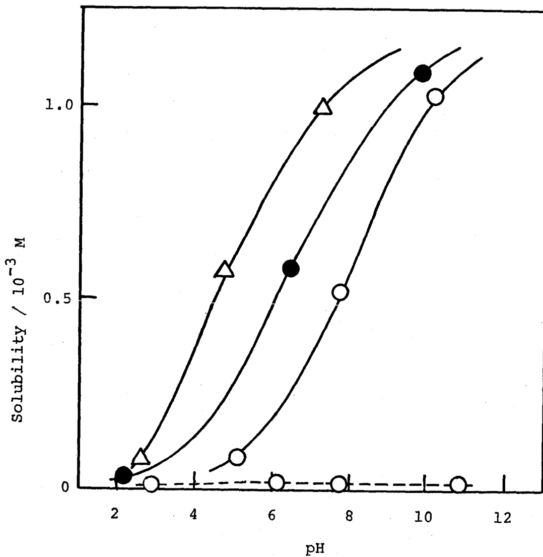
Fig. 14. The pH-dependence of the solubility of rhodamine B (—) and rhodamine 6G (-----) in the aqueous solution containing alkali halides: \circ , 1 M KI; \bullet , 1 M KBr; \triangle , 1 M KCl
