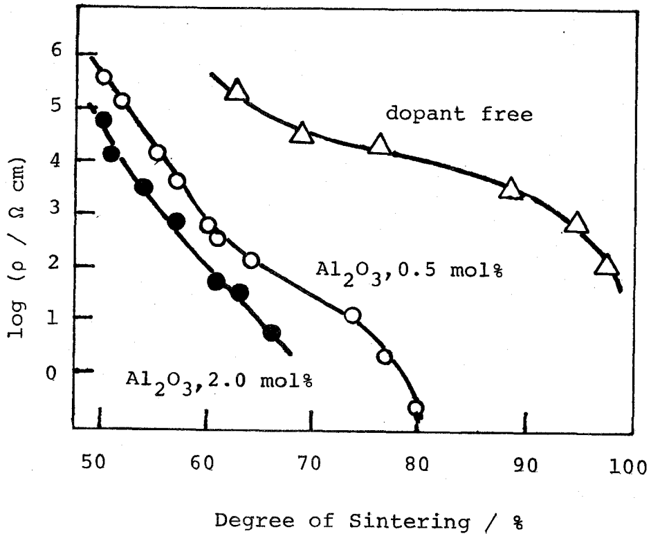
Fig. 8. Resistivity of the ZnO sinter against the degree of sintering; \Delta dopant free, \circ doped with 0.5 mol% Al 2 O 3 , \bullet doped with 2.0 mol% Al 2 O 3 .
