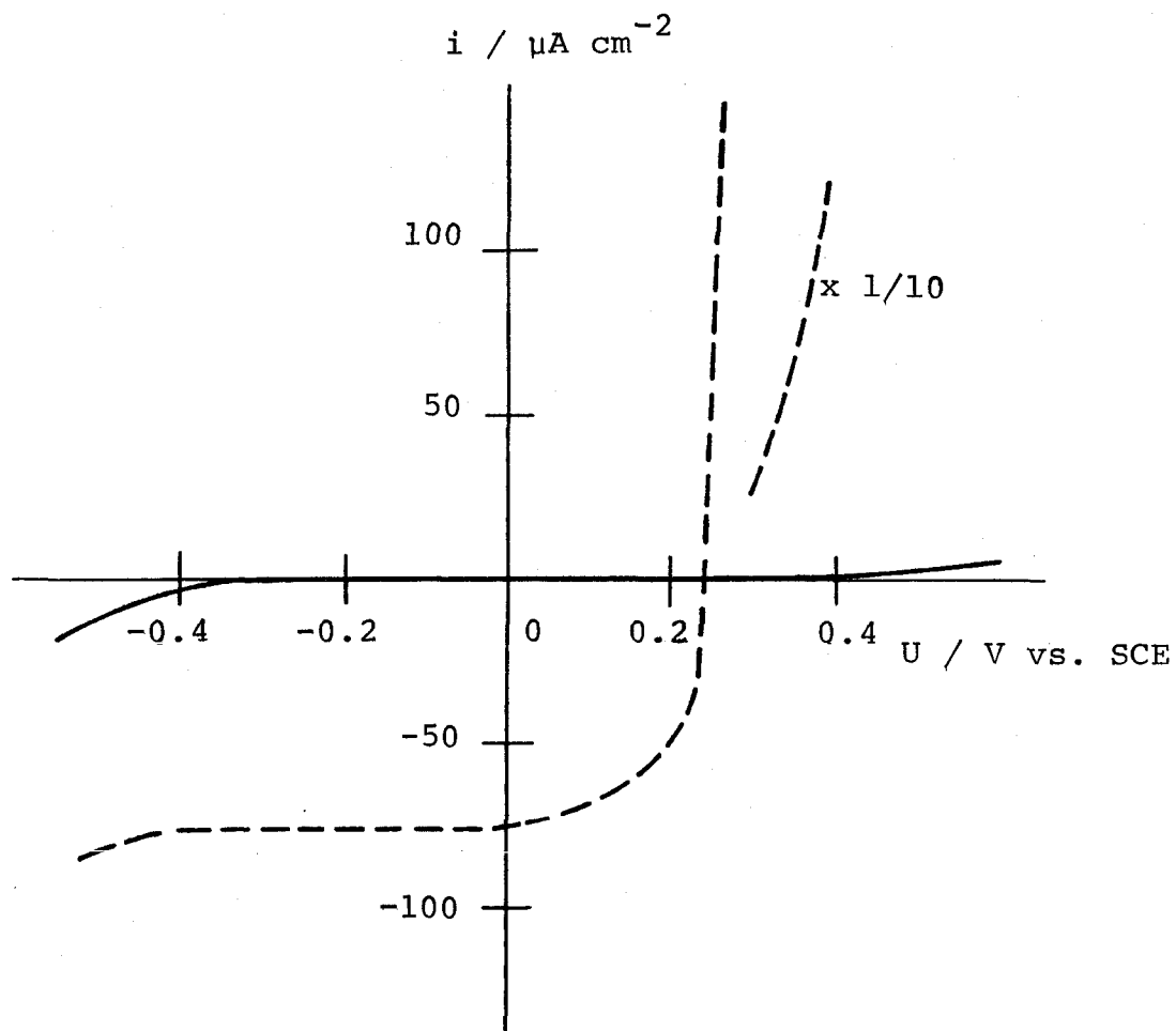
Fig. 4. Current-potential curves of a platinum electrode in aqueous solutions; —, 0.2 M \text{Na}_2\text{SO}_4 ; ----, 0.1 M \text{KI} + 3 \times 10^{-4} M \text{I}_2 .
