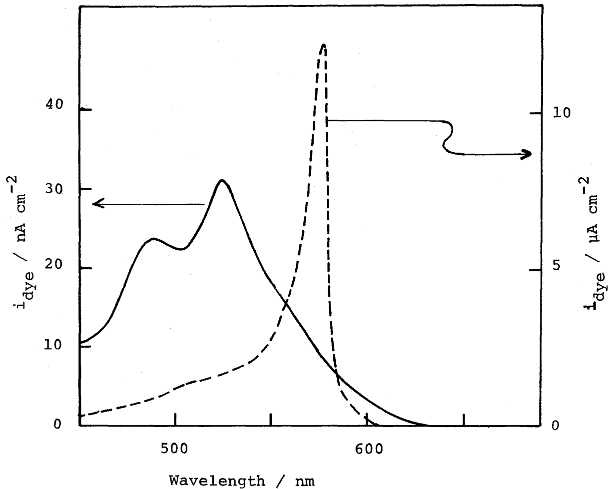
Fig. 17. Action spectra of the photocurrents at the ZnO electrode sensitized by 1,1'-diethyl-2,2'-cyanine ( 3 \times 10^{-5} M): U, 0.5 V vs SCE; —, 0.02 M \text{KNO}_3 ; ----, 0.5 M KBr.
