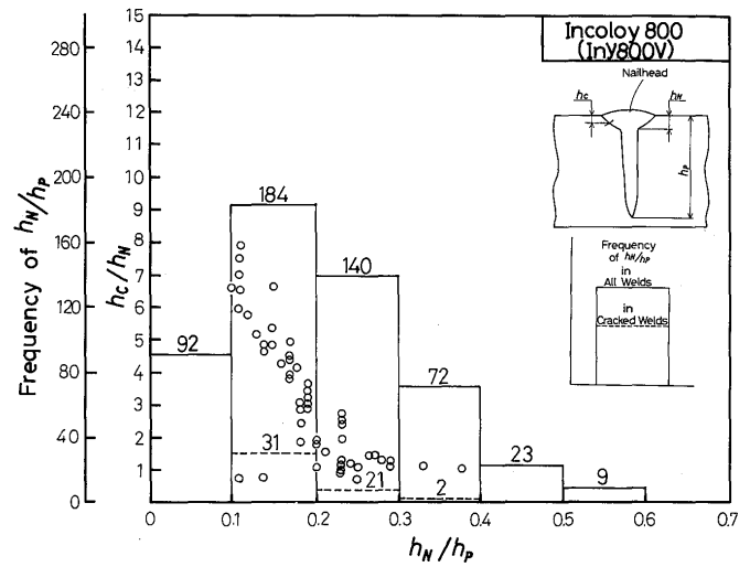
Fig. 12 Effect of h_N/h_P and h_c/h_N on Microcrack
