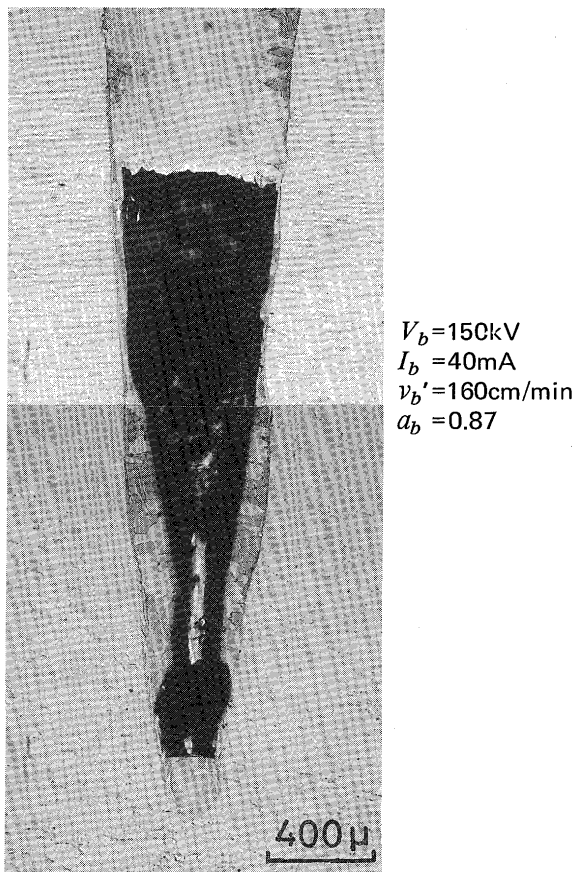
Photo. 1 Typical R-porosity (SUS 316)
