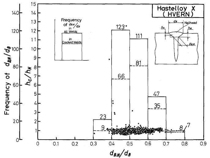
Fig. 13 Effect of d_{B,N}/d_B and h_c/h_N on Microcrack
