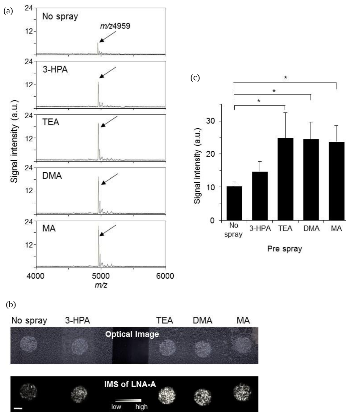
Figure 12. Improvement of detection sensitivity of LNA-A by addition of amines to 3-HPA solution. (a) Typical mass spectra of kidney homogenate sections applying each additive. (b) Typical images of kidney homogenate sections (optical image) and IMS of LNA-A by extracting m/z 4959. (c) Bar diagram of signal intensity of LNA-A for the comparison of additives effect. No spray represents normal method (ImagePrep only). Pre-sprayed 3-HPA, TEA, DMA, and MA with an airbrush. All error bars derive from four times measurements for each method. Data represent mean values \pm SD. * p < 0.05 , a.u. arbitrary unit. Scale bar: 2.5 mm.
