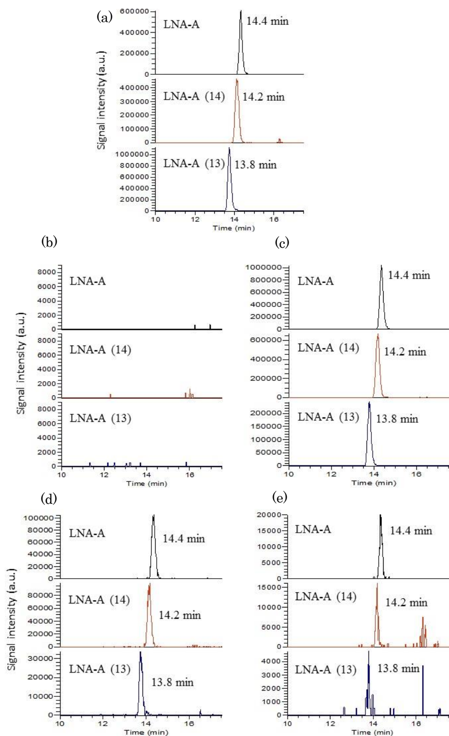
Figure 6. Measurement of mouse plasma after intravenous injection of LNA-A. Extracted ion chromatogram of LNA-A, LNA-A (14), and LNA-A (13) spiked mouse plasma (a), control mouse plasma (b), LNA-A dosed mouse plasma after 0.5 h (c), 2 h (d), and 4 h (e). a.u. arbitrary unit.
