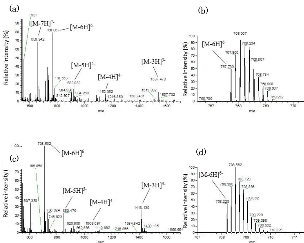
Figure 4. ESI-mass spectra of LNA-A (14) in mouse plasma of the mass range of m/z 540-1700 (a) and expanding mass range of its [M-6H]^6 group (b). ESI-mass spectra of LNA-A (13) in mouse plasma of the mass range of m/z 540-1700 (c) and expanding mass range of its [M-6H]^6 group (d).
