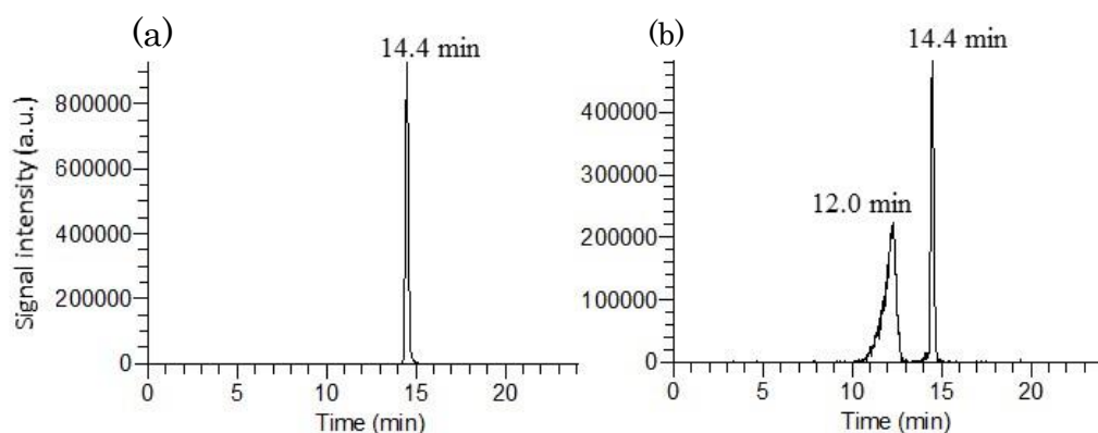
Figure 2. Detection of LNA-A in purified water or mouse plasma after Phe-Chl extraction. Extracted ion ( m/z 825.239) chromatograms of LNA-A in water (a) and mouse plasma (b) by ion-pair LC-MS assay. a.u. arbitrary unit.
