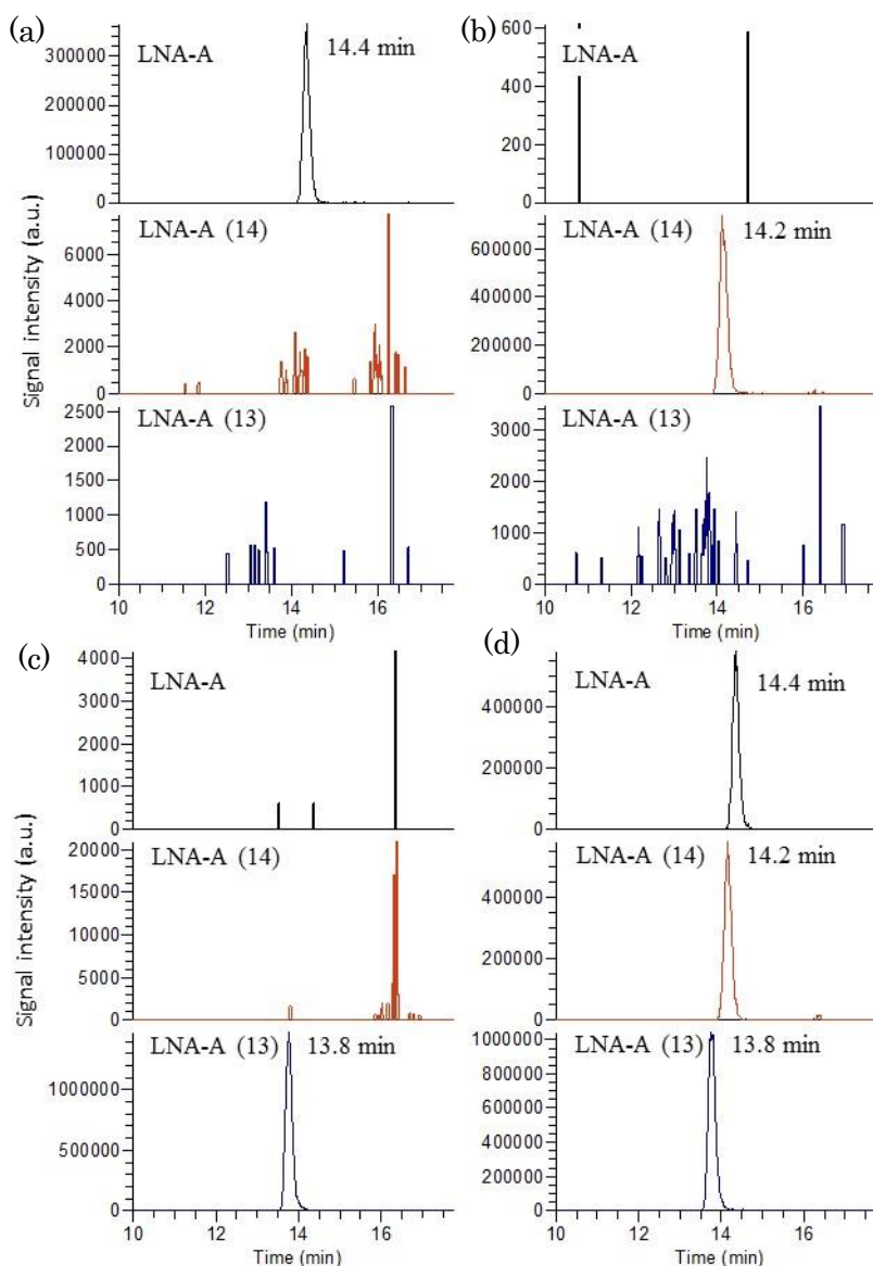
Figure 5. Detection of LNA-A, LNA-A (14), and LNA-A (13) in mouse plasma with LNA-A ( m/z 825.239), LNA-A (14) ( m/z 825.239), and LNA-A (13) ( m/z 708.228) added alone or mixed. LNA-A spiked mouse plasma (a), LNA-A (14) spiked mouse plasma (b), LNA-A (13) spiked mouse plasma (c), and all spiked mouse plasma (d). a.u. arbitrary unit.
