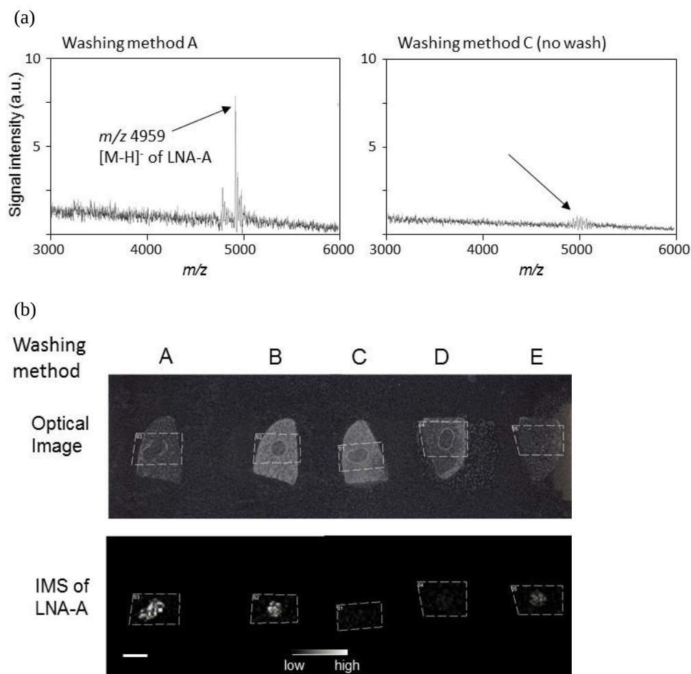
Figure 8. Relationship between washing methods and detection sensitivity of LNA-A on liver section. Applied washing methods A-E are indicated in Table 3. (a) Typical mass spectra of liver sections applied washing method A and method C (no wash). (b) Images of liver sections with LNA-A on the surface (optical image) and IMS of LNA-A by extracting m/z 4959. The part surrounded by the white broken line is the measurement site. a.u. arbitrary unit. Scale bar: 2.5 mm.
