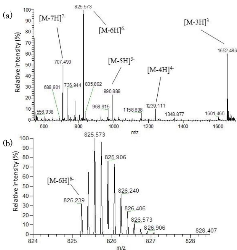
Figure 1. ESI-mass spectra of LNA-A in purified water of the mass range m/z 540-1700 (a) and expanding mass range of its [M-6H]^{6-} group (b).
