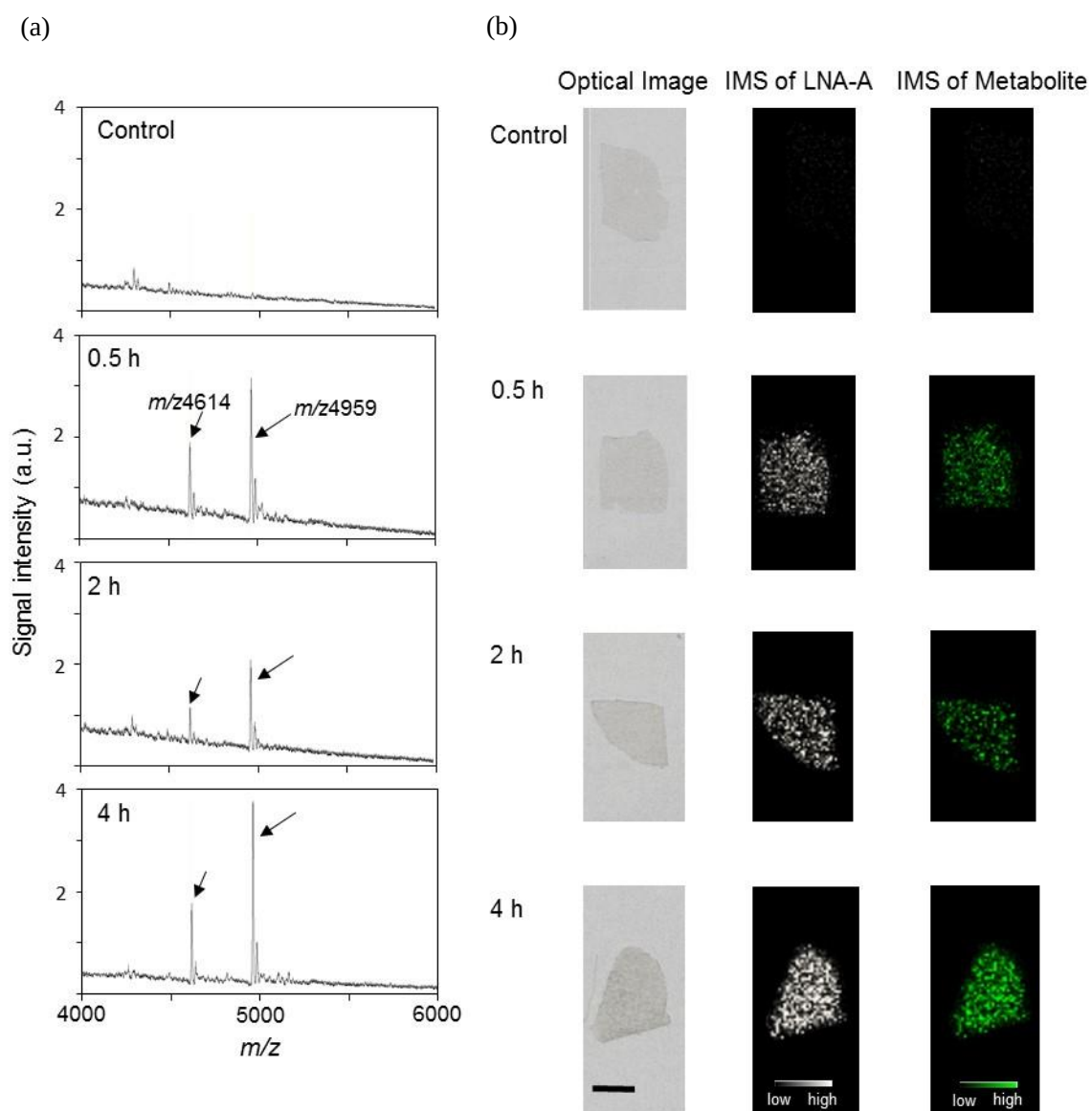
Figure 14. Measurement of mouse liver section after administration of LNA-A. (a) Typical mass spectra of control liver section and 0.5, 2, and 4 h post-dose liver sections. (b) Images of mouse liver section (optical image) and IMS of LNA-A (extracting m/z 4959) and its metabolite (extracting m/z 4614). a.u. arbitrary unit. Scale bar: 5 mm.
