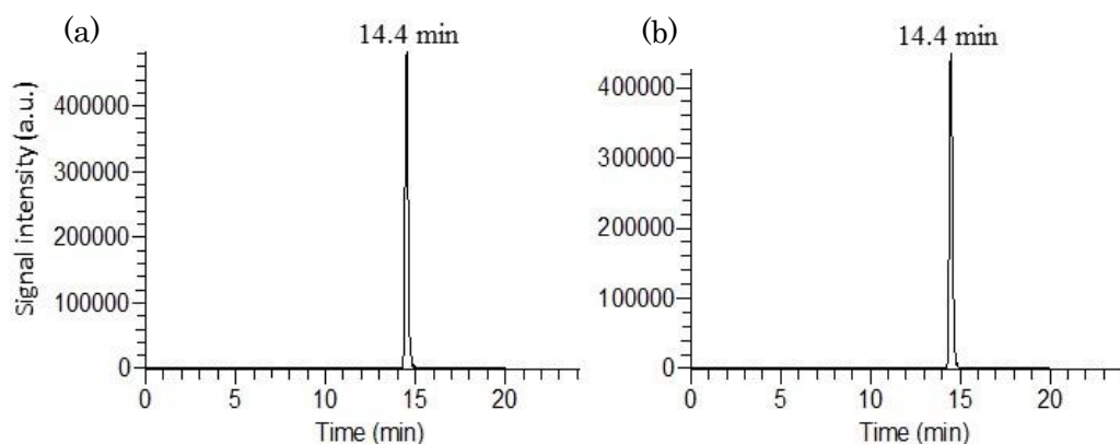
Figure 3. Detection of LNA-A in purified water or mouse plasma after two step extraction. Extracted ion ( m/z 825.239) chromatogram of LNA-A in water (a) and mouse plasma (b) after two step extraction by ion-pair LC-MS assay. a.u. arbitrary unit.
