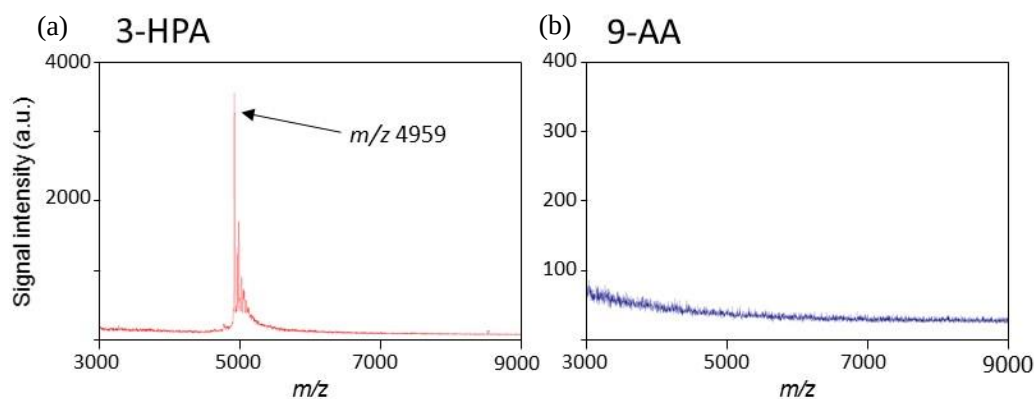
Figure 7. MALDI mass spectra of LNA-A using 3-HPA (a) or 9-AA (b) as matrix. a.u. arbitrary unit.
