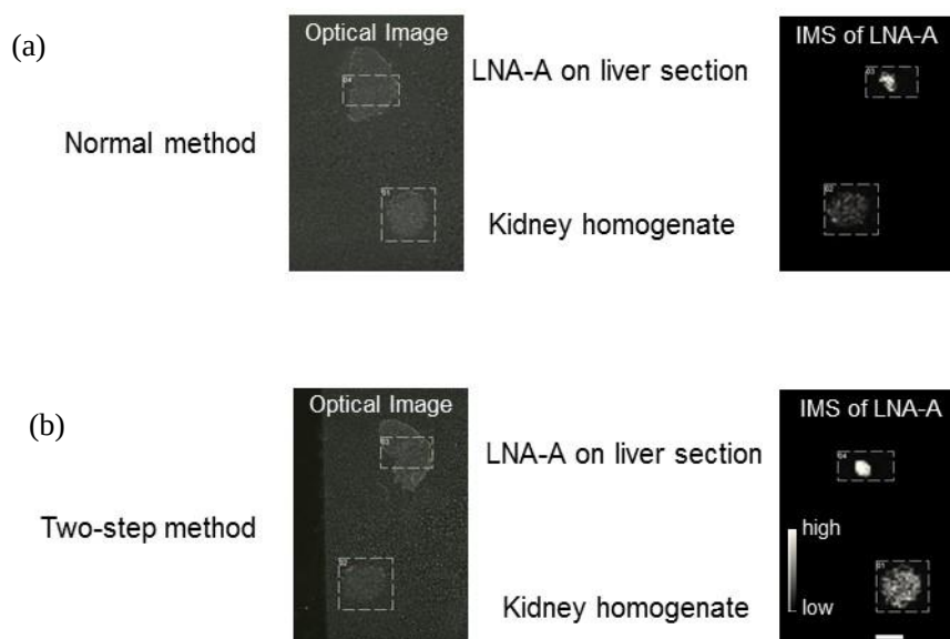
Figure 11. Improvement of detection sensitivity of LNA-A by two-step method developed in this study. Images of liver section and kidney homogenate sections (optical image) and IMS of LNA-A by extracting m/z 4959 applying normal method (a) and two-step method (b). The part surrounded by the white broken line is the measurement site. a.u. arbitrary unit. Scale bar: 2.5 mm.
