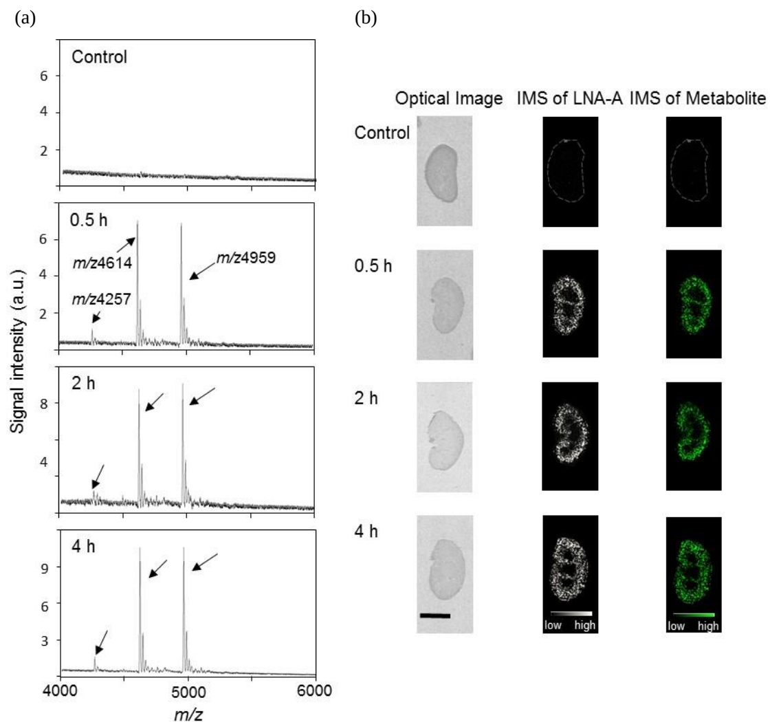
Figure 15. Measurement of mouse kidney section after administration of LNA-A. (a) Typical mass spectra of control kidney section and 0.5, 2, and 4 h post-dose kidney sections. (b) Images of mouse kidney section (optical image) and IMS of LNA-A (extracting m/z 4959) and its metabolite (extracting m/z 4614). a.u. arbitrary unit. Scale bar: 5 mm.
