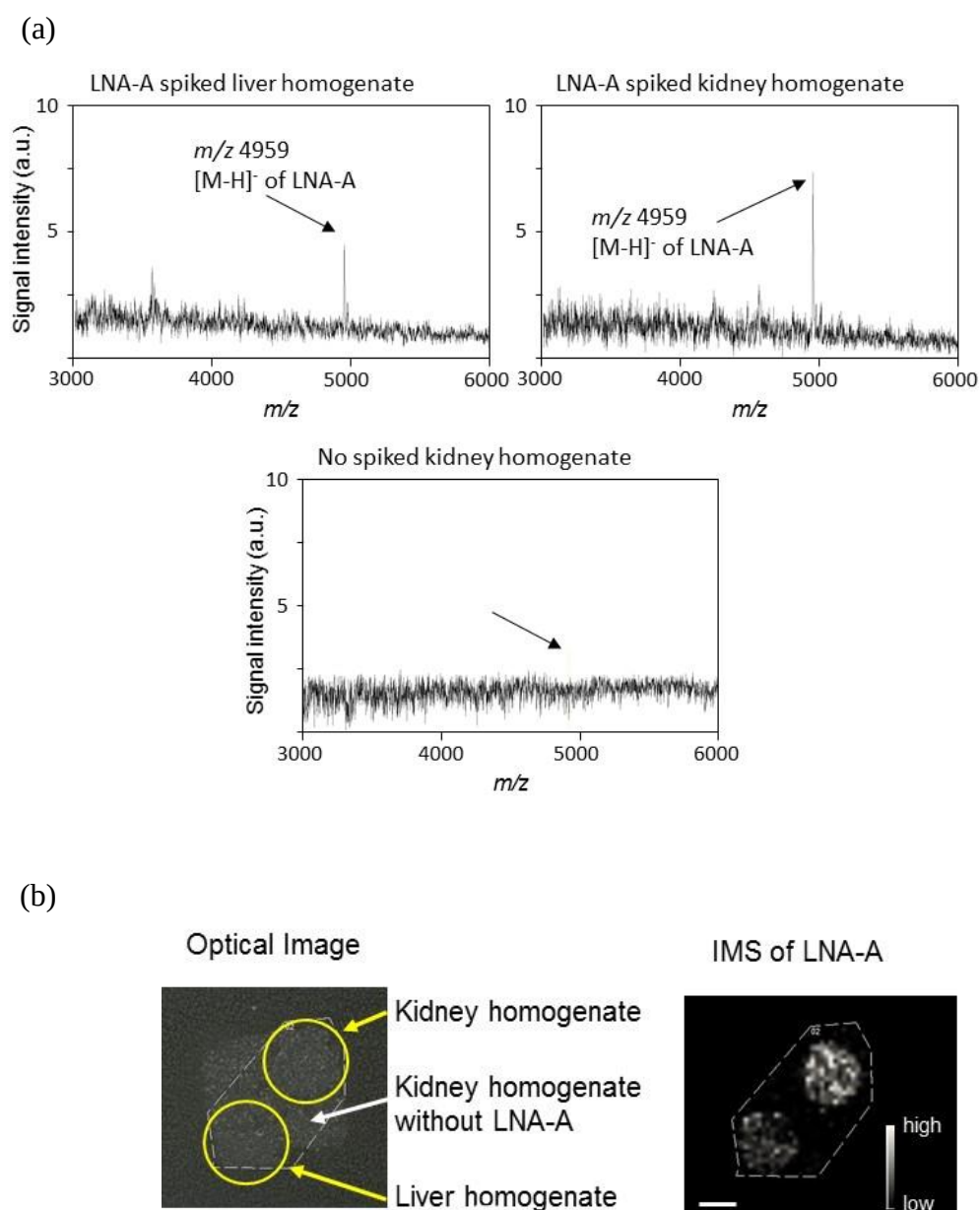
Figure 10. Comparison of LNA-A detection in kidney homogenate section and liver homogenate section. (a) Typical mass spectra of LNA-A spiked liver and kidney homogenate section and kidney homogenate section without LNA-A. (b) Images of frozen homogenate sections (optical image) and IMS of LNA-A by extracting m/z 4959. The part surrounded by the white broken line is the measurement site. a.u. arbitrary unit. Scale bar: 2.5 mm.
