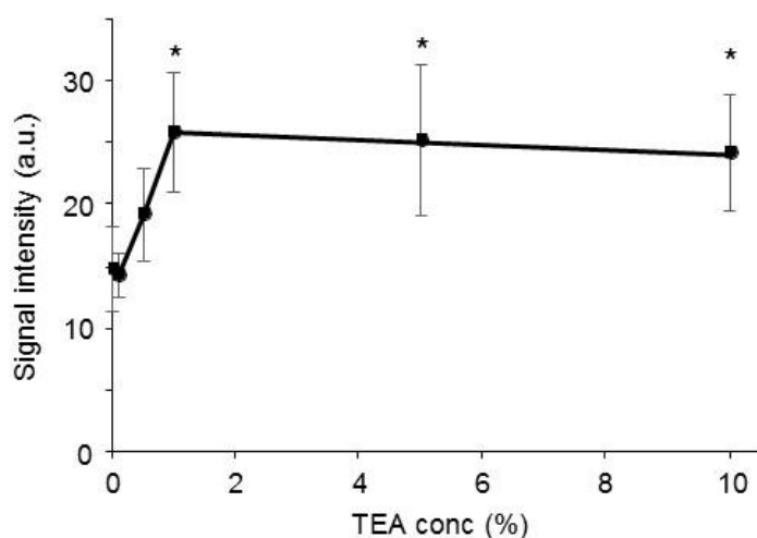
Figure 13. Signal intensity profiles of LNA-A dependent on TEA concentrations in matrix solution. All error bars derive from four times measurements for each concentration. Data represent mean values \pm SD. * p < 0.05 , a.u. arbitrary unit.
