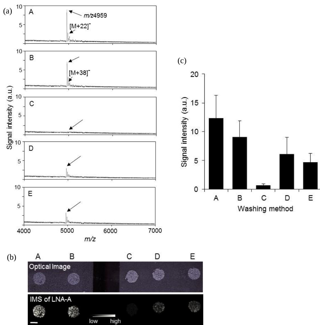
Figure 9. Relationship between washing methods and detection sensitivity of LNA-A in kidney homogenate section. Applied washing methods A-E are indicated in Table 3. (a) Typical mass spectra of homogenate sections applying each washing method. (b) Typical images of homogenate sections (optical image) and IMS of LNA-A by extracting m/z 4959. (c) Bar diagram of signal intensity of LNA-A for the five applied washing methods. All error bars derive from four times measurements for each washing method. Data represent mean values \pm SD. a.u. arbitrary unit. Scale bar: 2.5 mm.
