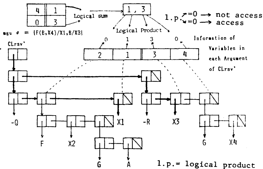
Information of Variables in ngu
