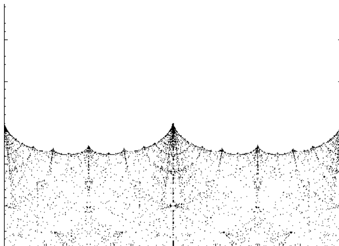
Fig. 1. The Maskit embedding in \mathbb{C} . Figure courtesy of David Wright.
