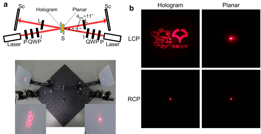
Figure 4. Reconstruction of the double-sided hologram. (a) Schematic image and picture of experimental setup. P: Polarizer; QWP: Quarter wave plate; I: Iris; S: Sample; L: Lens ( f = 150 mm); Sc: Screen. The hologram image is observed only on the left screen, corresponding to the side with the hologram pattern. Inset: magnified view of screens. (b) Reflected light patterns on the screen upon illumination of the device from the hologram and planar sides, by left and right-handed circularly polarized light incidence (LCP/RCP).
