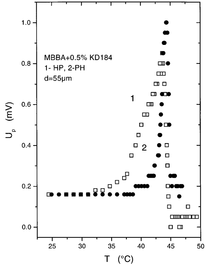
FIG. 4. Pyroelectric response vs temperature for hybrid (HP) cell irradiated from either the front (homeotropic and grounded) electrode (curve 1) or rear (planar) electrode (curve 2).
