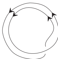
Fig.9. Doubly iterated torus knot
