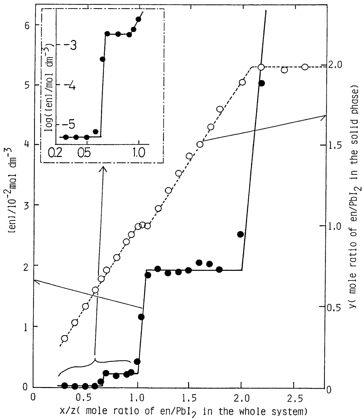
Fig. 5. A phase diagram for the \text{PbI}_2 -ethylenediamine(en)-ethanol system treated at 15^\circ\text{C} by the mole ratio method; z = 2.17 \text{ mmol} , V = 10 \text{ cm}^3 ; \bullet , concentration curve; \circ , composition curve. Low [\text{en}] 's are plotted in logarithm to express clearly changes of its concentration.
