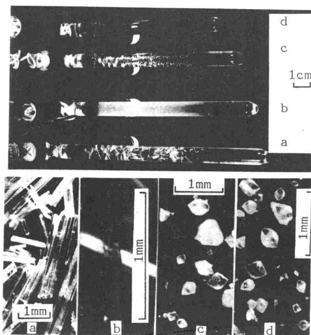
Fig. 21. Photographs of the single crystals grown by the transport method.
