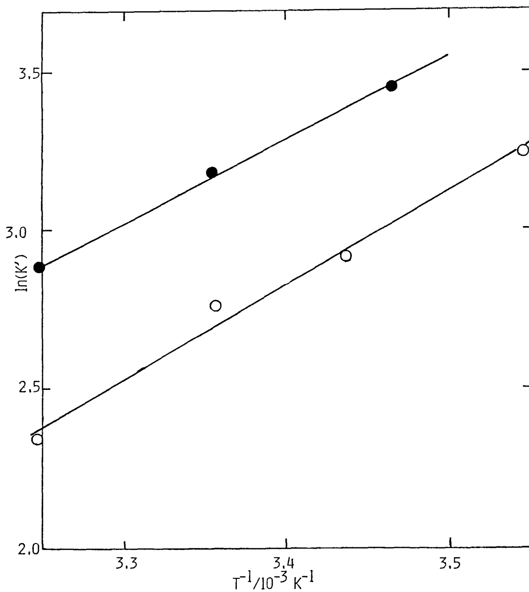
Fig. 14. Plot of logarithm of the stability constant versus 1/T :
