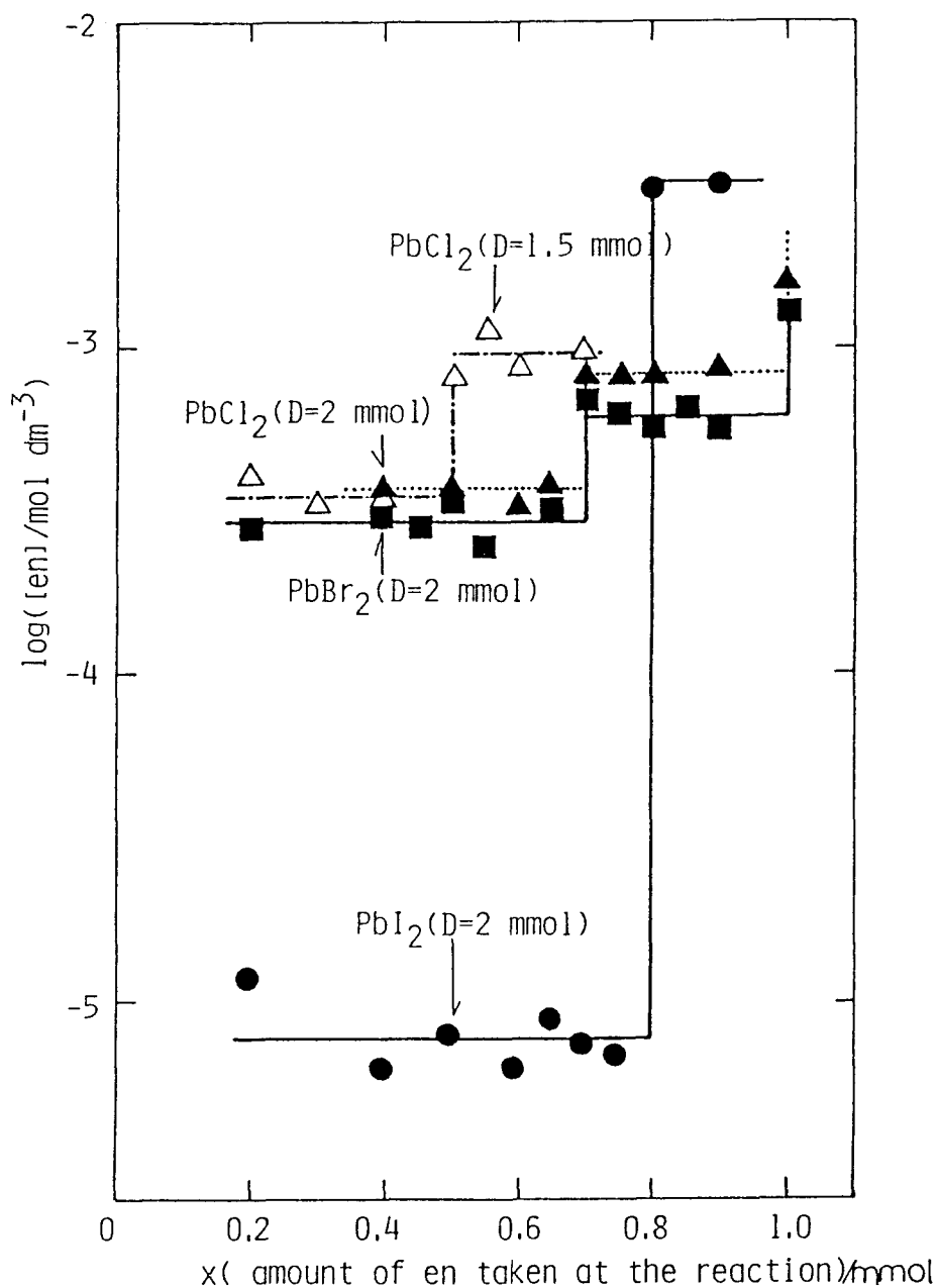
Fig. 12. A phase diagram for the ethylenediamine(en)- \text{PbX}_2 (X= Cl, Br, and I) - ethanol system treated at 25 °C by the continuous variation method; V=10 \text{ cm}^3 ; —●—, \text{PbI}_2 , D=2 mmol; —■—, \text{PbBr}_2 , D=2 mmol; —▲—, \text{PbCl}_2 , D=2 mmol; —△—, \text{PbCl}_2 , D= 1.5 mmol.
