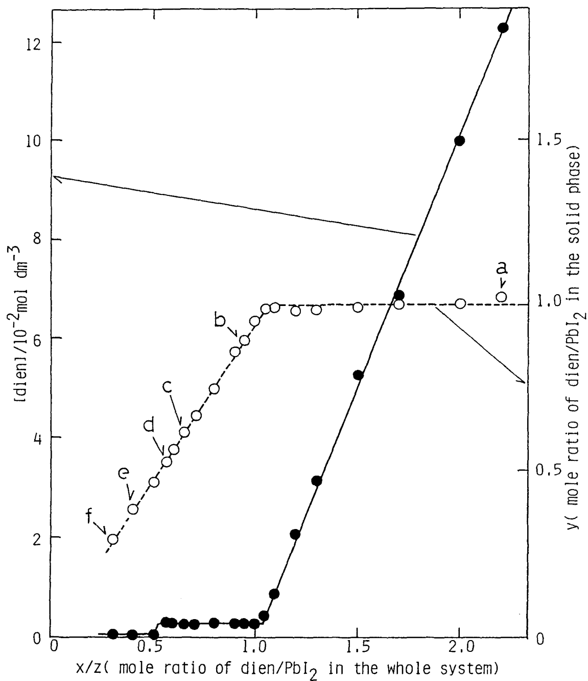
Fig. 6. A phase diagram for the \text{PbI}_2 - diethylenetriamine(dien)-ethanol system treated at 20 °C by the mole ratio method; z=1.08 \text{ mmol} , V=10 \text{ cm}^3 ; —●—, concentration curve; ---○---, composition curve.
