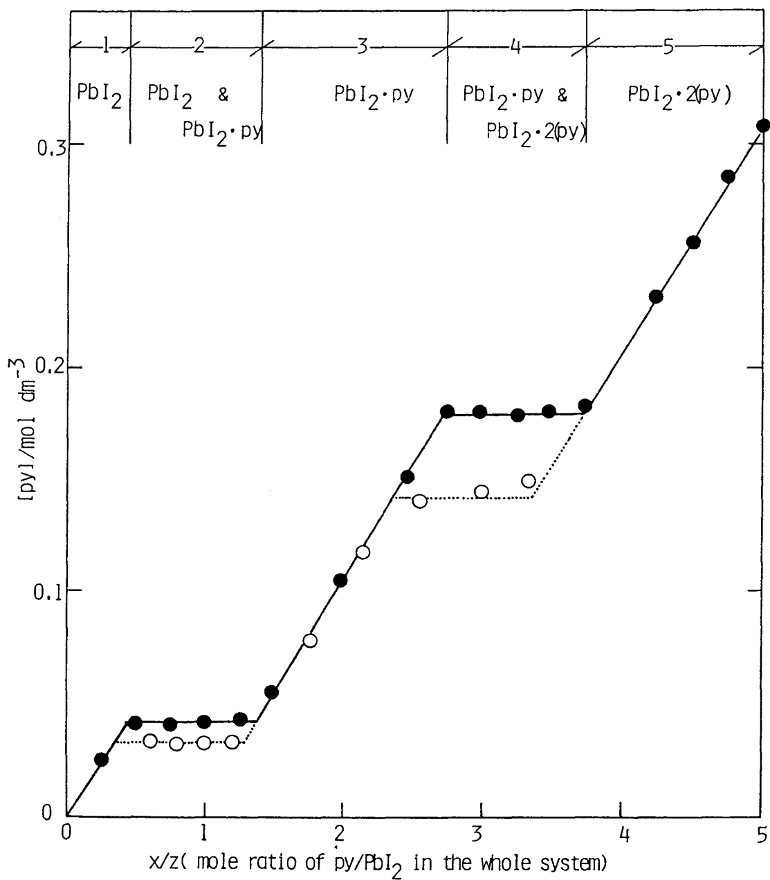
Fig. 17. A phase diagram for the \text{PbI}_2 -pyridine-ethanol system treated at 25 °C (●) and 15 °C (○) by the mole ratio method : z = 1.00 \text{ mmol} , V = 10 \text{ cm}^3 .
