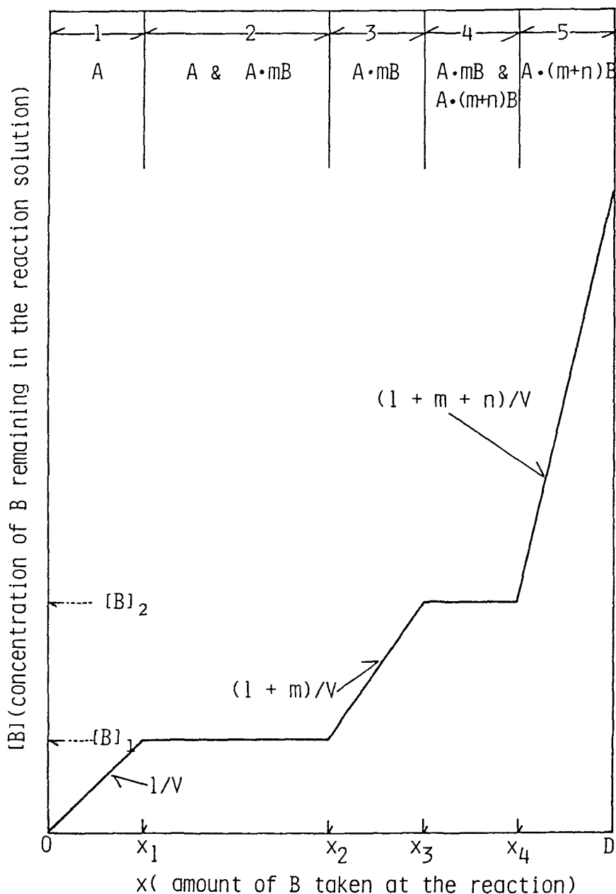
Fig. 8. A typical phase diagram for a ternary system when the continuous variation method is applied to a solid-liquid reaction, where two insoluble addition compounds, A \cdot mB and A \cdot (m+n)B , form. The values of the slope on the concentration curve equal 1/V , (1+m)/V , and (1+m+n)/V in the monovariant regions of 1, 3, and 5, respectively, where V is the volume of reaction solution.
