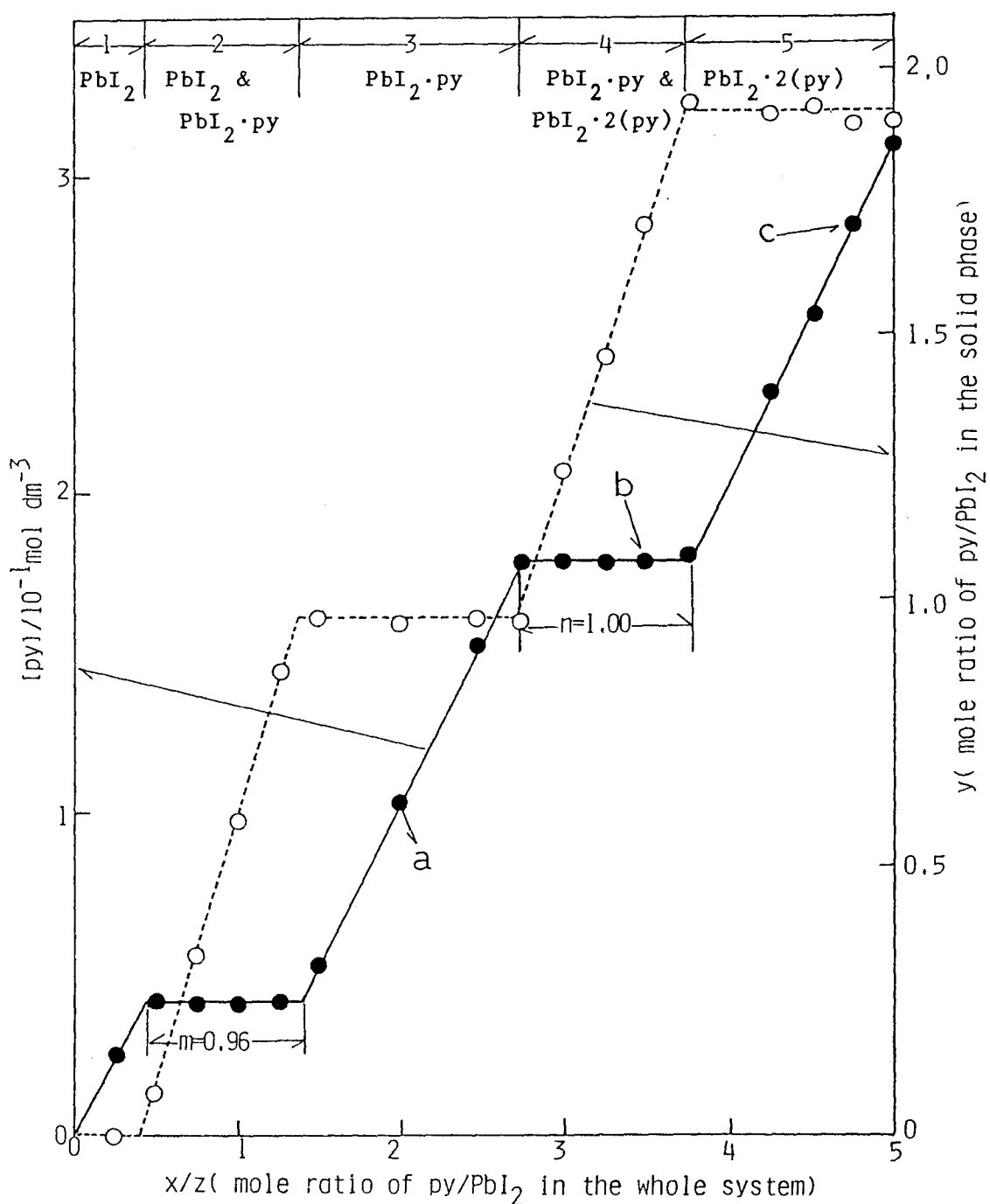
Fig. 2. A phase diagram for the \text{PbI}_2 -pyridine( py )-ethanol system treated at 25 °C by the mole ratio method: z = 1.00 mmol, V = 10 \text{ cm}^3 .
