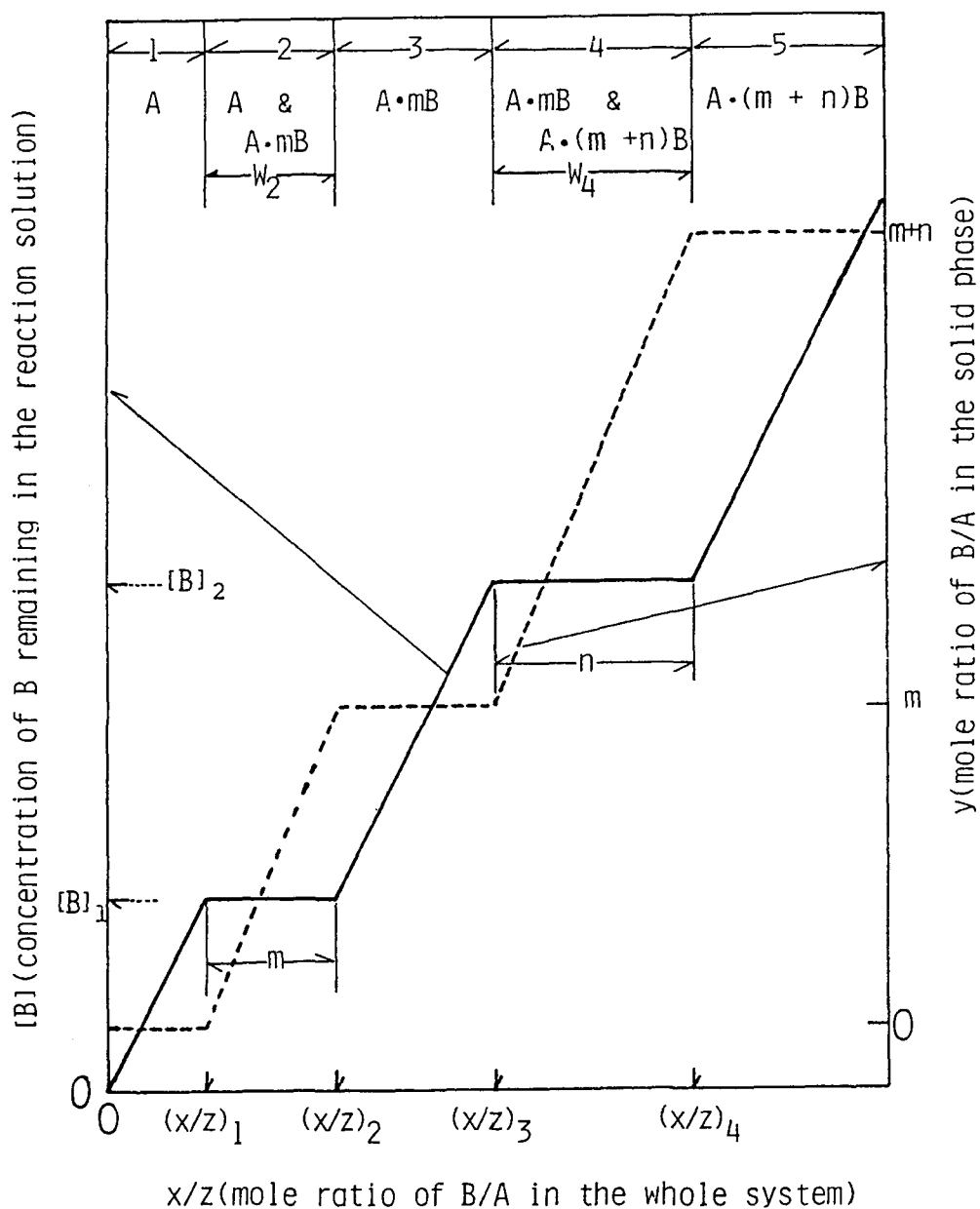
Fig. 1. A typical phase diagram for a ternary system when the mole ratio method is applied to a solid-liquid reaction, where two insoluble addition compounds, A \cdot mB and A \cdot (m+n)B , form:—, concentration curve;---, composition curve.
