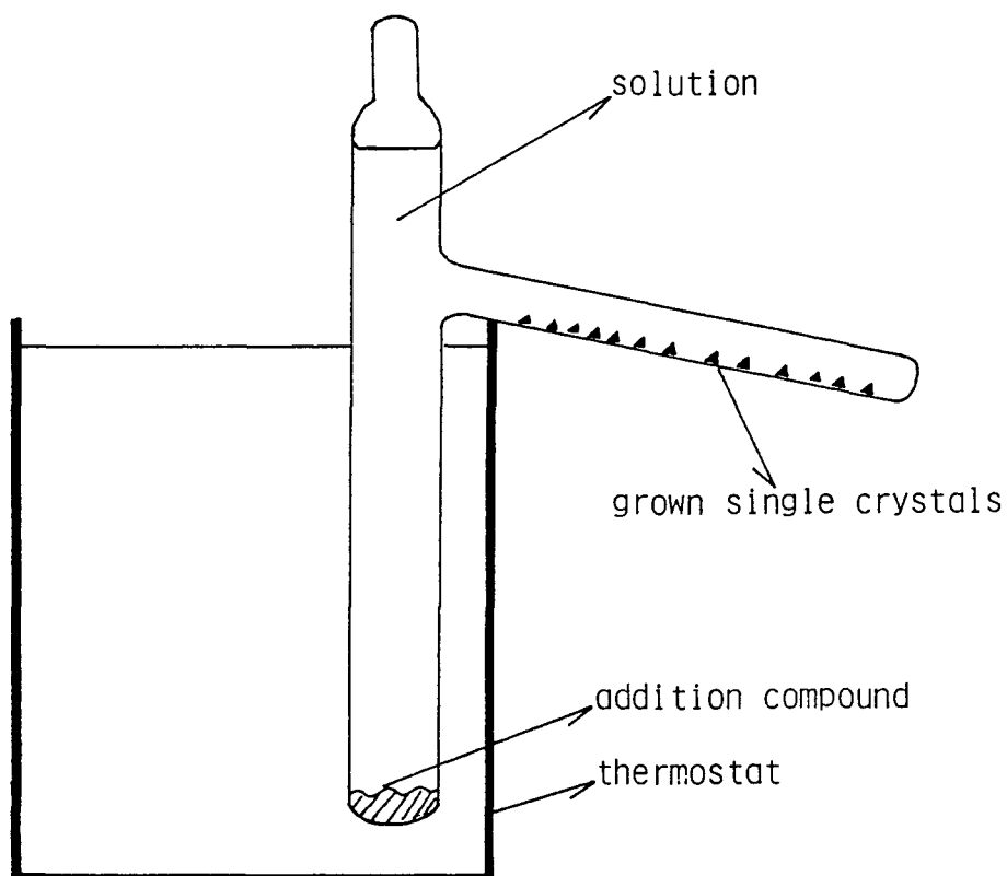
Fig. 22. A simple transport method for the single crystal growth of an insoluble addition compound: Temperature of a thermostat is kept higher than room temperature.
