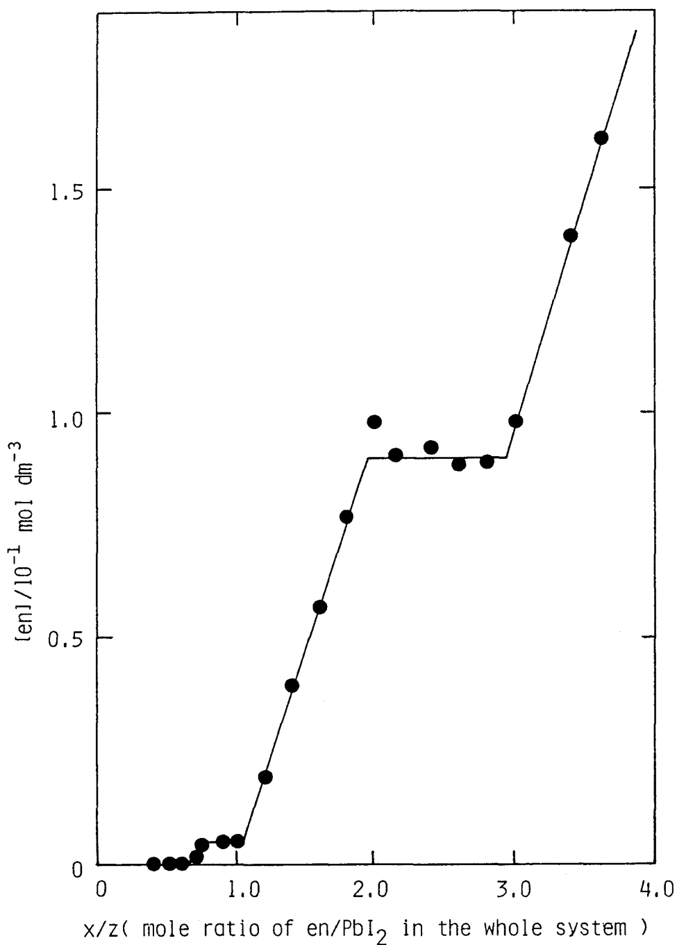
Fig. 23. A phase diagram for the \text{PbI}_2 - ethylenediamine(en) - methanol system treated at 25 °C by the mole ratio method z = 1.00 \text{ mmol} , V = 10 \text{ cm}^3 ; —●—, concentration curve.
