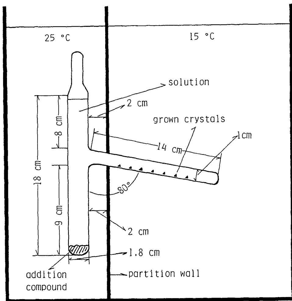
Fig. 18. A transport method for the single crystal growth of insoluble addition compounds.
