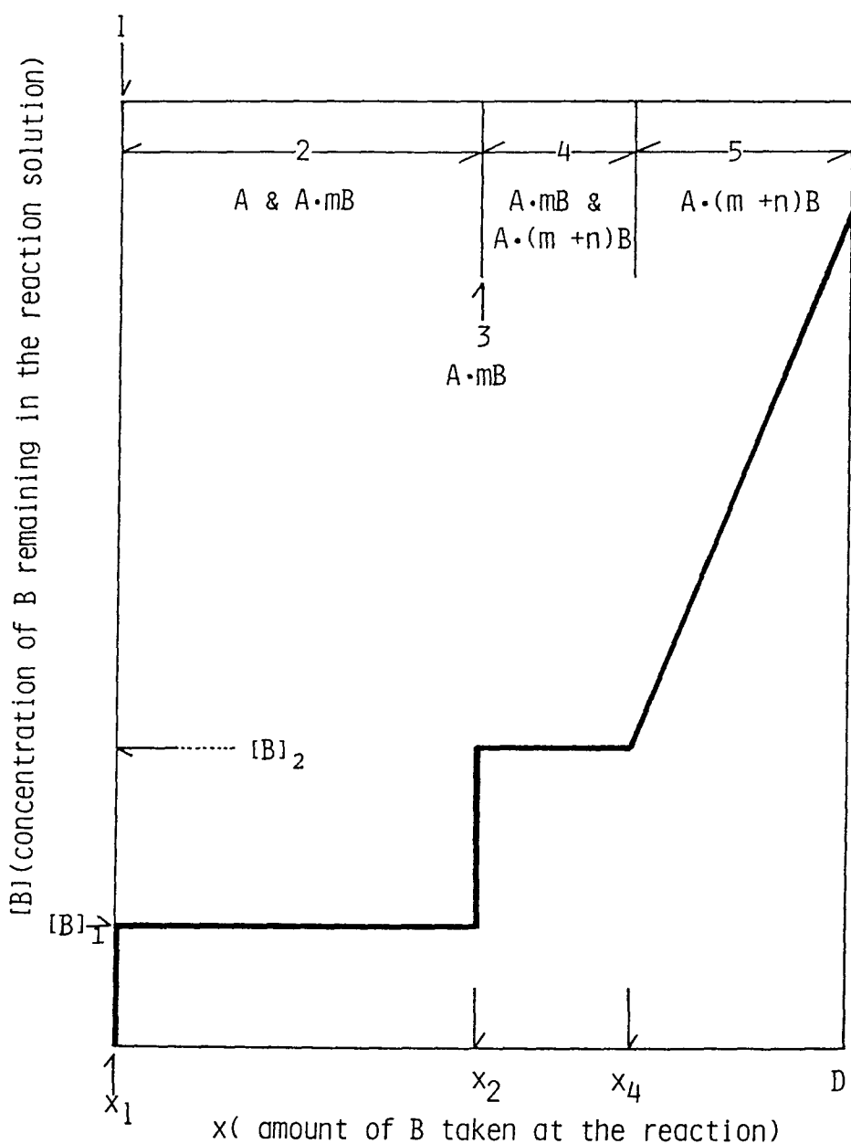
Fig. 9. A typical phase diagram for a ternary system where both [B]_1 and [B]_2 in the invariant regions are very low, when the continuous variation method is applied to a solid-liquid reaction. Since the widths of two monovariant regions 1 and 3 are narrow, the concentration curve ascends sharply at x_1 and x_2 .
