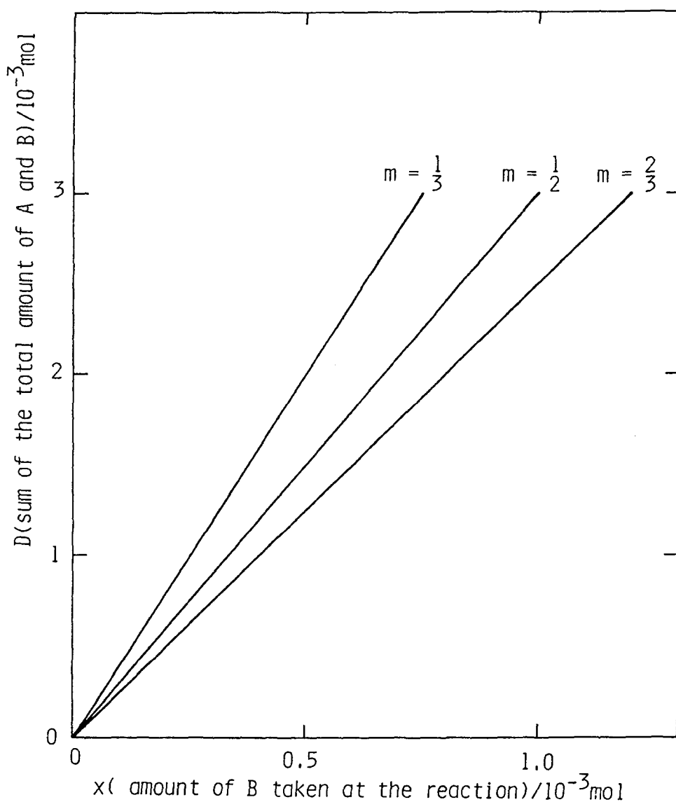
Fig. 10. Relation between the point of phase boundary and the sum(D) of A and B by application of the continuous variation method to a solid-liquid reaction where both [B]_1 and [B]_2 in the invariant regions are very low: m is the composition of the addition compound.
