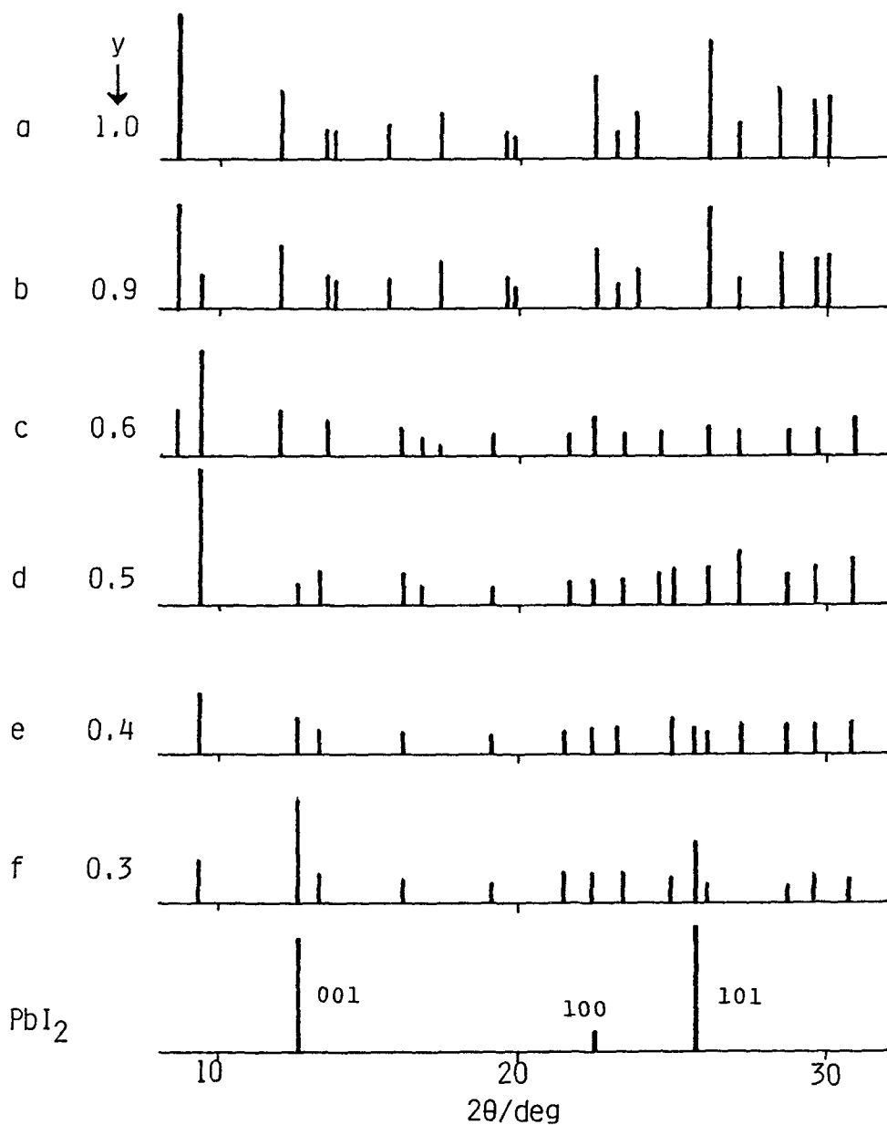
Fig. 7. The powder X-ray diffraction patterns of \text{PbI}_2 \cdot y(\text{dien}) and \text{PbI}_2 where y represents the mole ratio of \text{dien}/\text{PbI}_2 determined by the chemical analysis. The marks, a - f, designate in Fig. 6. The peaks of \text{PbI}_2 are indexed. 15)
