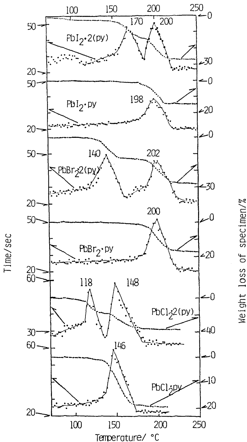
Fig. 15. Thermal behavior of \text{PbX}_2 \cdot y(\text{pyridine}) ( X = \text{Cl}, \text{Br}, \text{and I} ; y = 1 \text{ and } 2 ) measured with a Shinkuriko TGCC-1500RH calorimetric thermobalance: specimen, 1 g; bias voltage, 150 \mu\text{V} ; \text{N}_2 gas flow rate, 55 ml/min .
