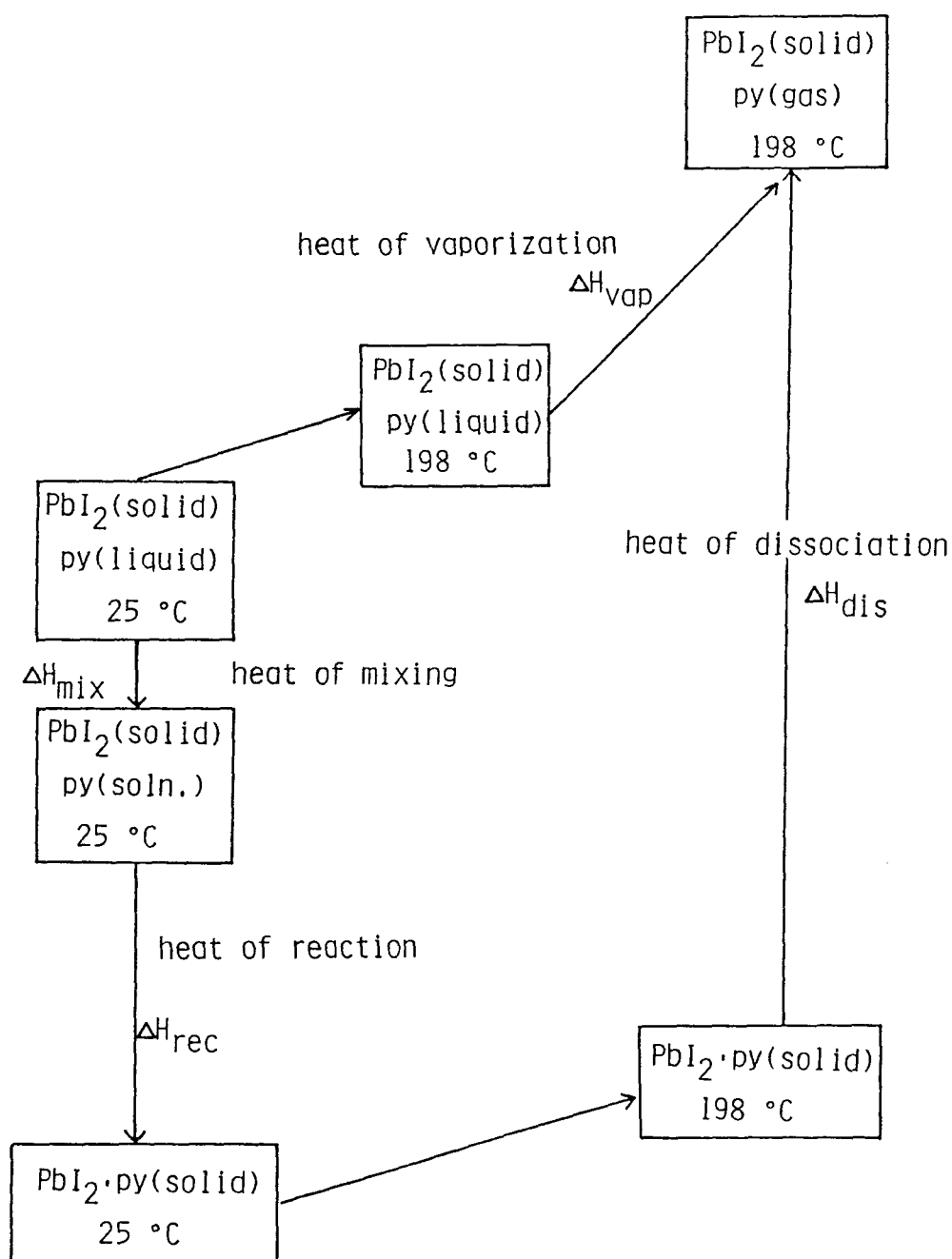
Fig. 16. The enthalpy cycle of \text{PbI}_2 \cdot \text{py} . Dissociation temperature of \text{PbI}_2 \cdot \text{py} is 198^\circ\text{C} . \Delta H_{\text{rec}} is the heat of reaction of \text{PbI}_2 \cdot \text{py} , \Delta H_{\text{vap}} , the heat of vaporization of pyridine, \Delta H_{\text{dis}} , the heat of dissociation of \text{PbI}_2 \cdot \text{py} , and \Delta H_{\text{mix}} , the heat of mixing of pyridine with ethanol.
