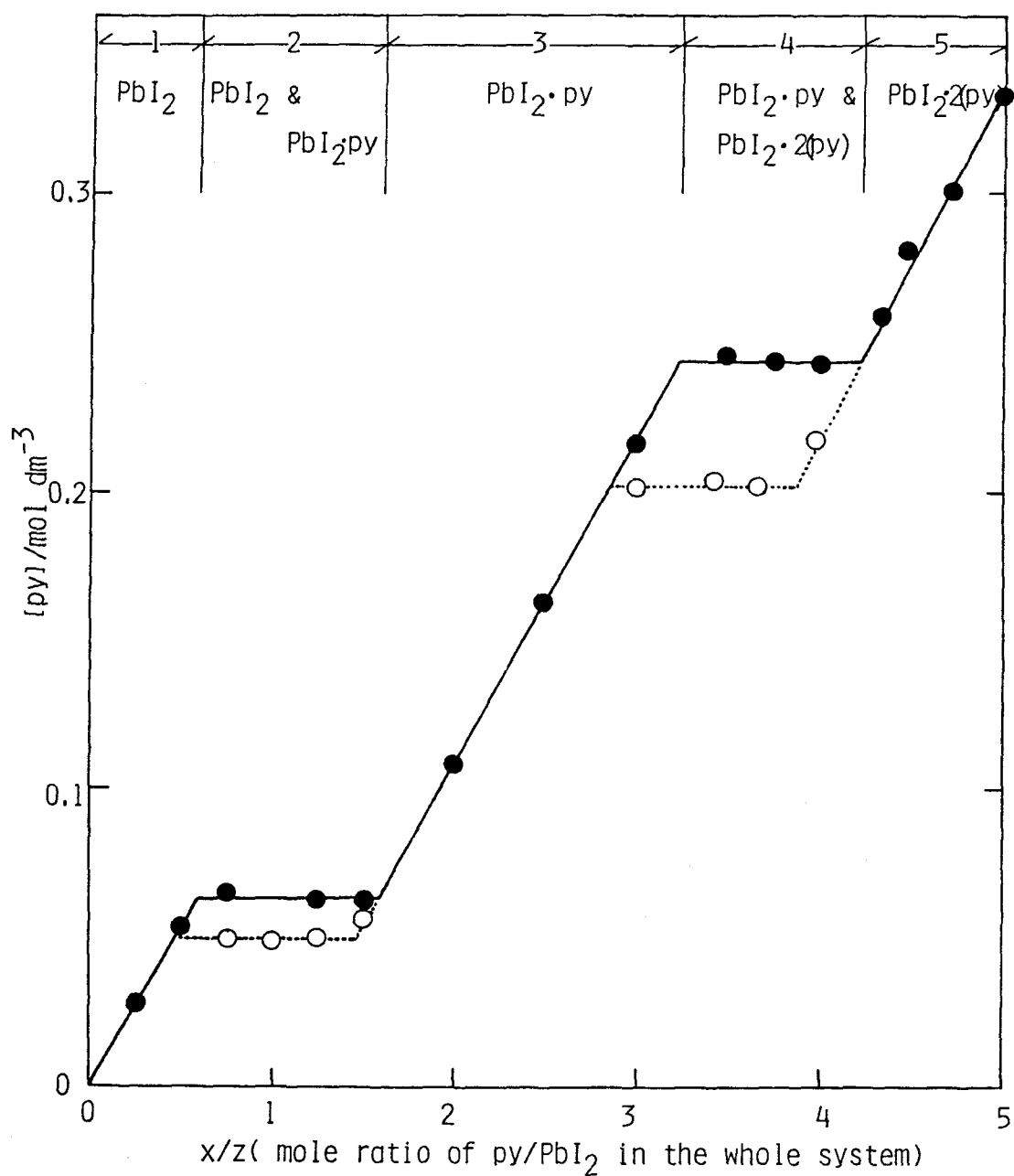
Fig. 20. A phase diagram for the \text{PbI}_2 - pyridine - methanol system treated at 25^\circ\text{C} (●) and 15^\circ\text{C} (○) by the mole ratio method : z = 1.08 \text{ mmol} , V = 10 \text{ cm}^3 .
