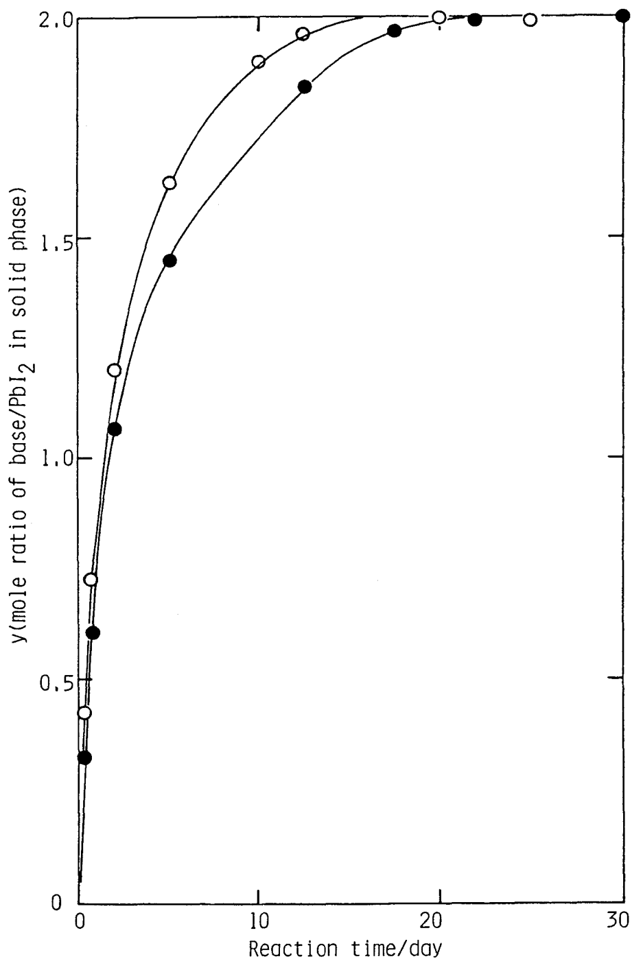
Fig. 3. Plot of the composition ( y ) of addition compounds formed in the solid phase versus reaction time for the \text{PbI}_2 - pyridine - ethanol and \text{PbI}_2 - ethylenediamine - ethanol systems: \bullet , pyridine ; \circ , ethylenediamine
