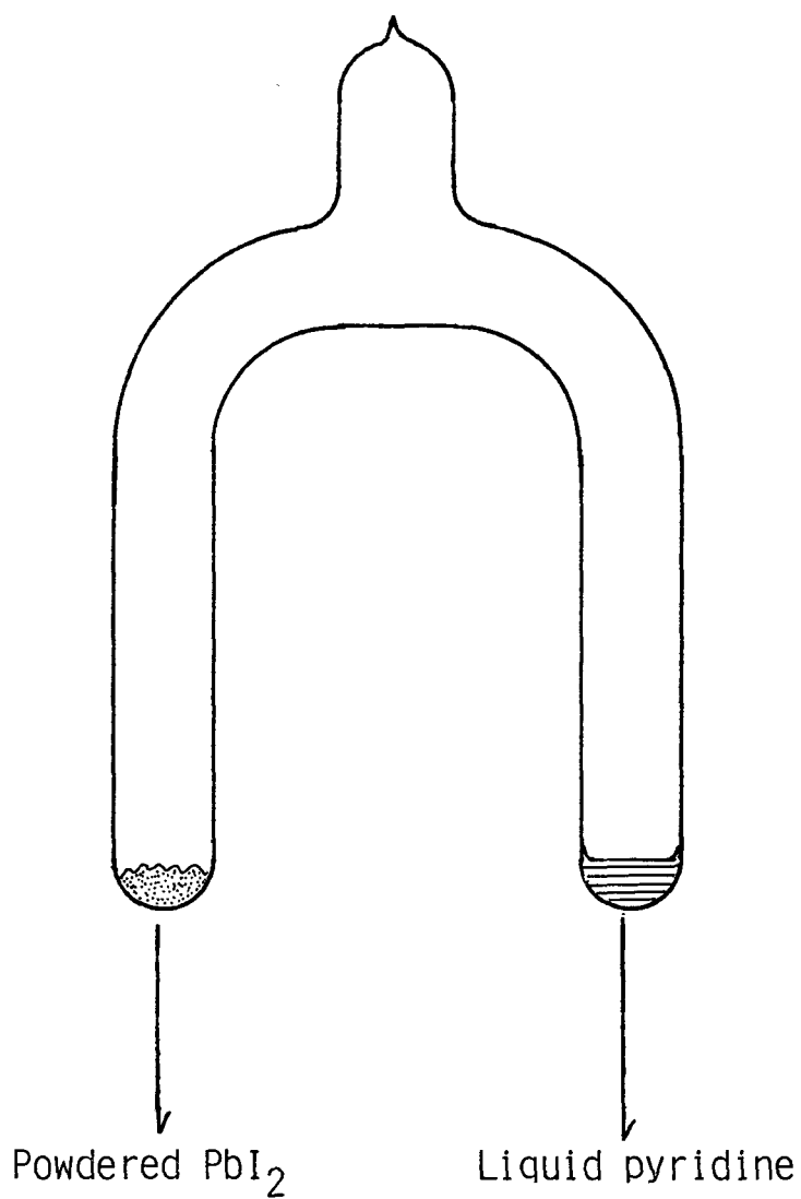
Fig. 4. A U-tube for the gas-solid reaction of \text{PbI}_2 with vapor pyridine.
