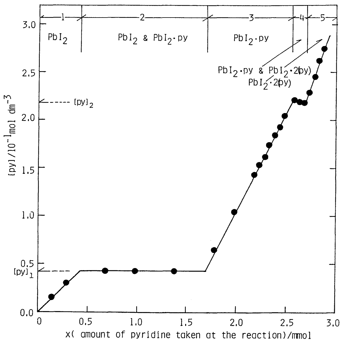
Fig. 11. A phase diagram for the \text{PbI}_2 - pyridine(py) - ethanol system treated at 25 °C by the continuous variation method; D=3.0 \text{ mmol} , V=10 \text{ cm}^3 .
