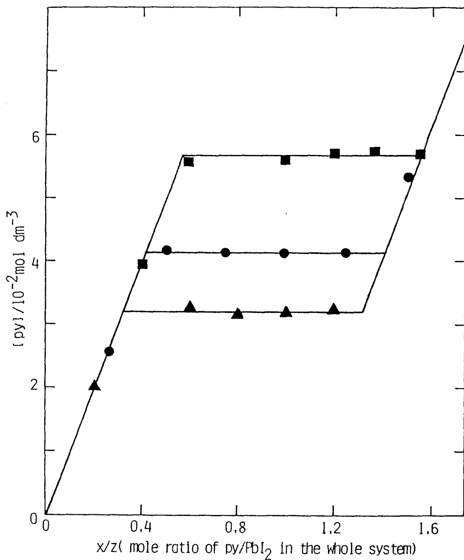
Fig. 13. Temperature dependence of the concentration of pyridine at the invariant region of the PbI_2 - pyridine - ethanol system by the mole ratio method: z = 1.00 \text{ mmol} , V = 10 \text{ cm}^3 . —■— , 34.8 °C ; —●— , 25.0 °C ; —▲— , 15.4 °C.
