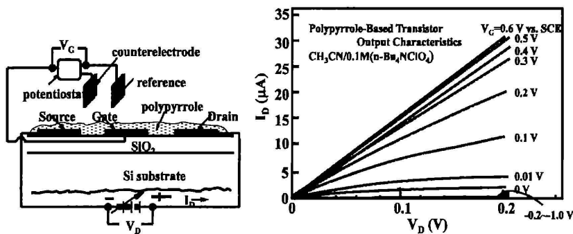
H.S.White, G.P.Kittlesen, and M.S.Wrighton, "Chemical derivatization of an array of three gold microelectrodes with polypyrrole: Fabrication of a molecular-based transistor", Journal of American Chemical Society , 106 (1984) p.5375-5377.
