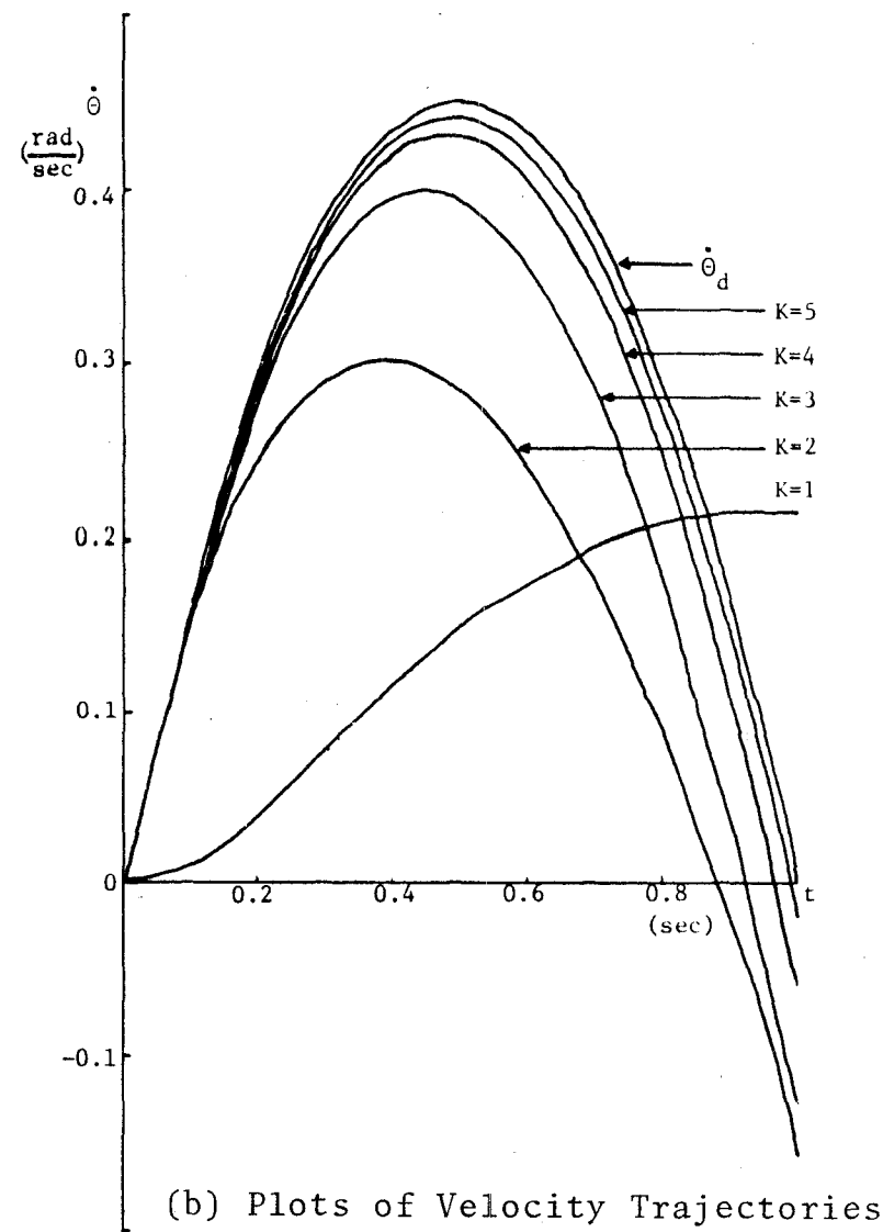
Fig.9-14 Simulation Result in Joint-angle Coordinates The gain matrix \Lambda = R(\theta_k(t))
