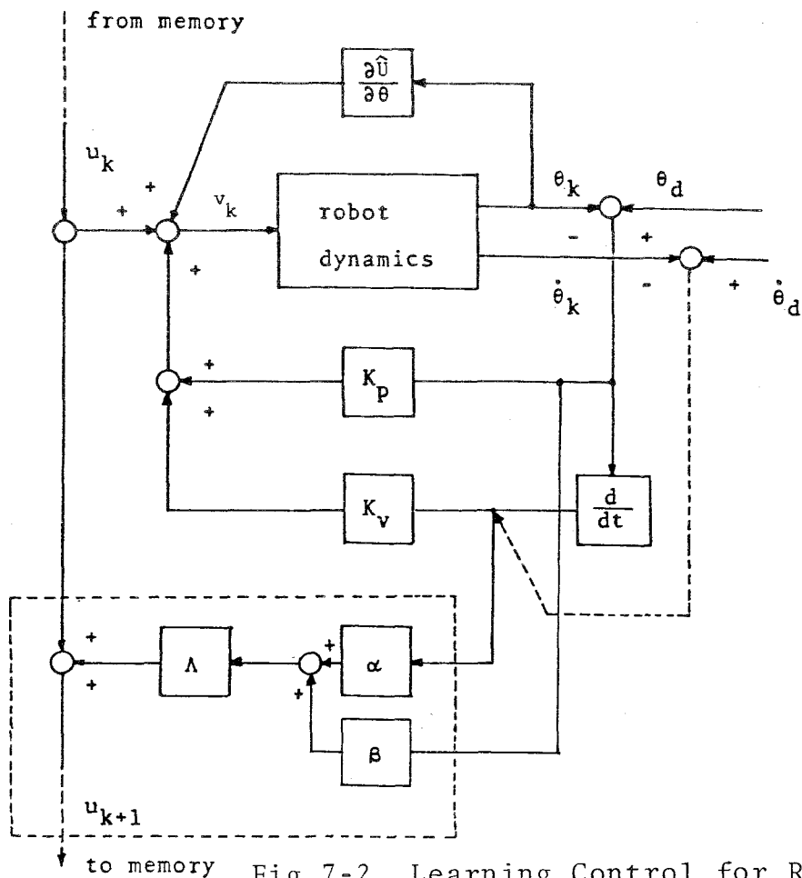
Fig.7-2 Learning Control for Robot Dynamics Based on the Velocity Signals
