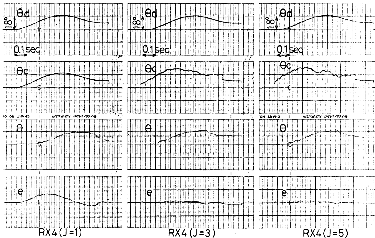
Fig.9-3 Experimental Result of the Biped Locomotion Robot
