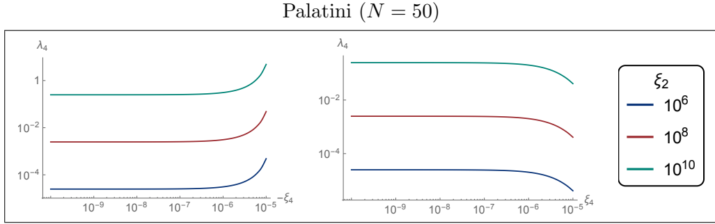
Figure 4: The same as in Fig. 2 except for N = 50 .
