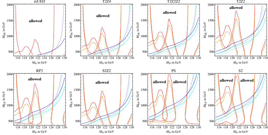
Figure 1: 95% CL bounds from H \rightarrow \gamma\gamma at ATLAS (red/orange dashed) and at CMS (red/orange solid) and from H \rightarrow WW \rightarrow \nu l \nu l at CMS with cut-based (blue/cyan solid) and with multi-variate BDT (dotted) event selections. The red and blue (orange and cyan) colors correspond to the maximum (minimum) UV cutoff scale in 6D.
