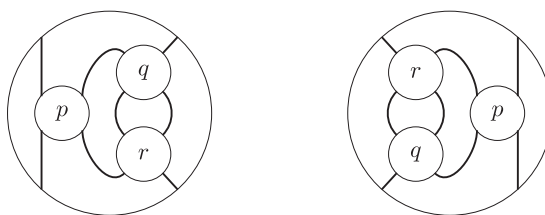
Fig.10. Equivalent tangles
