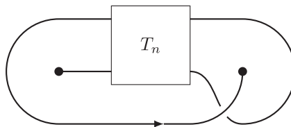
Fig.5. The diagram D_n
