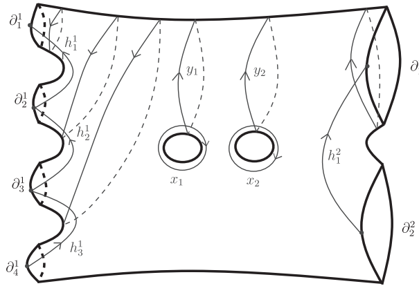
Fig. 1. An example illustrating homology basis elements of H_1^P(\Sigma_{2,6}; \mathbb{Z}) , where \mathcal{P} = \{\{\partial_1^1, \partial_2^1, \partial_3^1, \partial_4^1\}, \{\partial_1^2, \partial_2^2\}\} .
