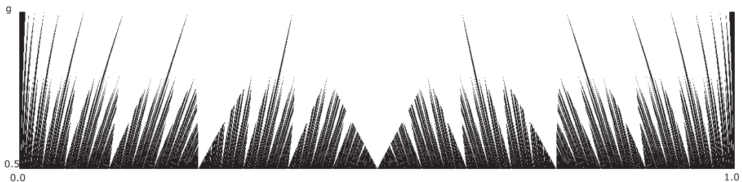
Fig. 1. J_1(S(a)) for a between 1/2 and the golden ratio g
