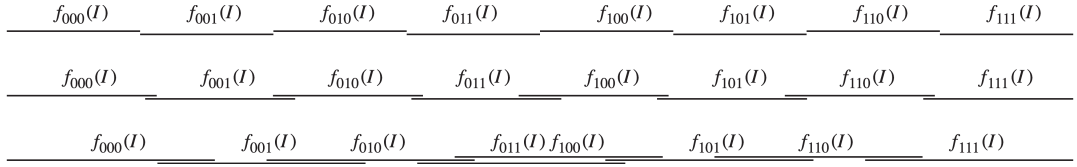
Fig. 2. The intervals f_\omega(I) for \omega \in \{0,1\}^3 when a = 0.5 (top), a = 0.52 (middle), and a = 0.58 (bottom).
