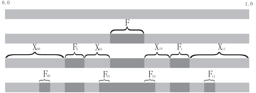
Fig.4. The structure of S_1(a) .
