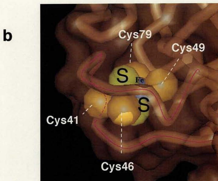
Spirulina ferredoxin
