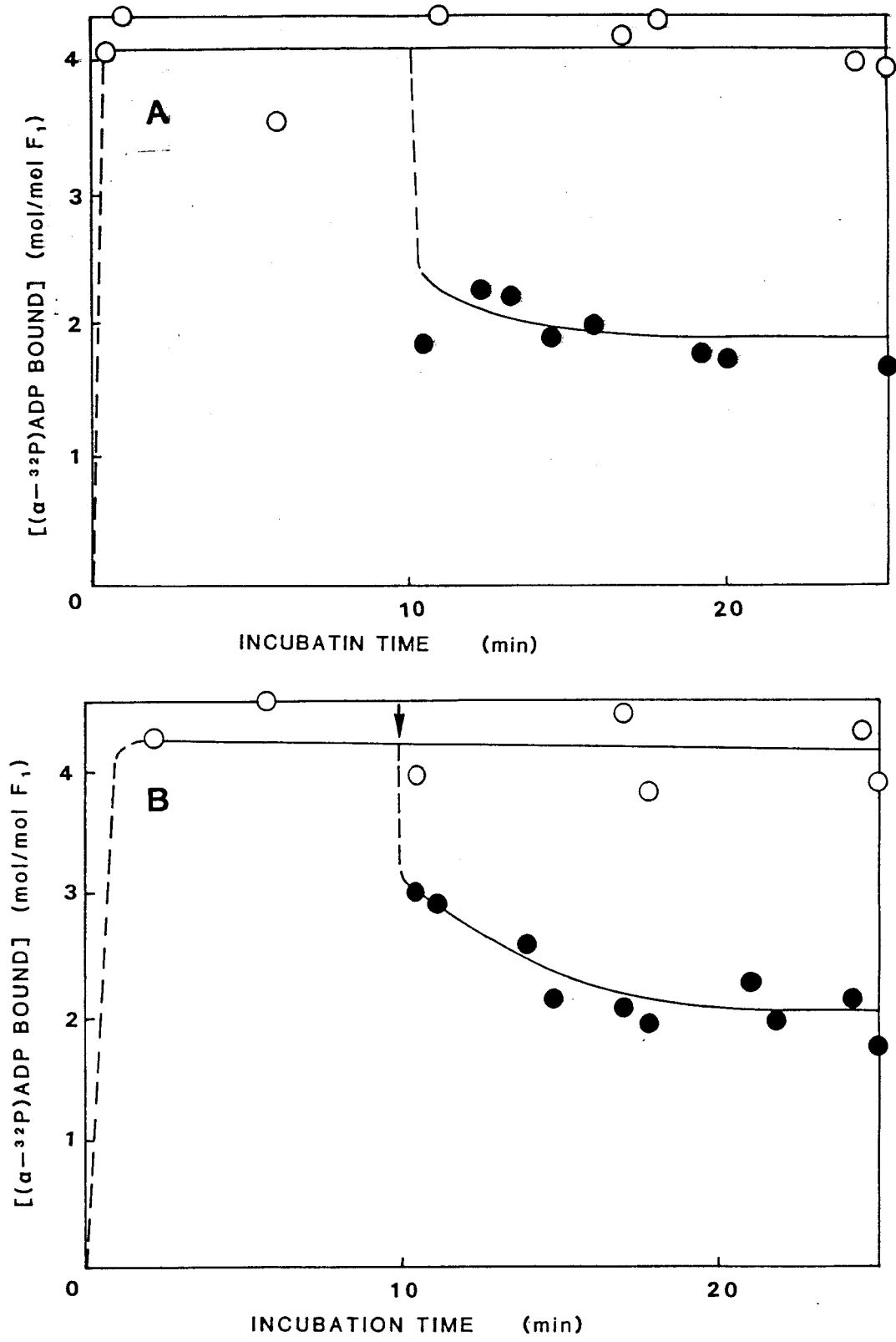
Fig. 2. Time courses of binding of ADP to F 1 in the presence and absence of DMSO. A: F 1 at 8.5 μM was incubated with 80 μM [\alpha-^{32}\text{P}]\text{ADP} in the standard DMSO-buffer solution at 30°C and the amount of bound [\alpha-^{32}\text{P}]\text{ADP} (○) was measured. The closed circles show the amount of [\alpha-^{32}\text{P}]\text{ADP} remaining on F 1 after addition of nonradioactive ADP at the final concentration of 2 mM. B: F 1 was incubated with [\alpha-^{32}\text{P}]\text{ADP} at 18°C in the same solution as for A except that DMSO was omitted but 150 mM sucrose was added. The reaction was chased by 1 mM of nonradioactive ADP.
