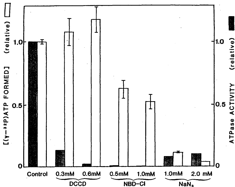
Fig. 6. Effects of inhibitors on the F_1 -ATPase activity and the ATP synthesis by F_1 . F_1 (2.1 mg/ml) was preincubated with DCCD, NBD-Cl or sodium azide in the presence of 33 \mu\text{M} ADP (no ADP in the case of sodium azide), 0.9 \text{ mM} EDTA, 35% (w/v) DMSO, 12% (w/v) glycerol, and 0.1 \text{ M} MES-Tris at pH 6.7 and 30^\circ\text{C} for 80 min. The concentration of each inhibitor used for the pretreatment is given on the abscissa. The preincubation mixture was mixed with 1/9 volume of a solution containing 0.3 \text{ mM} ADP, 2 \text{ mM} ^{32}\text{P}_i , 35% (w/v) DMSO, and 0.1 \text{ M} MES-Tris at pH 6.7, and the amount of [\gamma\text{-}^{32}\text{P}]\text{ATP} formed was measured 30 min after the start of the reaction. The ATPase activity was measured as described in EXPERIMENTAL PROCEDURES. Values are expressed relative to those of the control, where F_1 was preincubated with no inhibitors. The control value of ATPase activity was 68 \text{ unit/mg} and that of the amount of ATP formed was 0.036 \text{ mol/mol } F_1 .
