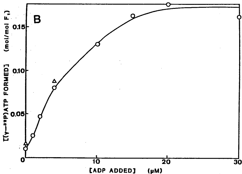
Fig. 11. Dependence on concentration of added ADP of the amount of ATP formed by F_1 . A: F_1 at 1.9 mg/ml was allowed to react with 10 mM P_i and various concentrations of [\alpha\text{-}^{32}\text{P}]\text{ADP} in the standard DMSO-buffer solution at 30°C for 30 min. The inset shows a double reciprocal plot of the amount of formed ATP against the concentration of free ADP calculated as described in the text. B: F_1 at 0.82 mg/ml was allowed to react with 0.2 mM ^{32}\text{P}_i and various concentrations of ADP in the standard DMSO-buffer solution at 30°C for 60 ( \circ ) or 100 min ( \Delta ).
